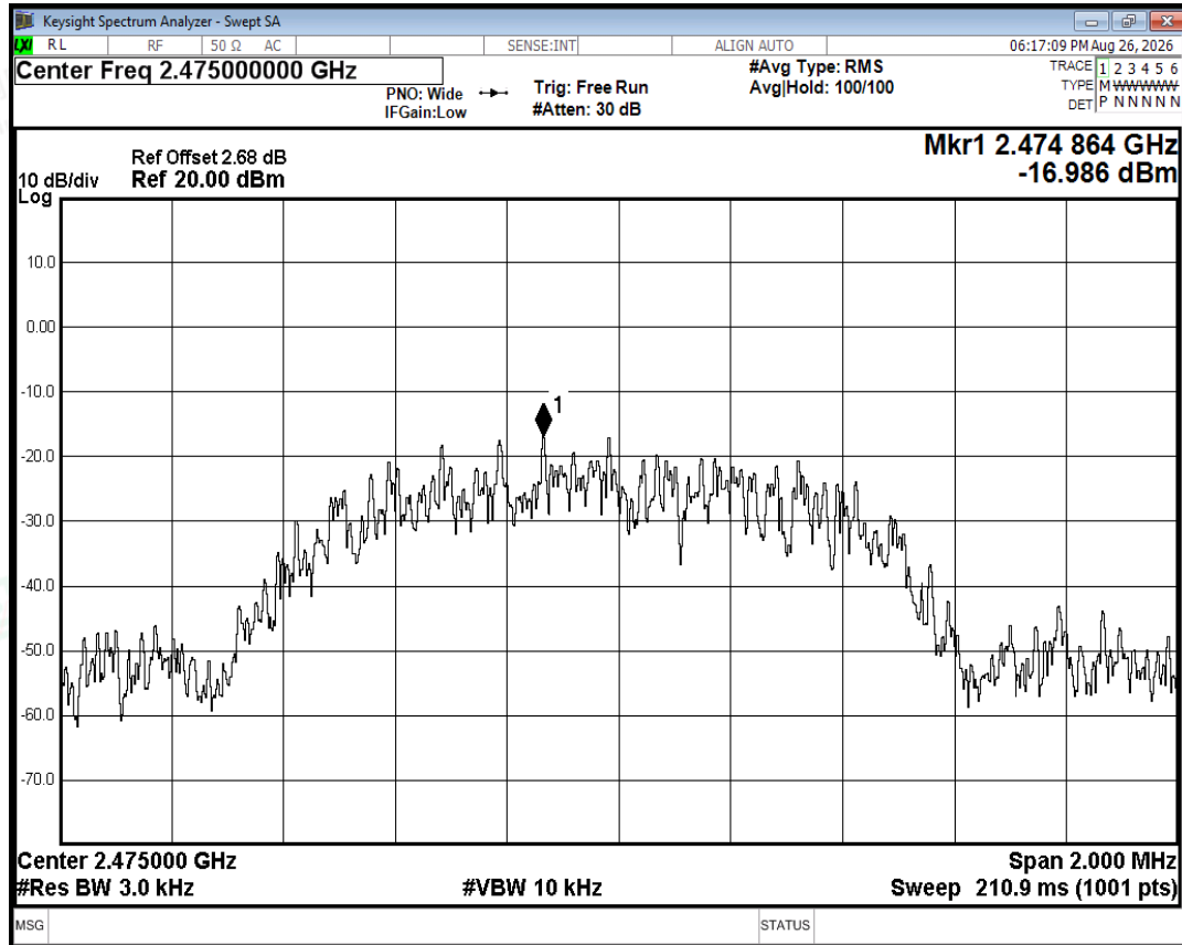
PSD NVNT 2.4G 2475MHz Ant1
