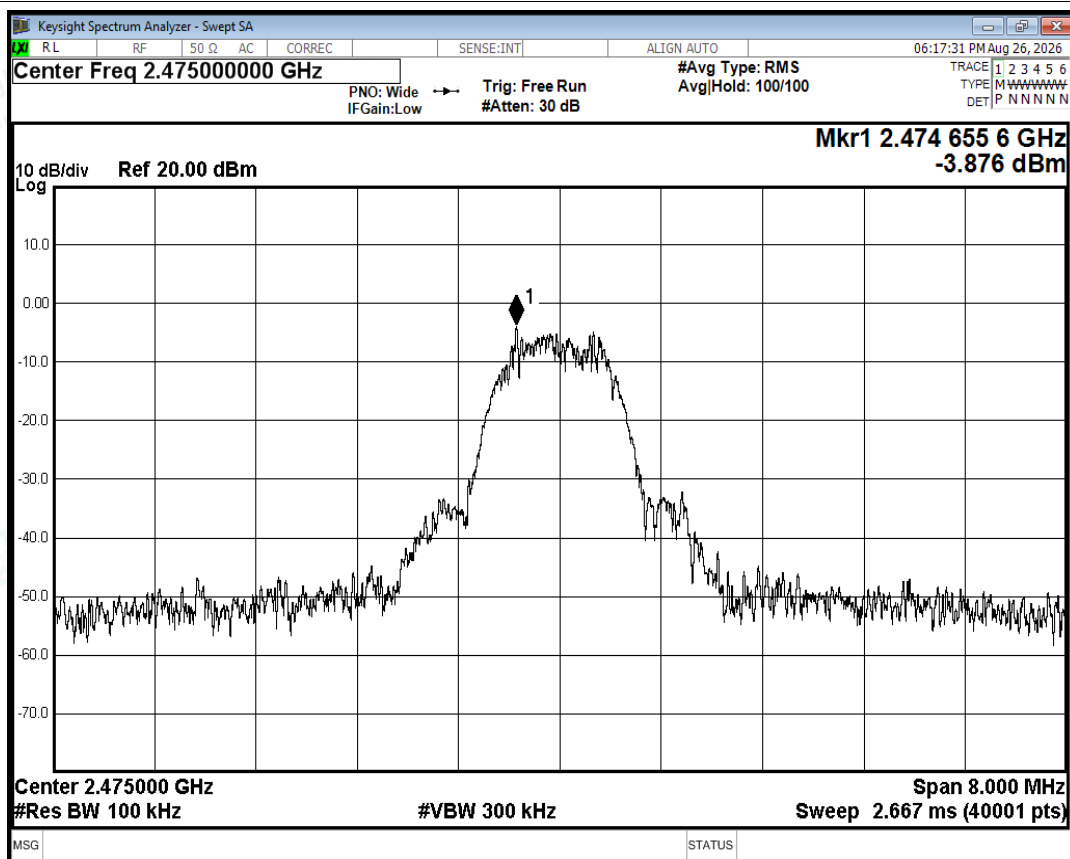
Tx. Spurious NVNT 2.4G 2475MHz Ant1 Ref
