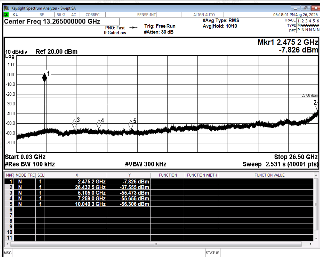
Tx. Spurious NVNT 2.4G 2475MHz Ant1 Emission
