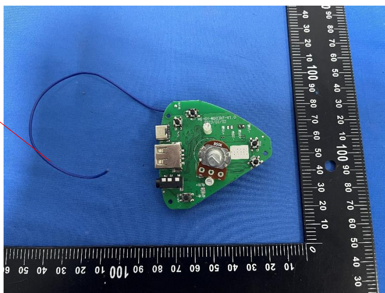
FM RX ANT
