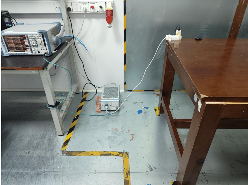
Conducted Emissions at Mains Terminals (150 kHz-30MHz)
