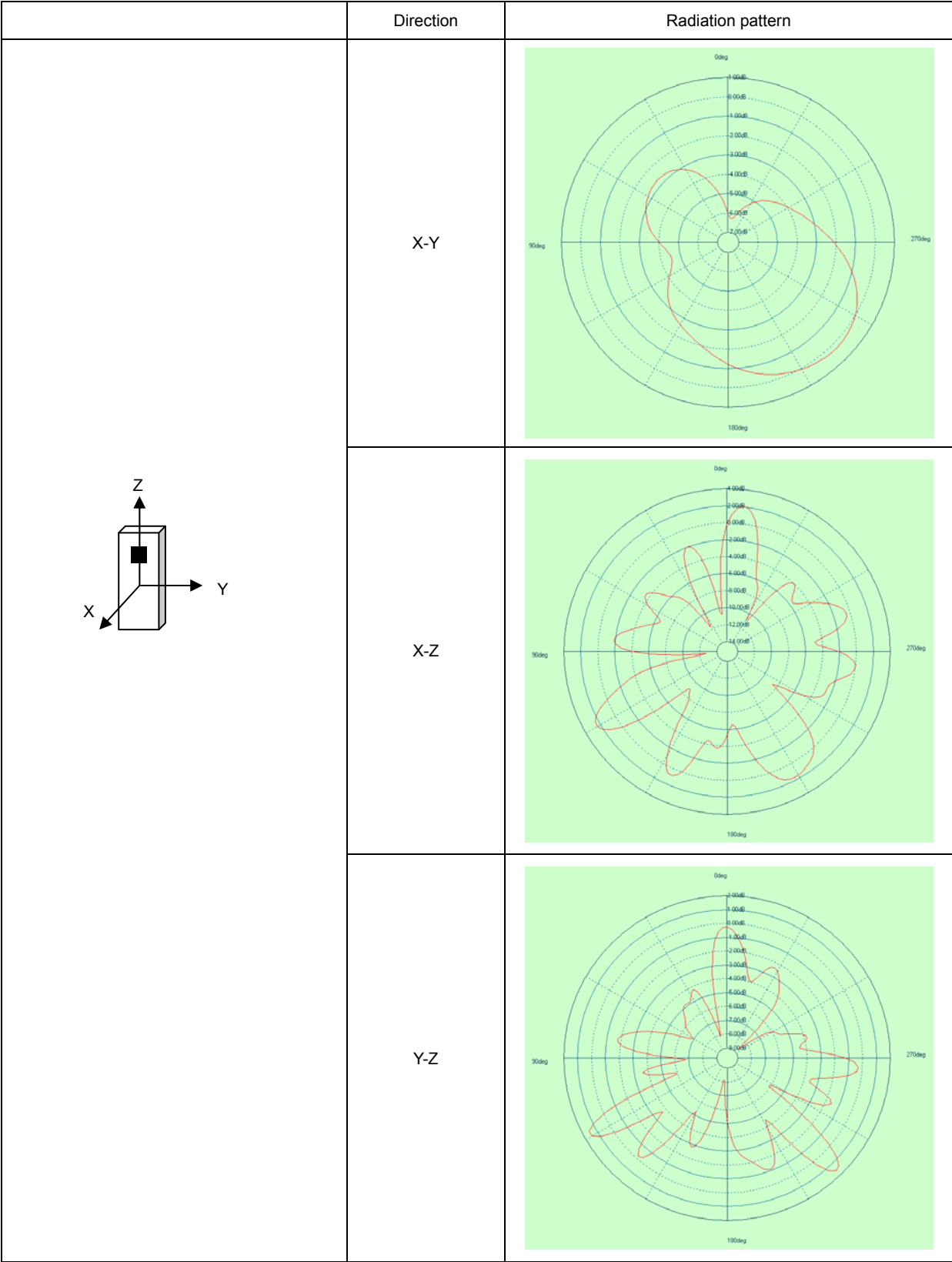
Radiation pattern:
