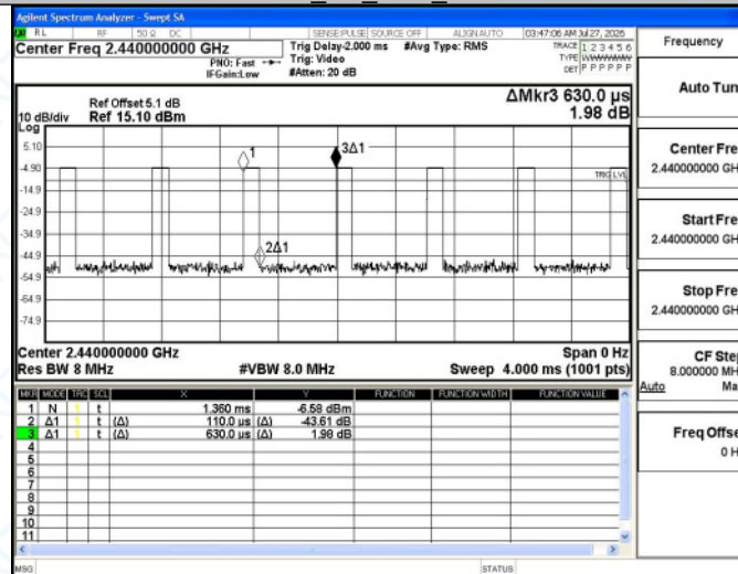
BLE_1M_Ant1_2440
