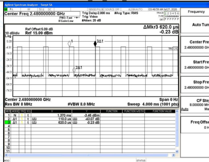
BLE_1M_Ant1_2480
