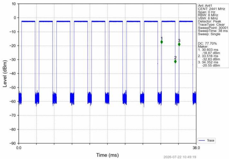
GFSK_DH5_MCH_2441MHz_ANT_NTNV
