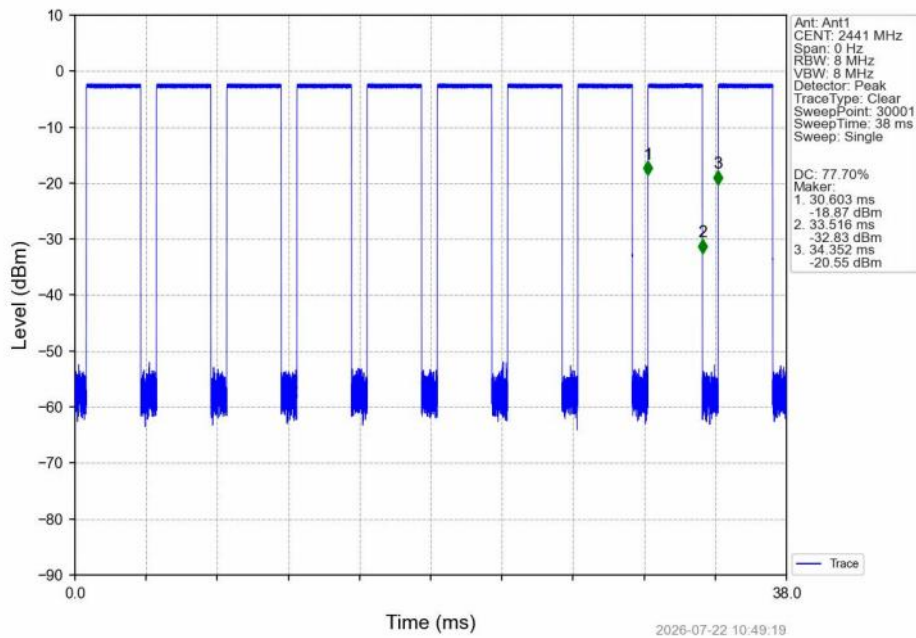
GFSK_DH5_MCH_2441MHz_ANT_NTNV
