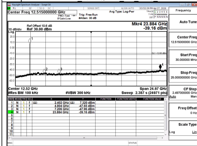
Spurious Emission 8DPSK 3M DH5 2402MHz
