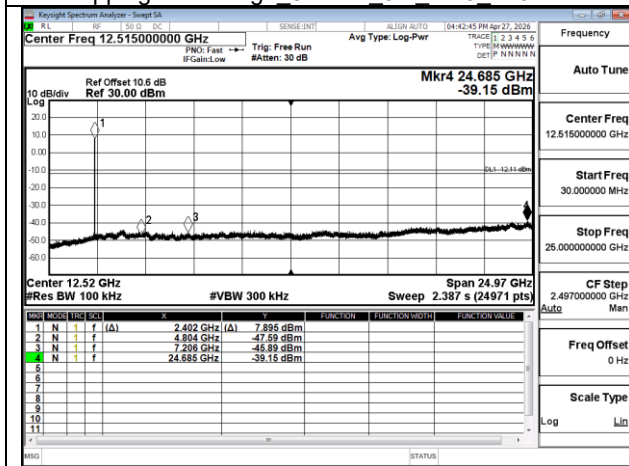
Spurious Emission GFSK 1M DH5 2402MHz
