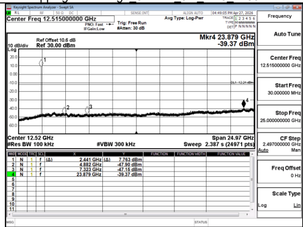
Spurious Emission GFSK 1M DH5 2441MHz
