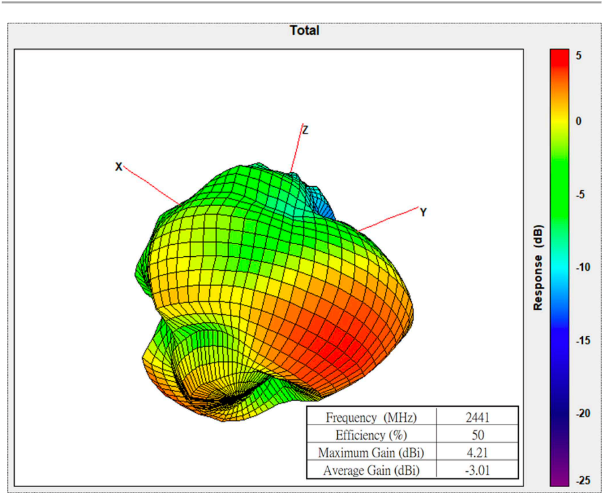
Figure 6-1 ATM2-MOD-A PCB Antenna Radiation Pattern and Characteristics
