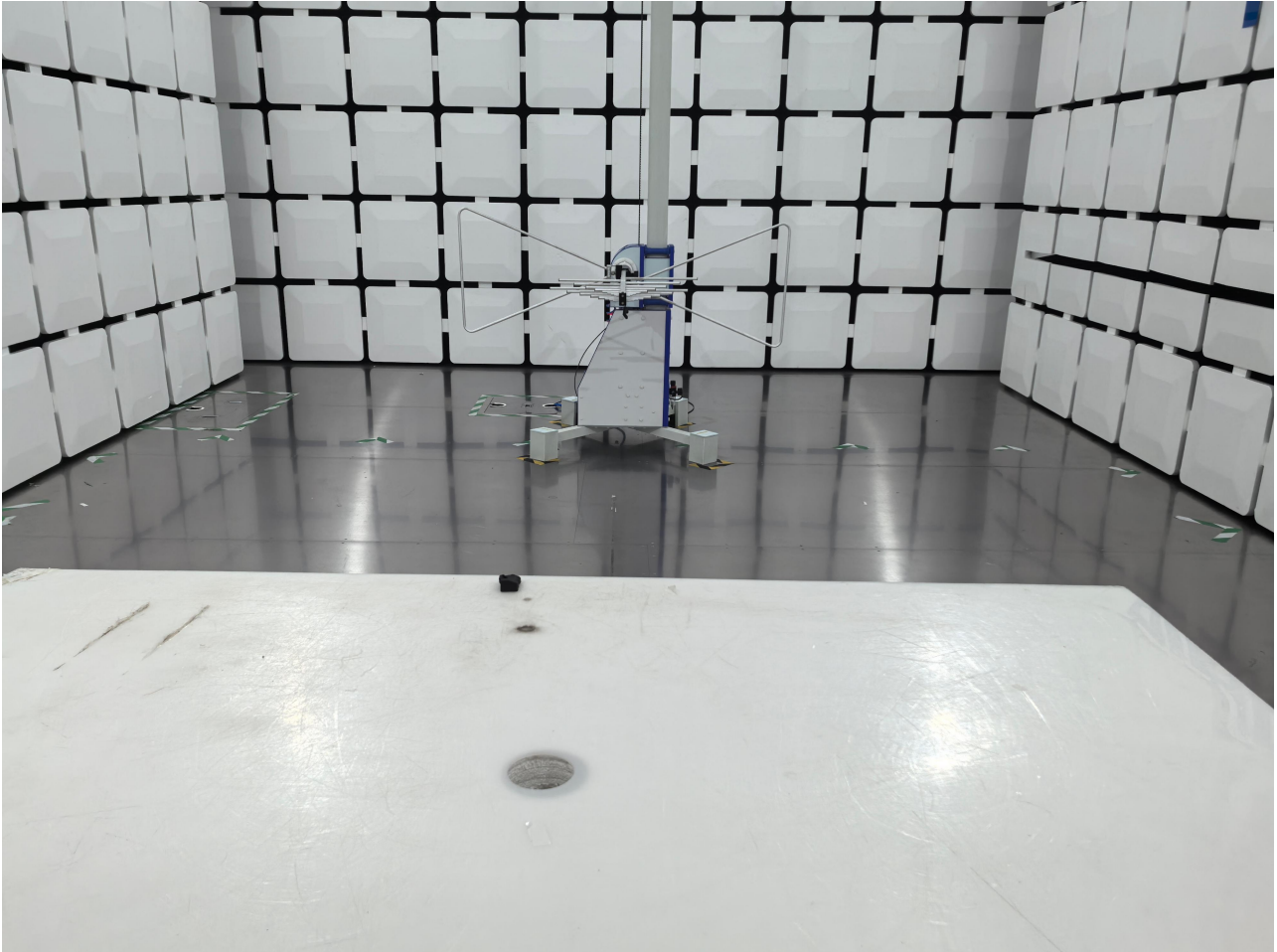
Radiated Spurious Emission Test View 1
