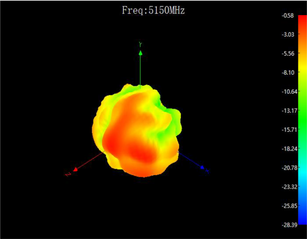
Antenna gain diagram
