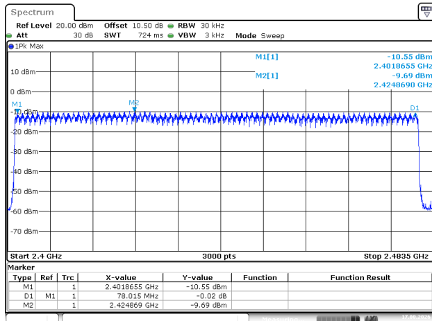
3DH1_Hopping
