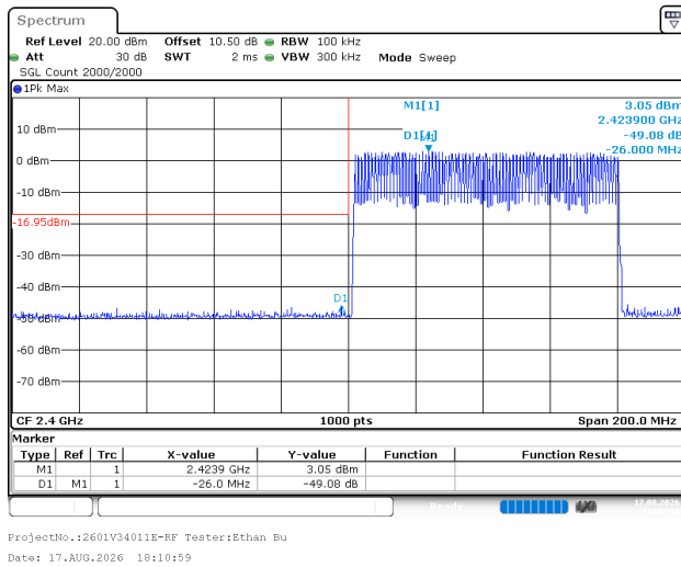
2DH1_Low
