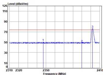
BLE_1M_TX_CH_00_Vertical-Peak
