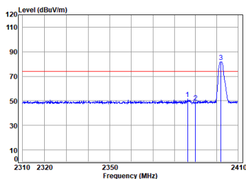
BLE_1M_TX_CH_00_Horizontal-Peak
