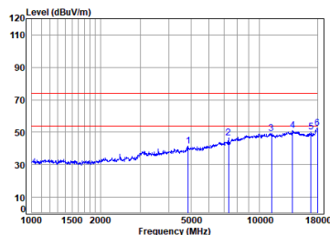
BLE_1M_TX_CH_19_Vertical
