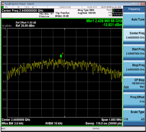
LE_1M-Ant1-2440-PASS
