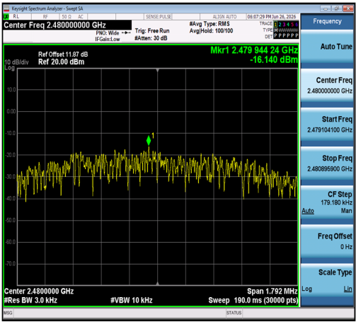
LE_2M-Ant1-2480-PASS
