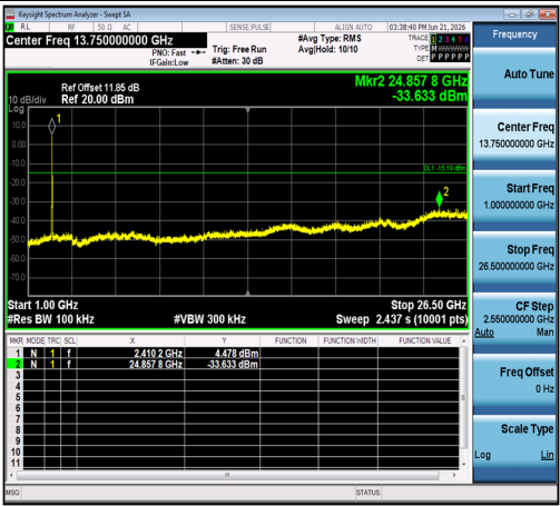
11AX20SISO-Ant1-2412-1000~26500-PASS
