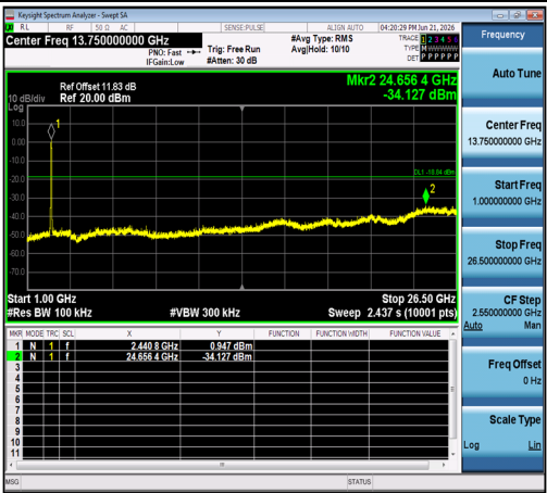
11AX40SISO-Ant1-2437-1000~26500-PASS
