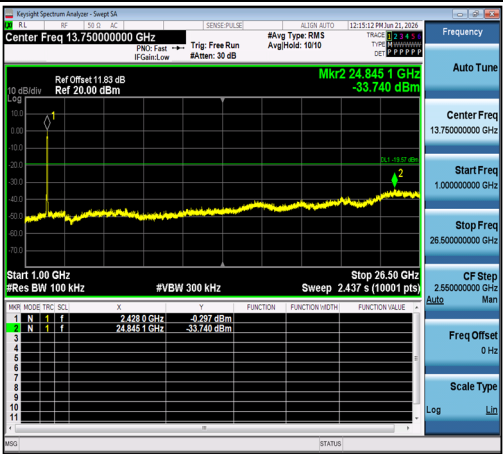
11N40SISO-Ant1-2437-1000~26500-PASS
