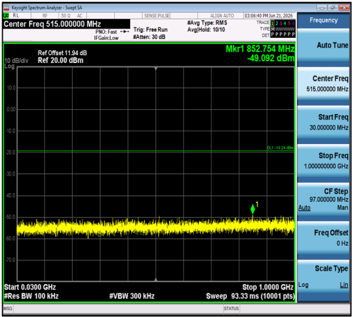
11N40SISO-Ant1-2452-30~1000-PASS
