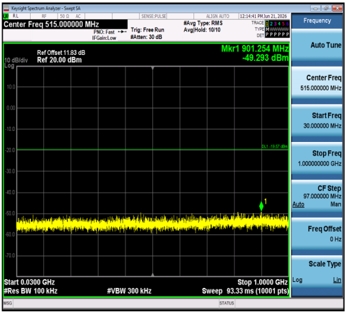
11N40SISO-Ant1-2437-30~1000-PASS
