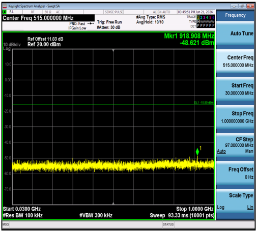
11AX20SISO-Ant1-2437-30~1000-PASS
