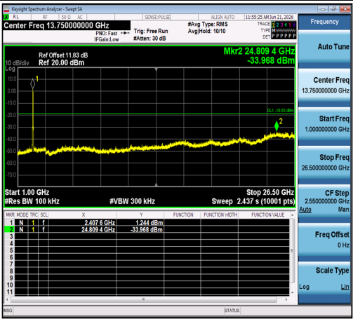
11N40SISO-Ant1-2422-1000~26500-PASS
