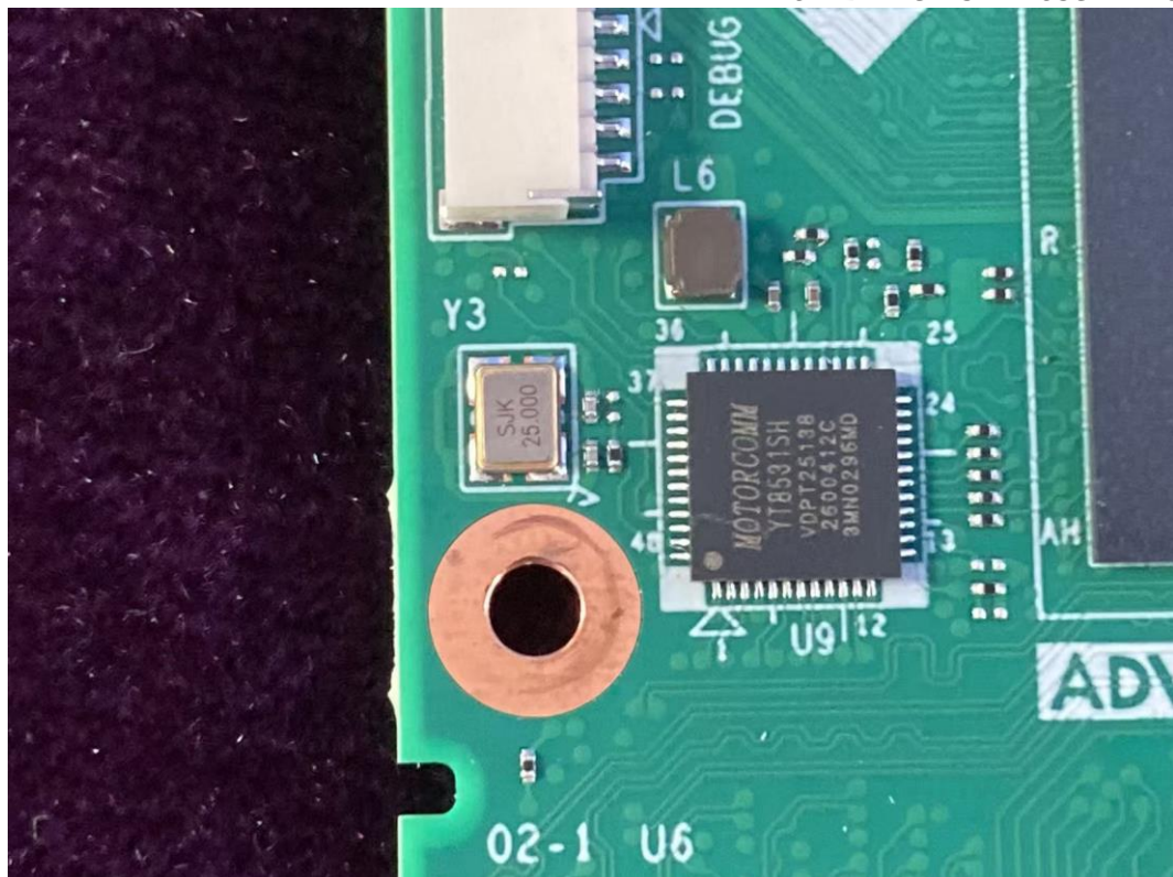
FIGURE 20 MULTI-INDUSTRY GENERAL PURPOSE SMART CONTROLLER (M/N: CMU3-R) BOARD 2 CRYSTAL OSCILLATOR 2
