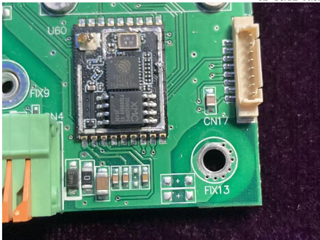
FIGURE 32 MULTI-INDUSTRY GENERAL PURPOSE SMART CONTROLLER (M/N: CMU3-R) RF BOARD FRONT 2
