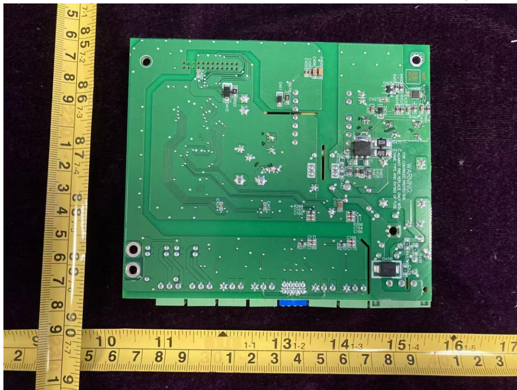
FIGURE 16 MULTI-INDUSTRY GENERAL PURPOSE SMART CONTROLLER (M/N: CMU3-R) BOARD 1 BACK
