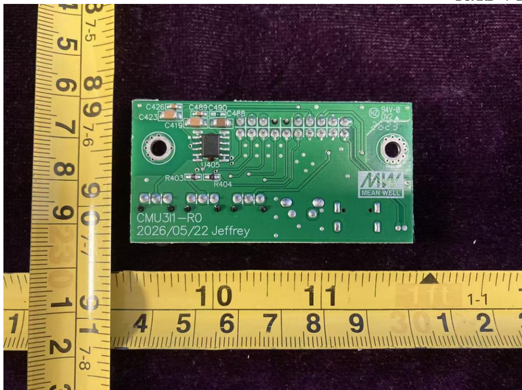
FIGURE 26 MULTI-INDUSTRY GENERAL PURPOSE SMART CONTROLLER (M/N: CMU3-R) BOARD 4 BACK
