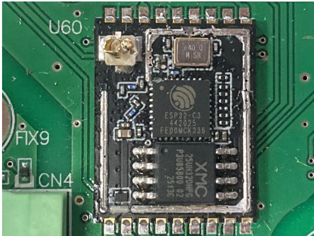
FIGURE 33 MULTI-INDUSTRY GENERAL PURPOSE SMART CONTROLLER (M/N: CMU3-R) RF BOARD FRONT 3
