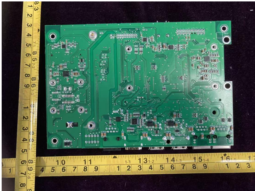
FIGURE 28 MULTI-INDUSTRY GENERAL PURPOSE SMART CONTROLLER (M/N: CMU3-R) BOARD 5 BACK
