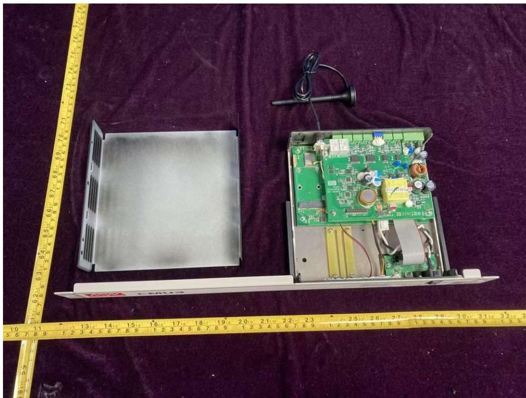
FIGURE 13 MULTI-INDUSTRY GENERAL PURPOSE SMART CONTROLLER (M/N: CMU3-R) COVER REMOVED 1
