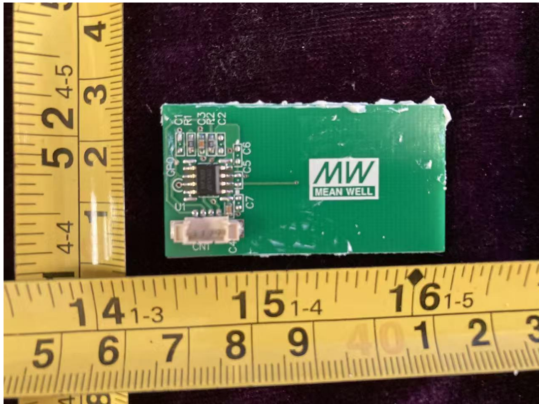
FIGURE 23 MULTI-INDUSTRY GENERAL PURPOSE SMART CONTROLLER (M/N: CMU3-R) BOARD 3 FRONT
