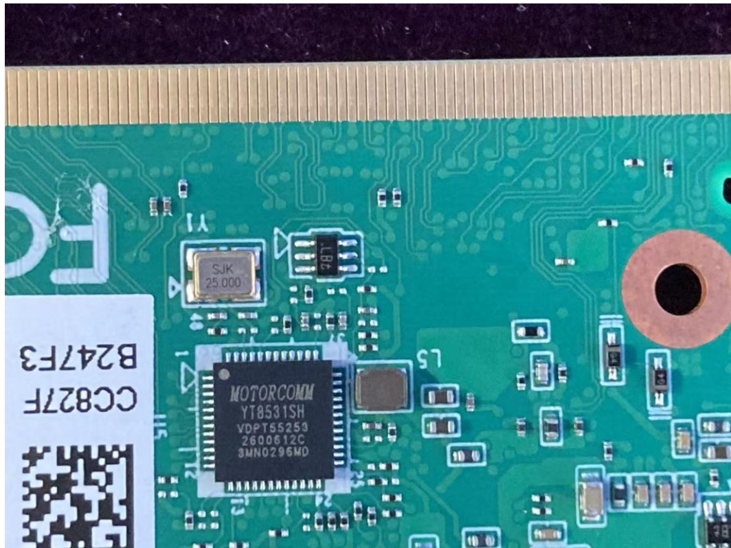
FIGURE 19 MULTI-INDUSTRY GENERAL PURPOSE SMART CONTROLLER (M/N: CMU3-R) BOARD 2 CRYSTAL OSCILLATOR 1
