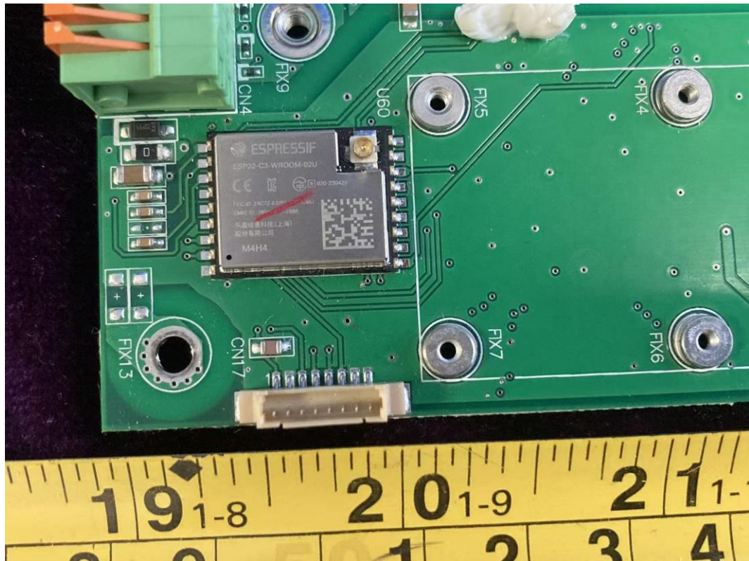
FIGURE 31 MULTI-INDUSTRY GENERAL PURPOSE SMART CONTROLLER (M/N: CMU3-R) RF BOARD FRONT 1
