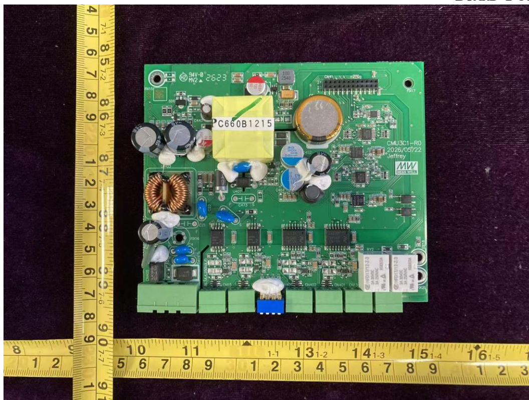
FIGURE 15 MULTI-INDUSTRY GENERAL PURPOSE SMART CONTROLLER (M/N: CMU3-R) BOARD 1 FRONT
