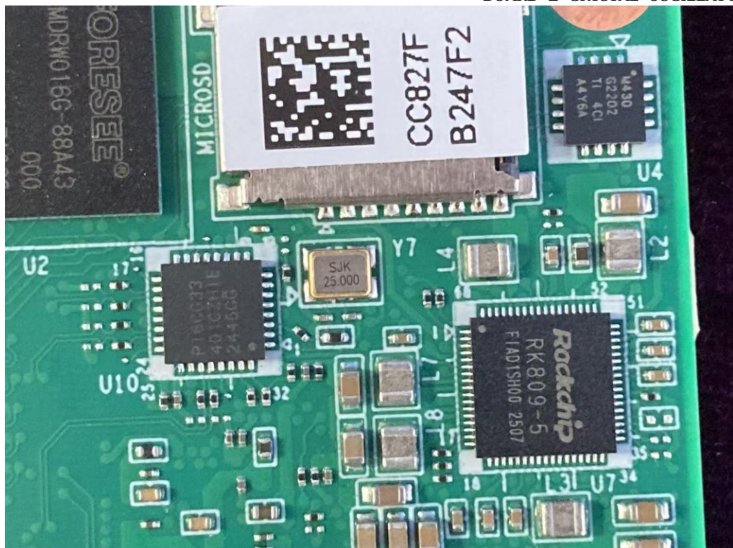
FIGURE 22 MULTI-INDUSTRY GENERAL PURPOSE SMART CONTROLLER (M/N: CMU3-R) BOARD 2 CRYSTAL OSCILLATOR 4
