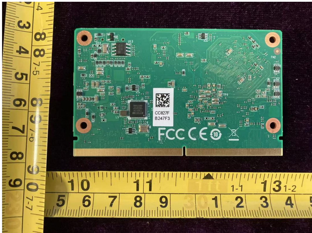
FIGURE 18 MULTI-INDUSTRY GENERAL PURPOSE SMART CONTROLLER (M/N: CMU3-R) BOARD 2 BACK
