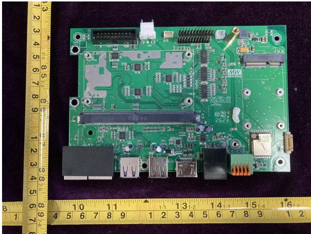
FIGURE 27 MULTI-INDUSTRY GENERAL PURPOSE SMART CONTROLLER (M/N: CMU3-R) BOARD 5 FRONT
