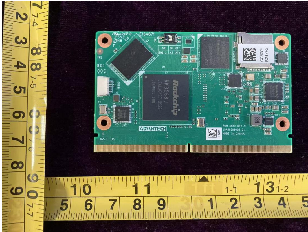
FIGURE 17 MULTI-INDUSTRY GENERAL PURPOSE SMART CONTROLLER (M/N: CMU3-R) BOARD 2 FRONT
