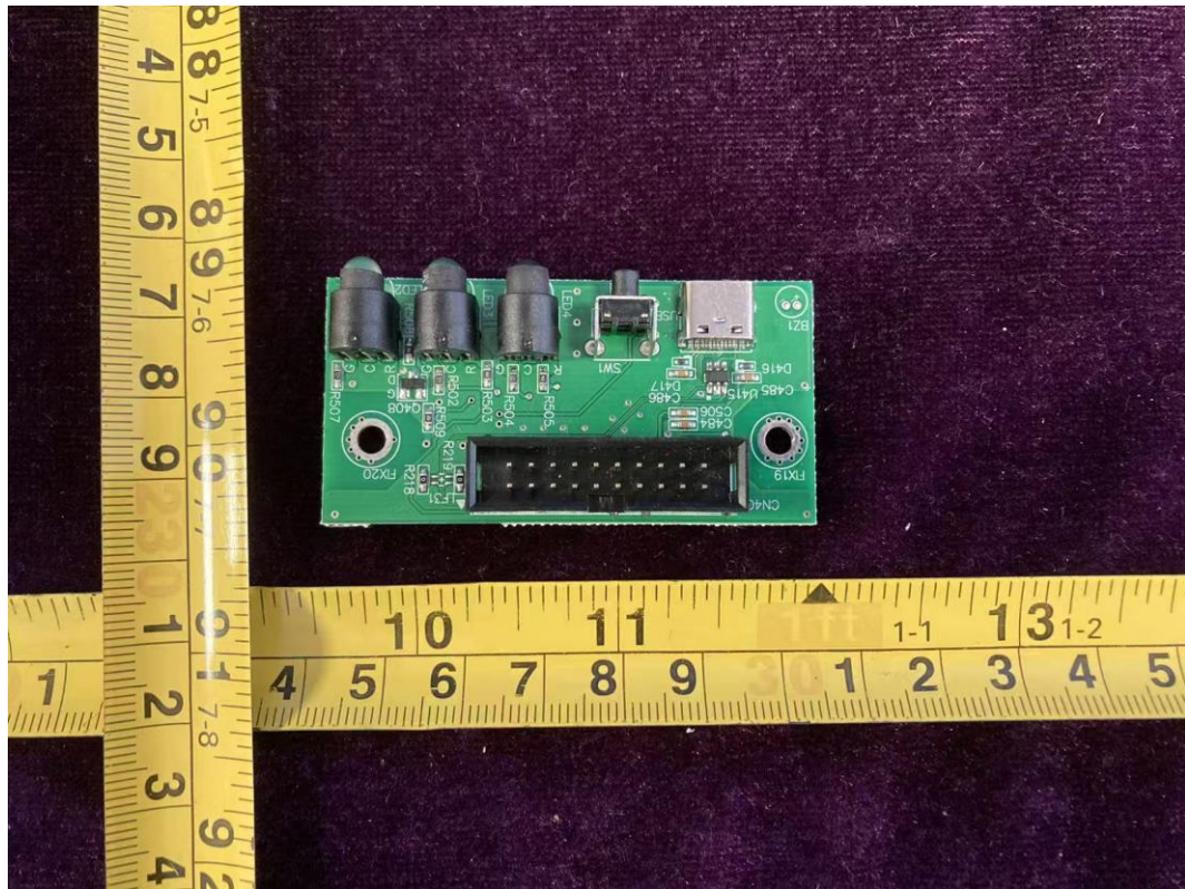
FIGURE 25 MULTI-INDUSTRY GENERAL PURPOSE SMART CONTROLLER (M/N: CMU3-R) BOARD 4 FRONT
