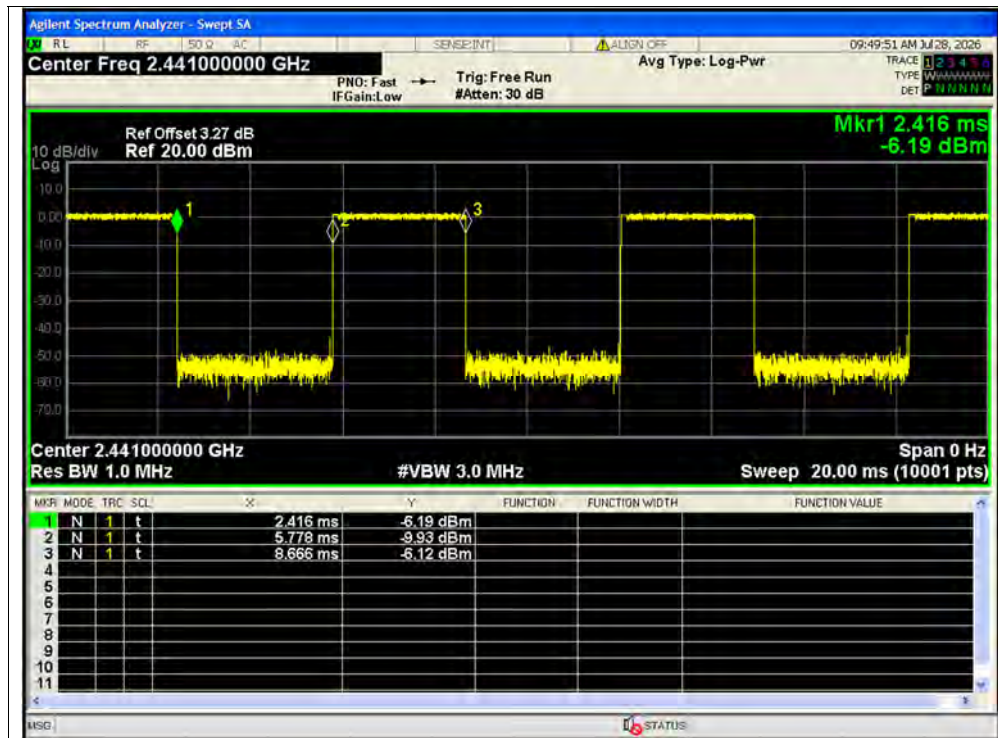
Duty Cycle NVNT 2-DH5 2441MHz Ant1
