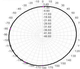
Total(H-XY), Max= 1.56dBi, CirD=4.51
