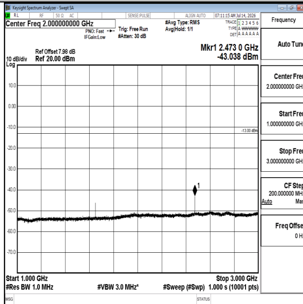
Band5-5MHz-QPSK-20425-1RB#0-1000~3000-PASS
