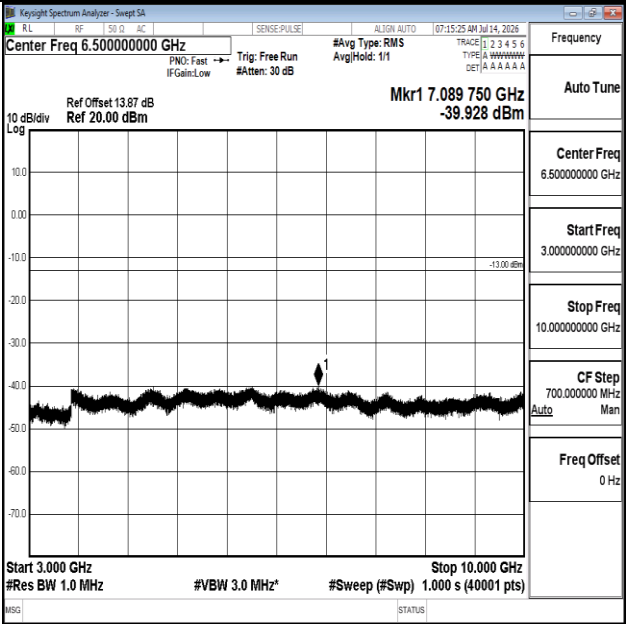
Band5-5MHz-16QAM-20625-1RB#0-3000~10000-PASS
