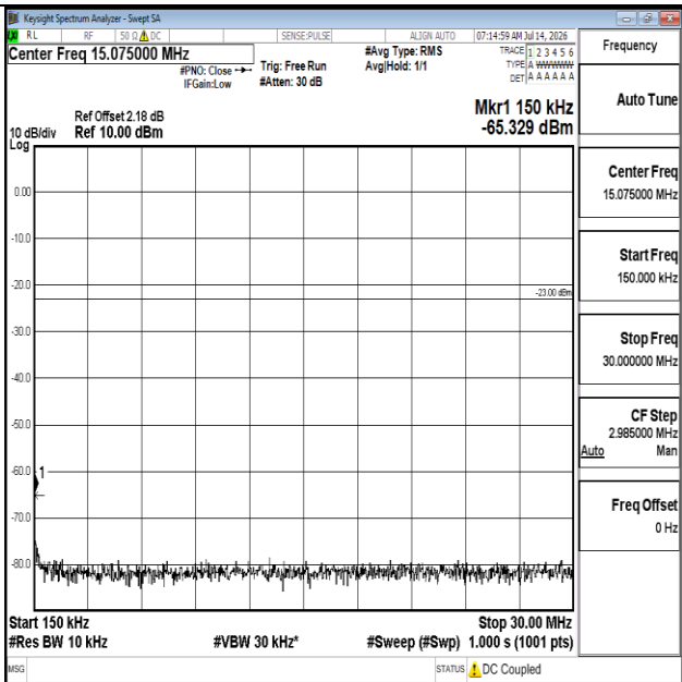
Band5-5MHz-16QAM-20625-1RB#0-0.15~30-PASS
