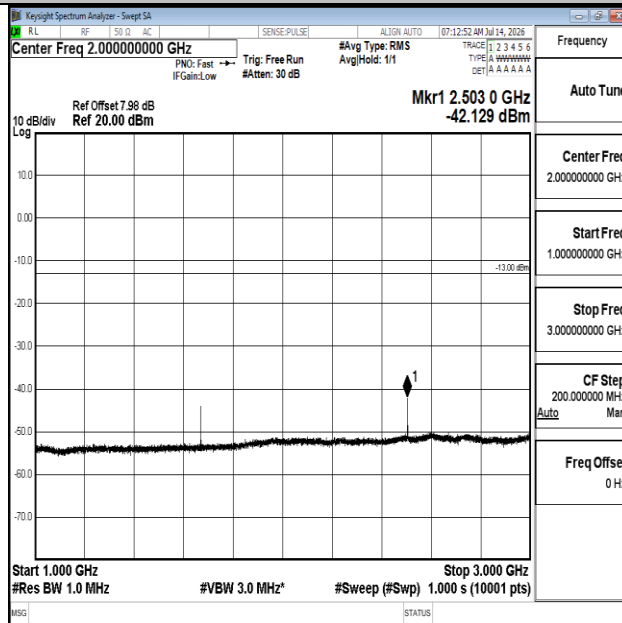
Band5-5MHz-QPSK-20525-1RB#0-1000~3000-PASS
