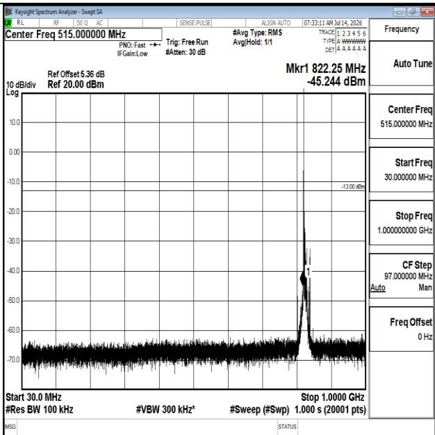
Band5-10MHz-QPSK-20450-1RB#0-30~1000-PASS
