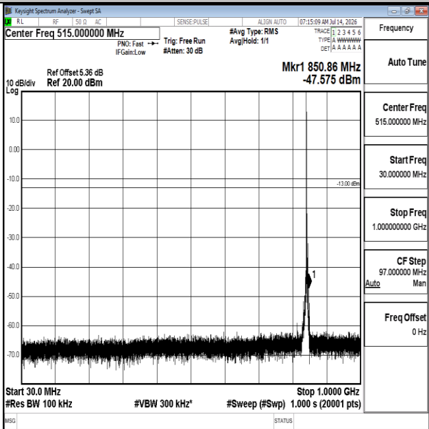
Band5-5MHz-16QAM-20625-1RB#0-30~1000-PASS
