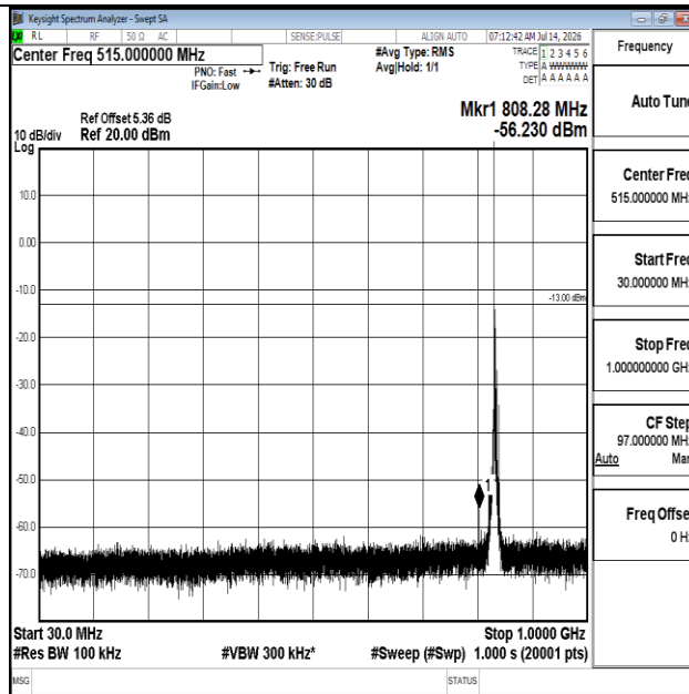
Band5-5MHz-QPSK-20525-1RB#0-30~1000-PASS
