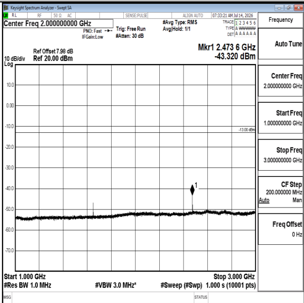
Band5-10MHz-QPSK-20450-1RB#0-1000~3000-PASS
