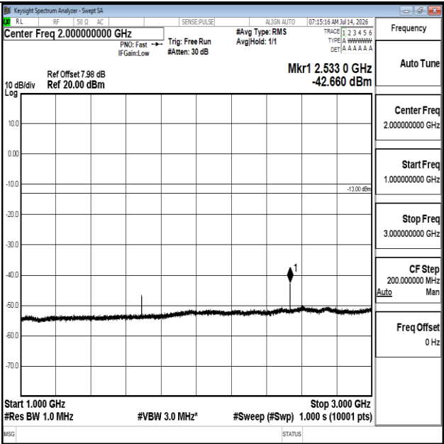
Band5-5MHz-16QAM-20625-1RB#0-1000~3000-PASS
