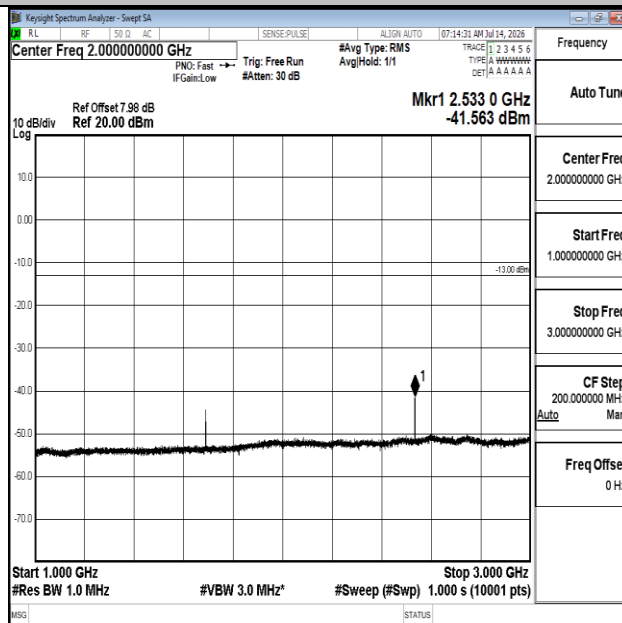
Band5-5MHz-QPSK-20625-1RB#0-1000~3000-PASS
