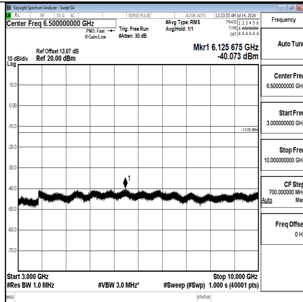
Band12-1.4MHz-QPSK-23017-1RB#0-3000~10000-PASS
