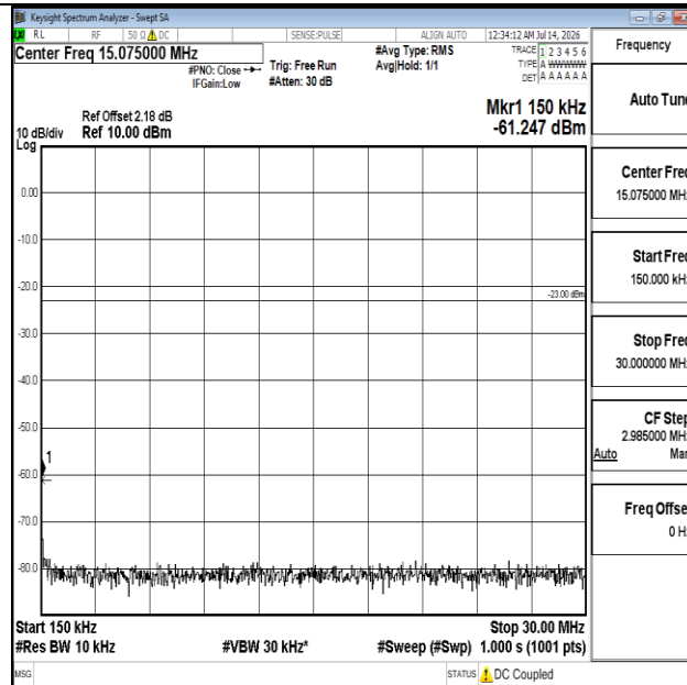
Band12-1.4MHz-16QAM-23017-1RB#0-0.15~30-PASS
