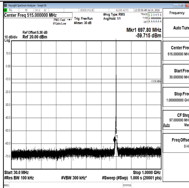
Band12-1.4MHz-16QAM-23095-1RB#0-30~1000-PASS
