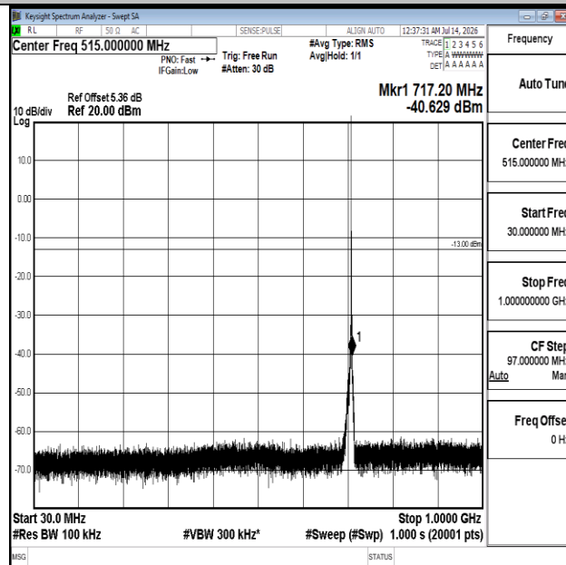
Band12-1.4MHz-16QAM-23173-1RB#0-30~1000-PASS
