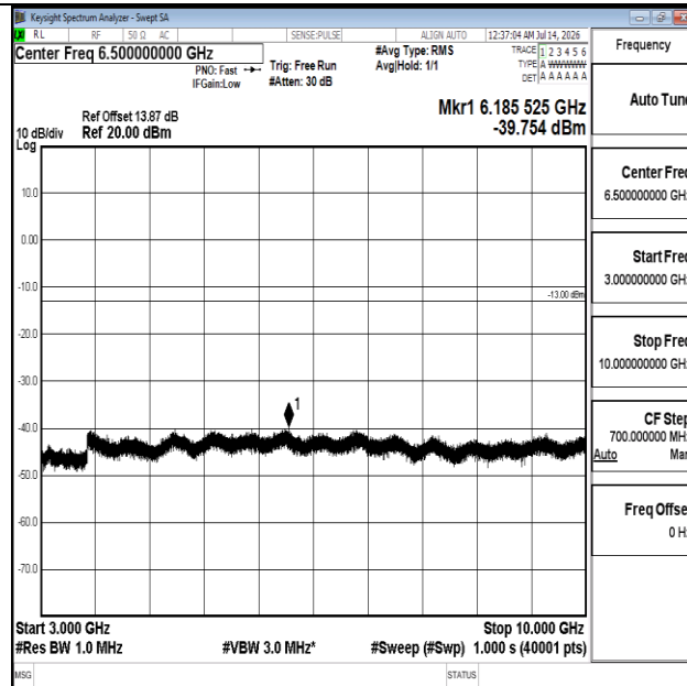
Band12-1.4MHz-QPSK-23173-1RB#0-3000~10000-PASS
