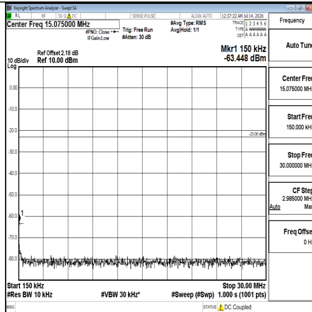
Band12-1.4MHz-16QAM-23173-1RB#0-0.15~30-PASS
