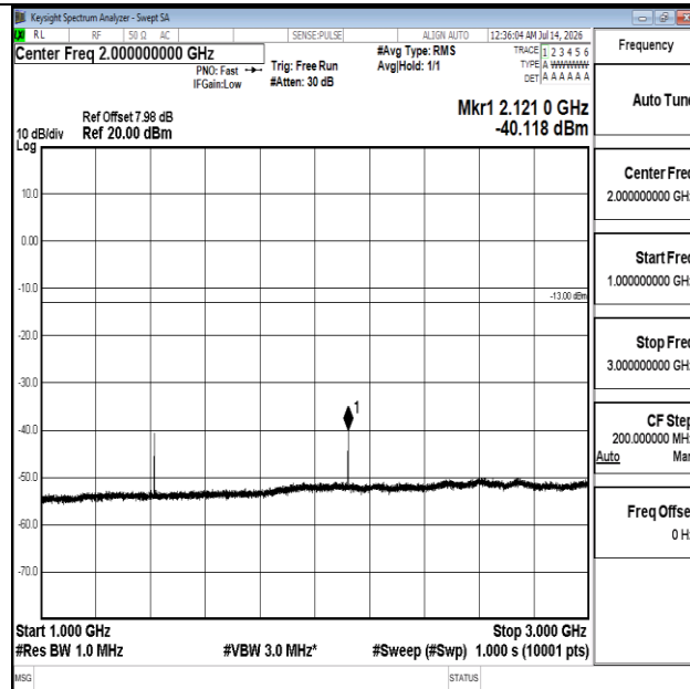
Band12-1.4MHz-16QAM-23095-1RB#0-1000~3000-PASS
