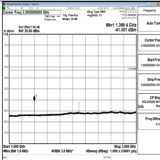
Band12-3MHz-16QAM-23025-1RB#0-1000~3000-PASS
