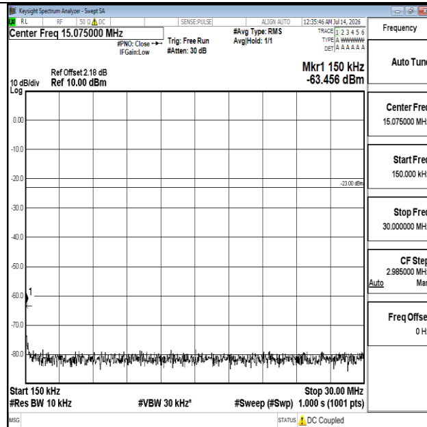
Band12-1.4MHz-16QAM-23095-1RB#0-0.15~30-PASS
