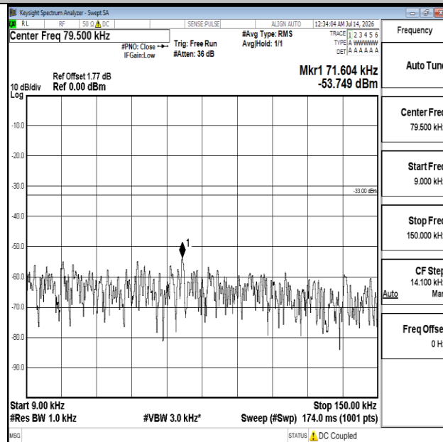
Band12-1.4MHz-16QAM-23017-1RB#0-0.009~0.15-PASS
