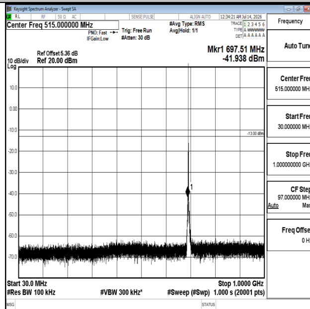
Band12-1.4MHz-16QAM-23017-1RB#0-30~1000-PASS
