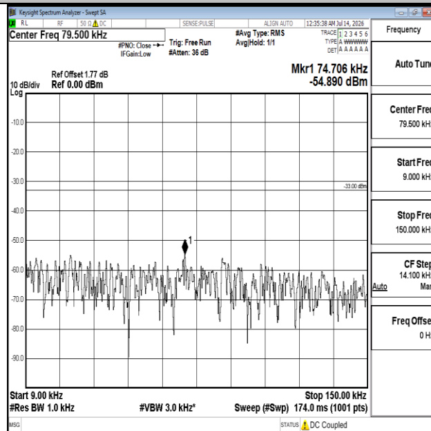
Band12-1.4MHz-16QAM-23095-1RB#0-0.009~0.15-PASS
