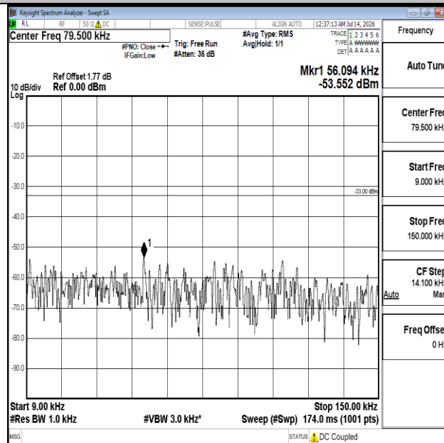
Band12-1.4MHz-16QAM-23173-1RB#0-0.009~0.15-PASS
