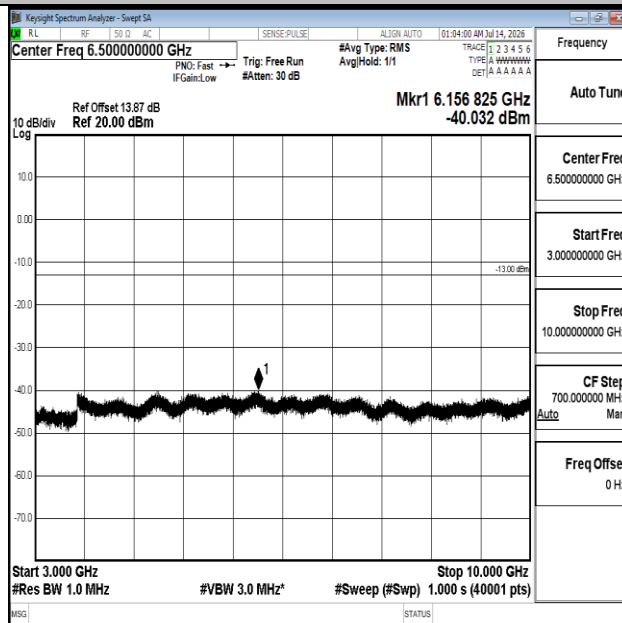
Band12-3MHz-16QAM-23025-1RB#0-3000~10000-PASS
