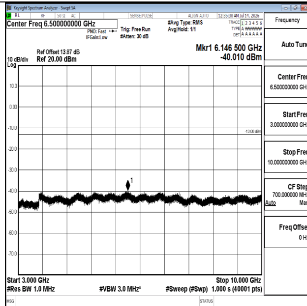
Band12-1.4MHz-QPSK-23095-1RB#0-3000~10000-PASS
