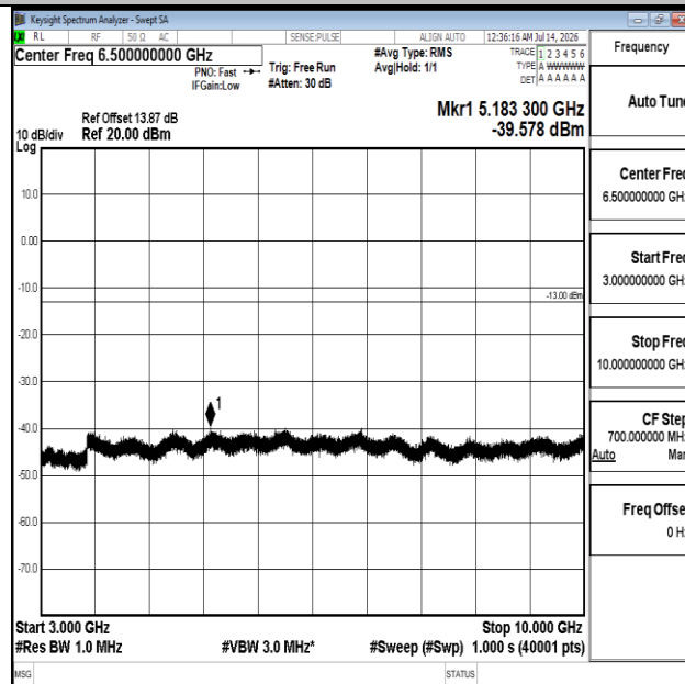
Band12-1.4MHz-16QAM-23095-1RB#0-3000~10000-PASS
