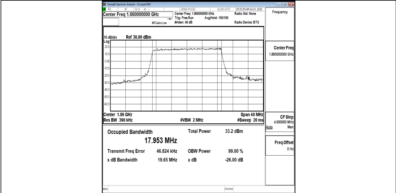
Band25-20MHz-16QAM-26140-100RB#0-PASS
