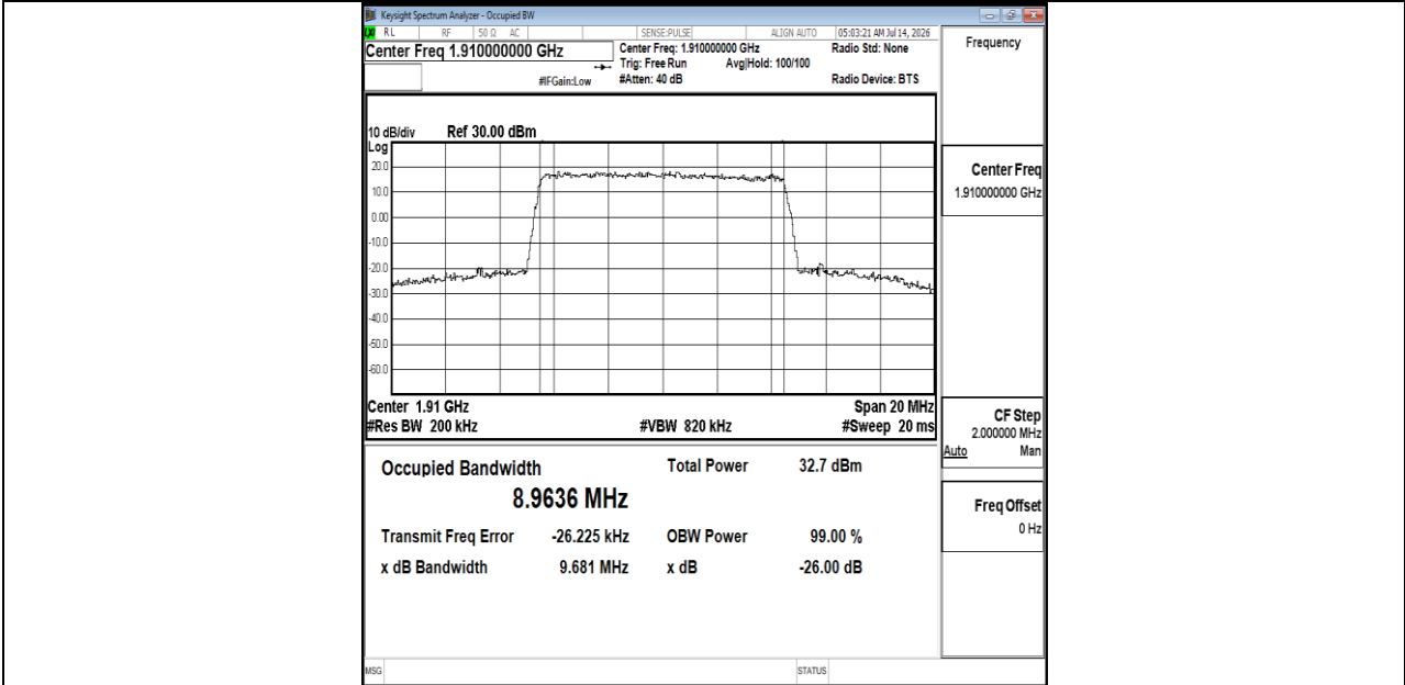
Band25-10MHz-16QAM-26640-50RB#0-PASS
