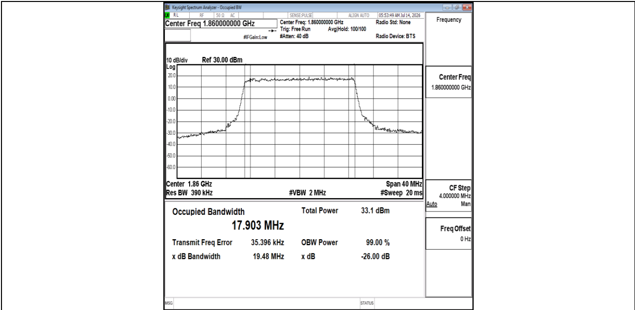
Band25-20MHz-QPSK-26140-100RB#0-PASS
