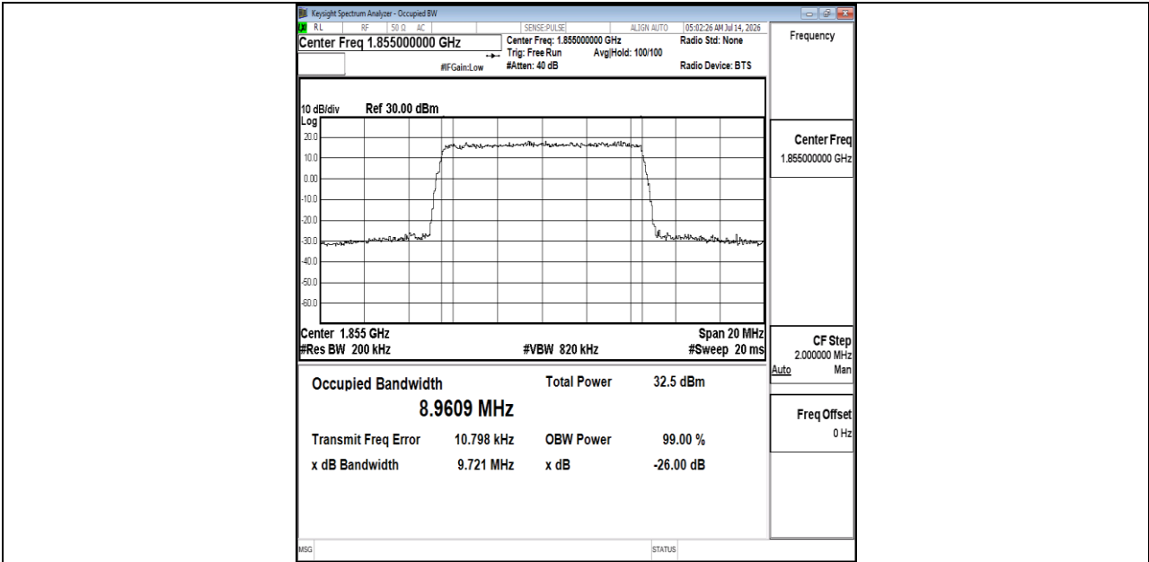
Band25-10MHz-QPSK-26090-50RB#0-PASS
