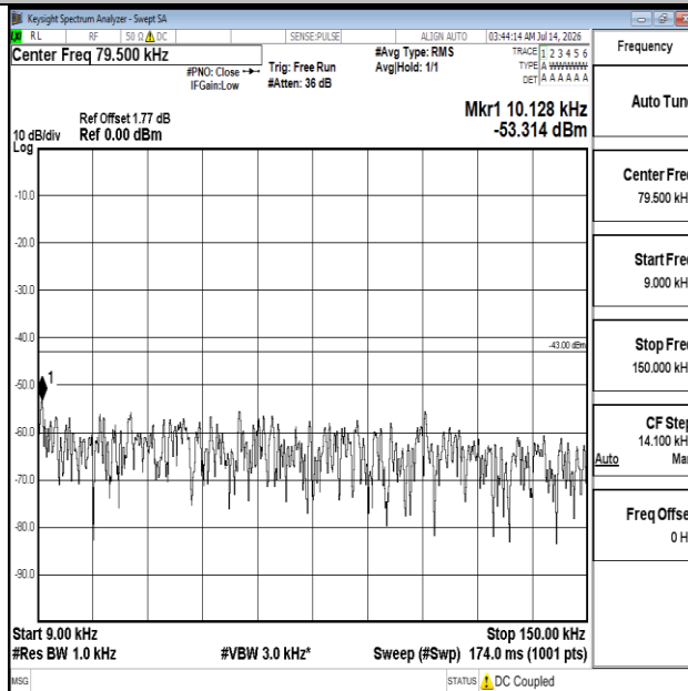
Band25-1.4MHz-16QAM-26365-1RB#0-0.009~0.15-PASS
