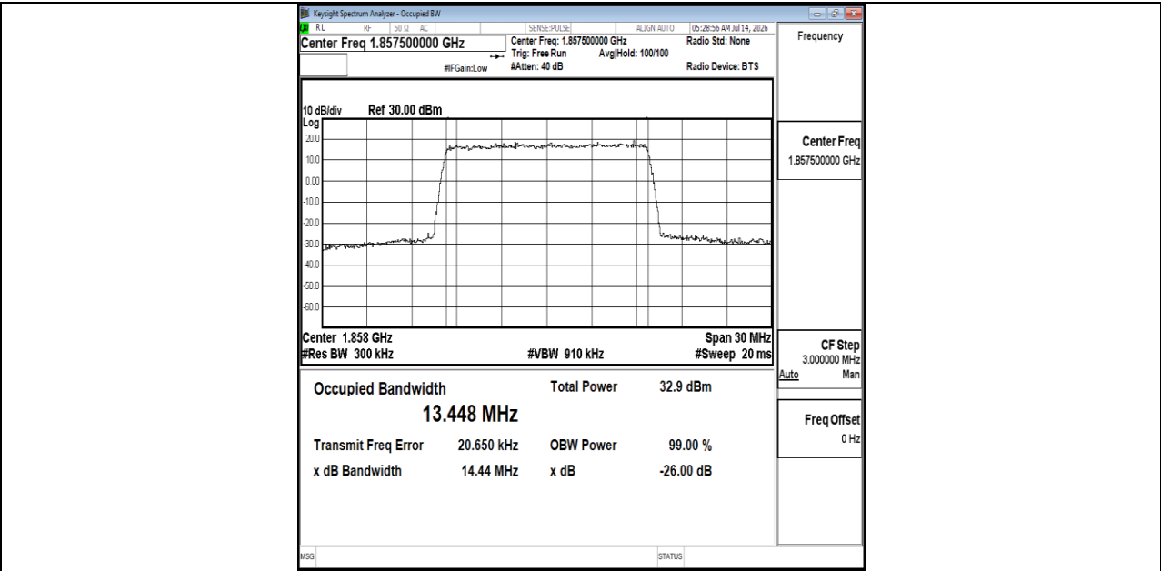
Band25-15MHz-QPSK-26115-75RB#0-PASS
