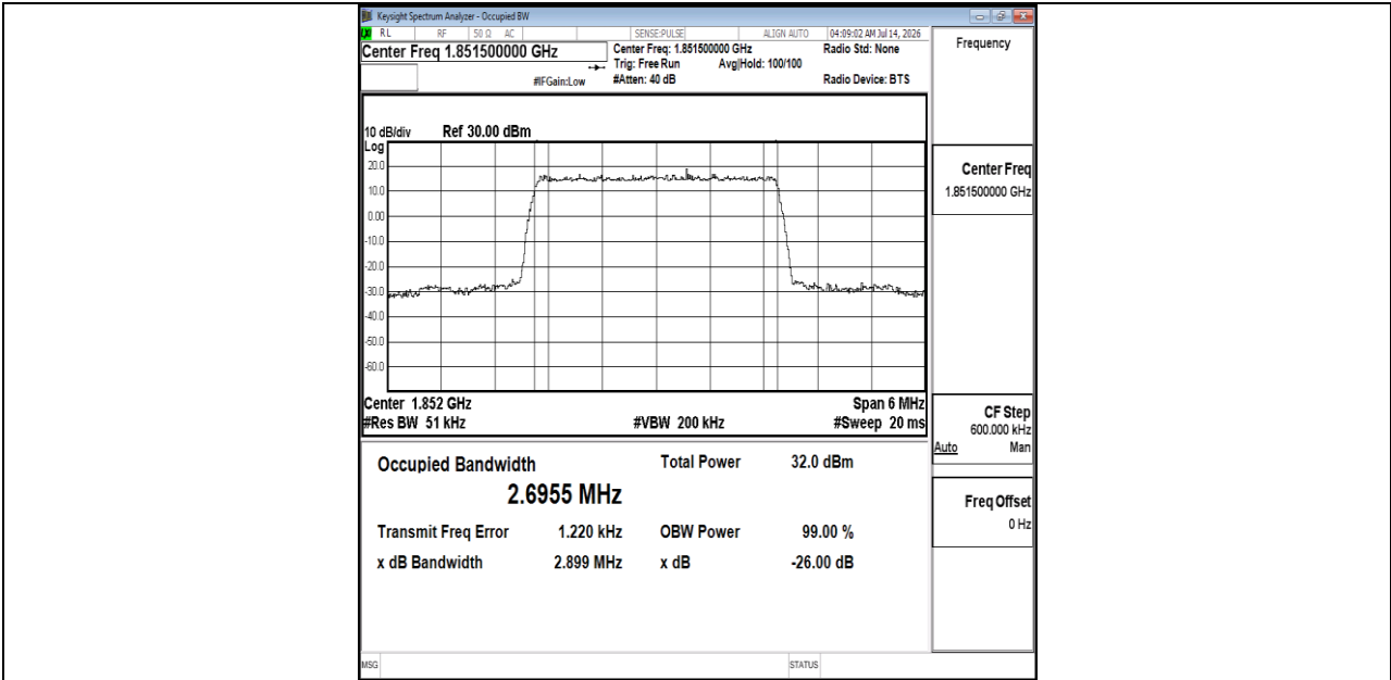
Band25-3MHz-QPSK-26055-15RB#0-PASS
