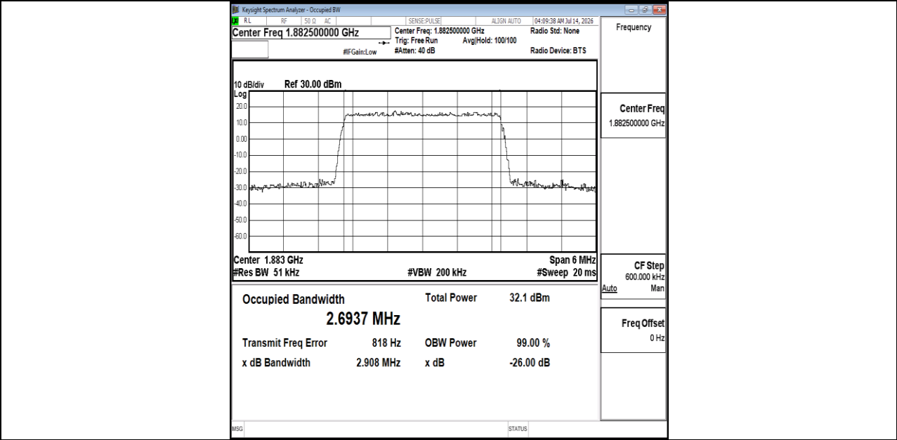
Band25-3MHz-16QAM-26365-15RB#0-PASS
