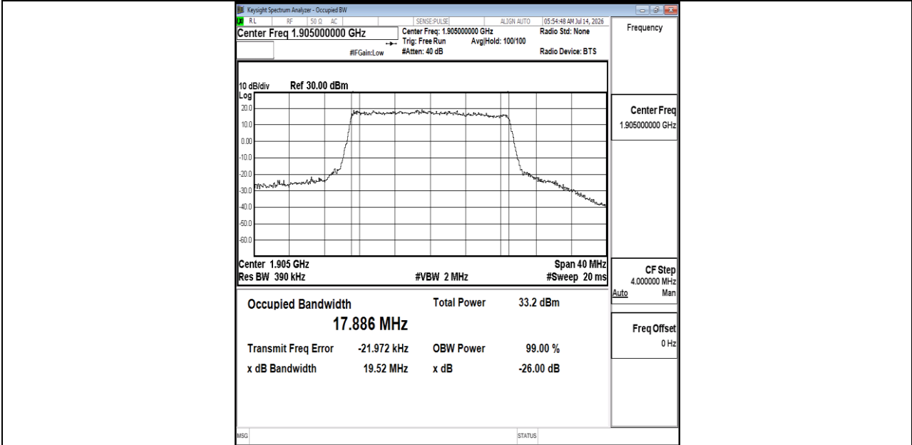
Band25-20MHz-16QAM-26590-100RB#0-PASS
