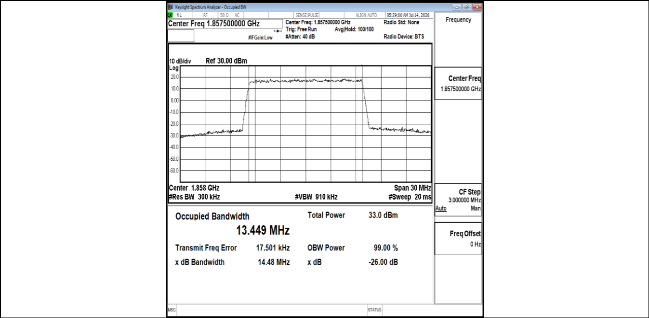
Band25-15MHz-16QAM-26115-75RB#0-PASS
