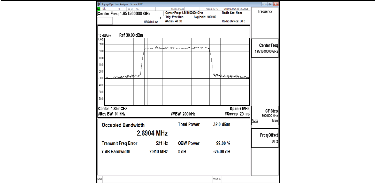
Band25-3MHz-16QAM-26055-15RB#0-PASS
