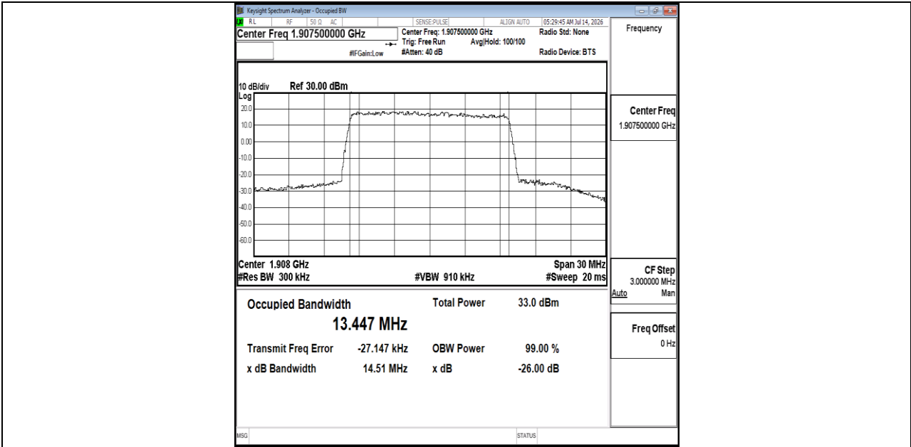
Band25-15MHz-QPSK-26615-75RB#0-PASS
