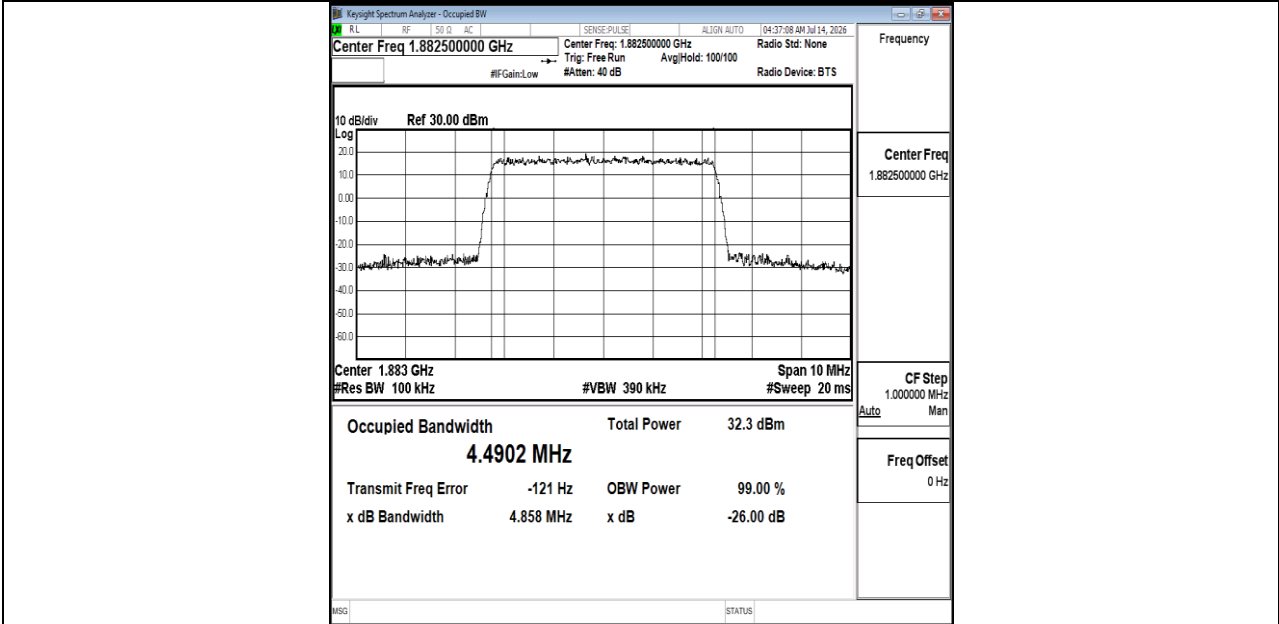
Band25-5MHz-16QAM-26365-25RB#0-PASS
