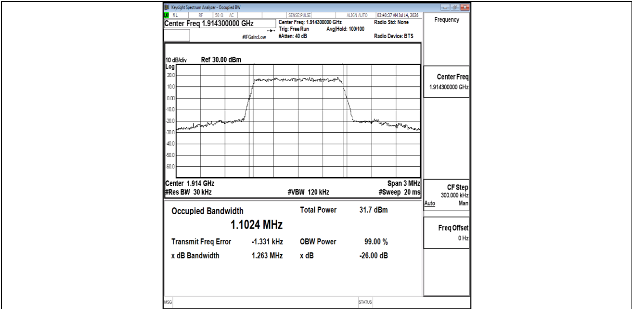
Band25-1.4MHz-QPSK-26683-6RB#0-PASS
