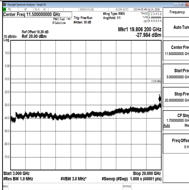
Band25-1.4MHz-QPSK-26365-1RB#0-3000~20000-PASS
