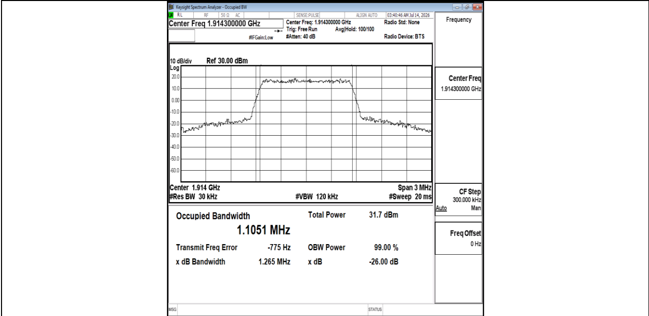
Band25-1.4MHz-16QAM-26683-6RB#0-PASS
