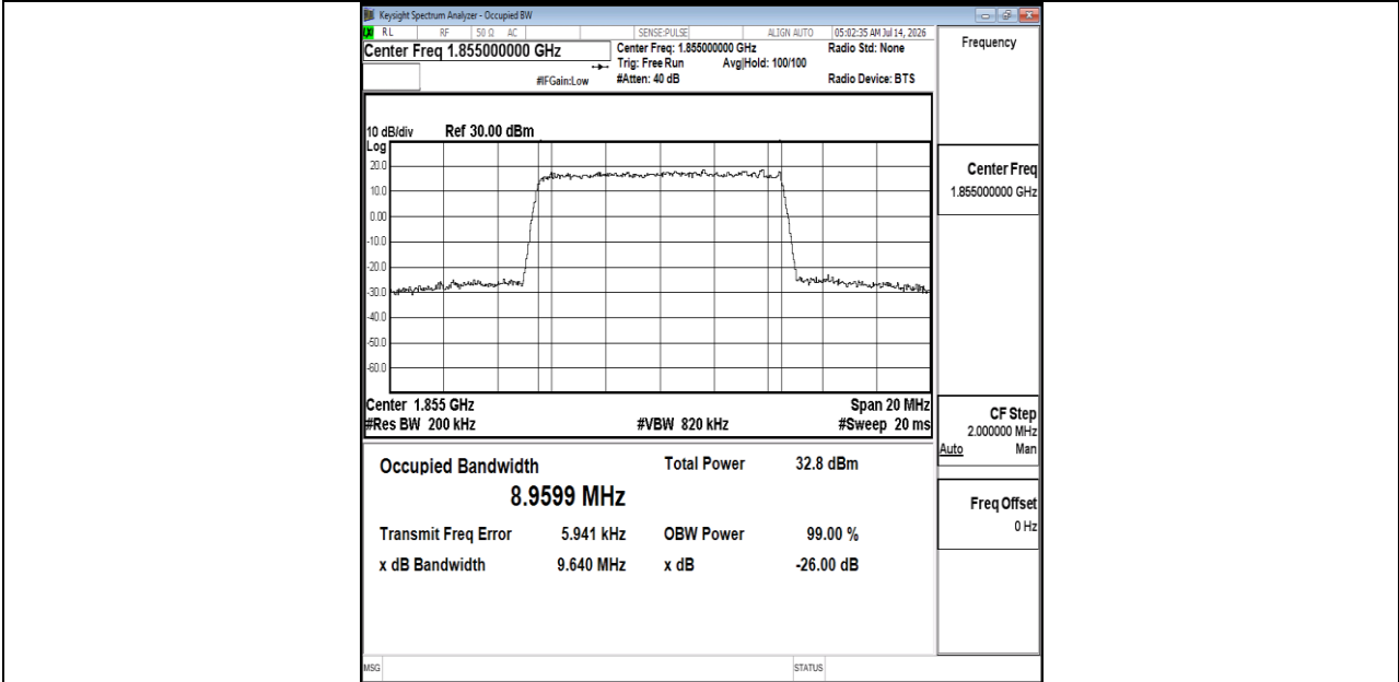
Band25-10MHz-16QAM-26090-50RB#0-PASS
