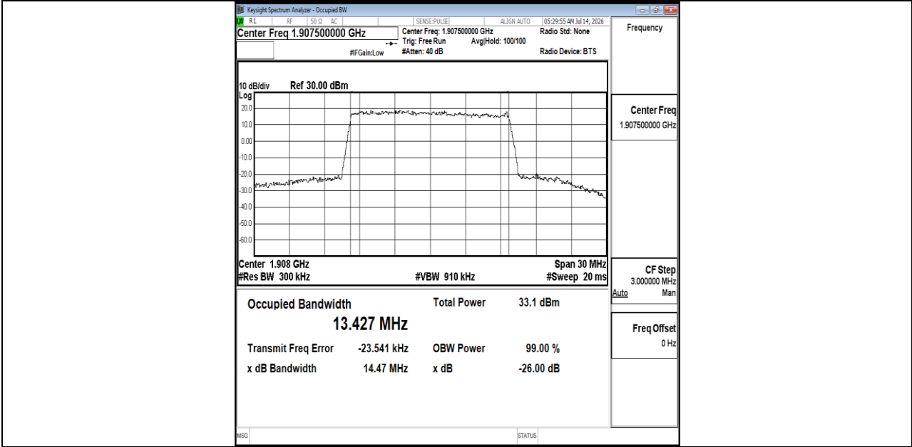
Band25-15MHz-16QAM-26615-75RB#0-PASS
