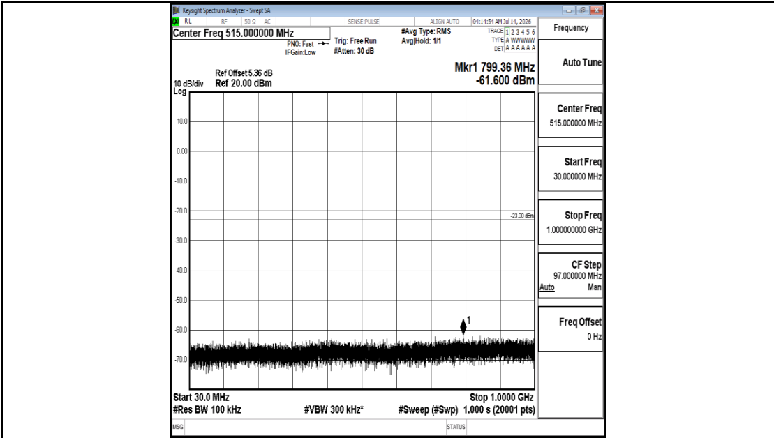
Band25-3MHz-QPSK-26675-1RB#0-30~1000-PASS
