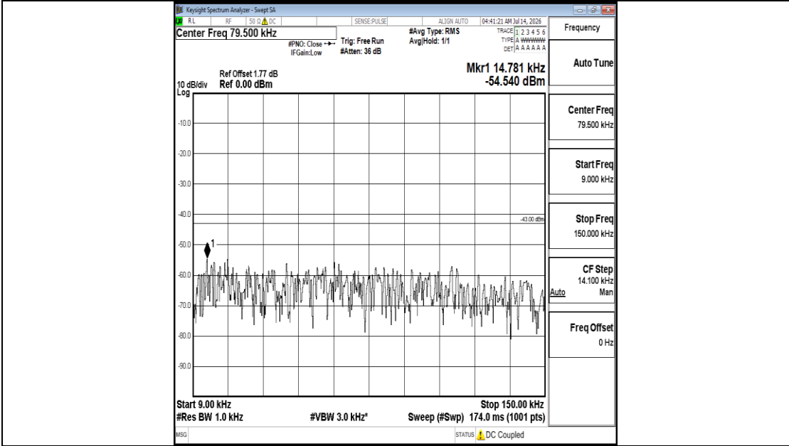
Band25-5MHz-16QAM-26365-1RB#0-0.009~0.15-PASS
