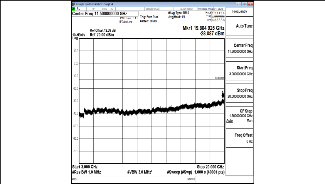
Band25-5MHz-16QAM-26665-1RB#0-3000~20000-PASS
