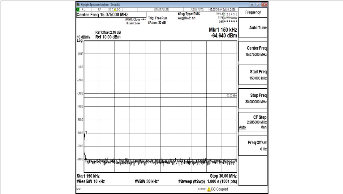
Band25-10MHz-16QAM-26090-1RB#0-0.15~30-PASS
