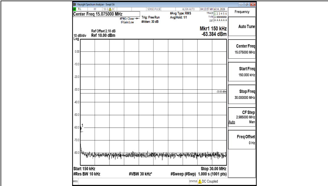
Band25-3MHz-16QAM-26365-1RB#0-0.15~30-PASS
