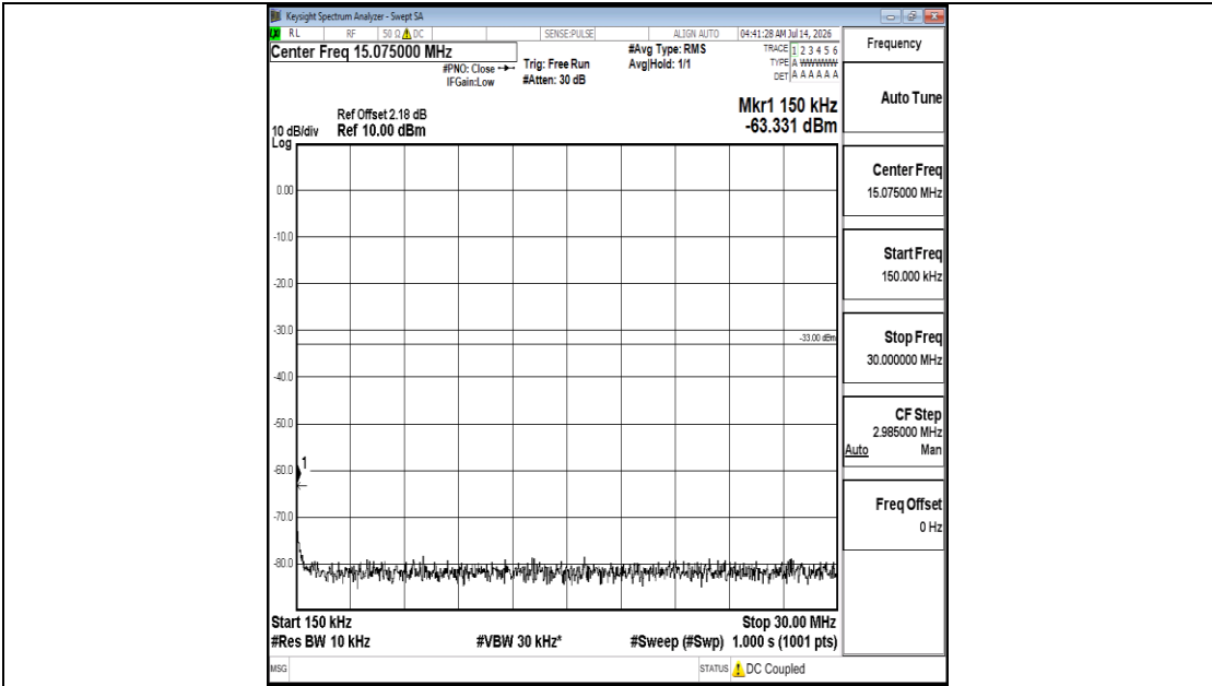
Band25-5MHz-16QAM-26365-1RB#0-0.15~30-PASS
