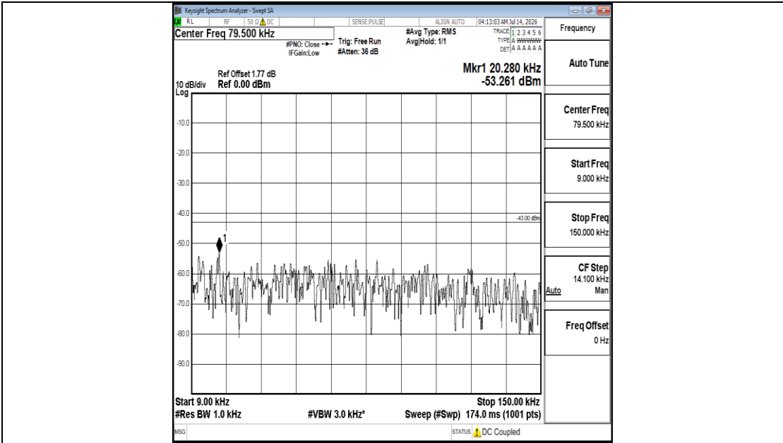
Band25-3MHz-QPSK-26365-1RB#0-0.009~0.15-PASS
