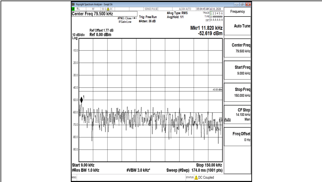
Band25-10MHz-QPSK-26090-1RB#0-0.009~0.15-PASS
