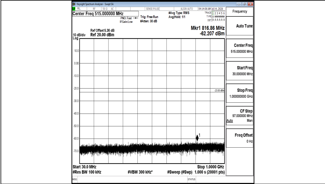
Band25-3MHz-16QAM-26365-1RB#0-30~1000-PASS
