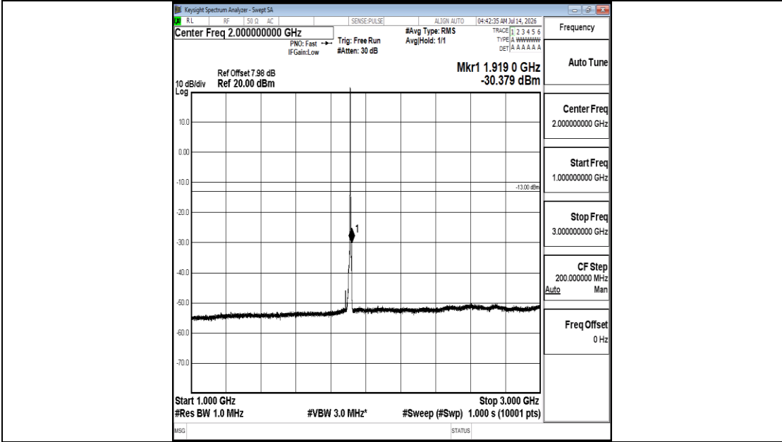
Band25-5MHz-QPSK-26665-1RB#0-1000~3000-PASS
