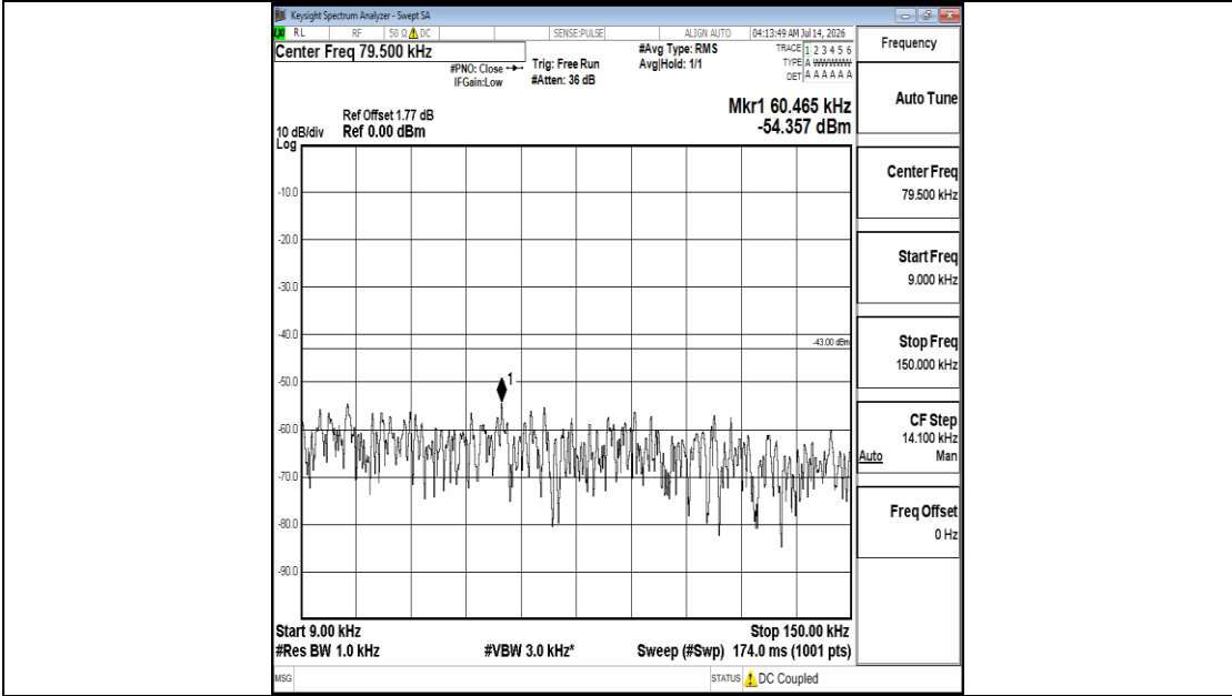
Band25-3MHz-16QAM-26365-1RB#0-0.009~0.15-PASS
