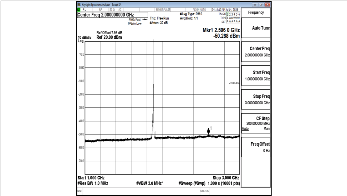
Band25-3MHz-16QAM-26365-1RB#0-1000~3000-PASS
