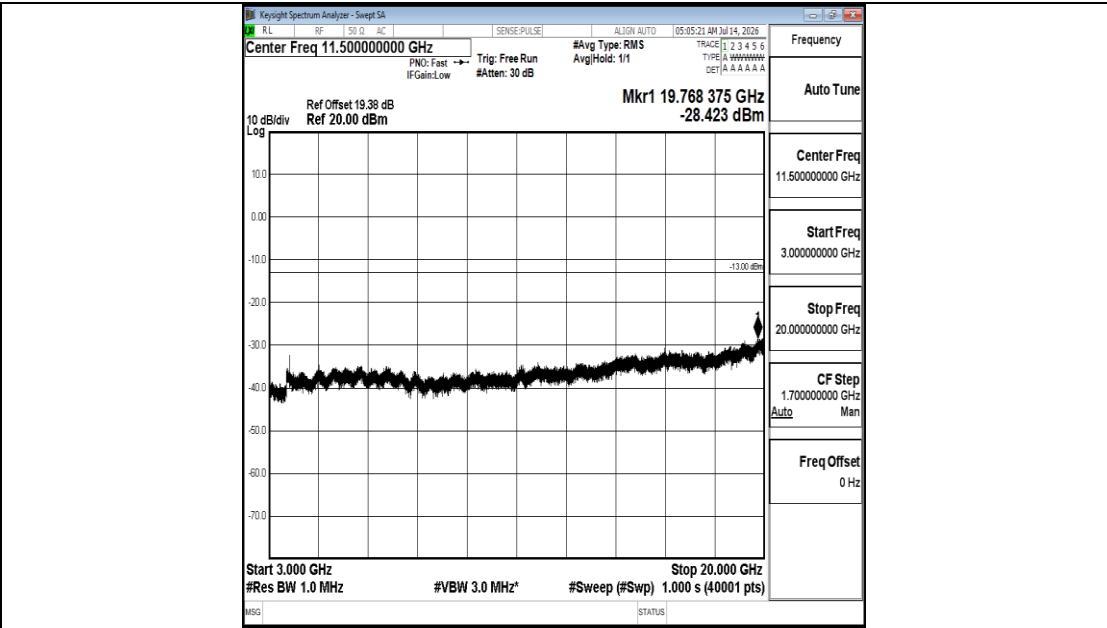
Band25-10MHz-QPSK-26090-1RB#0-3000~20000-PASS
