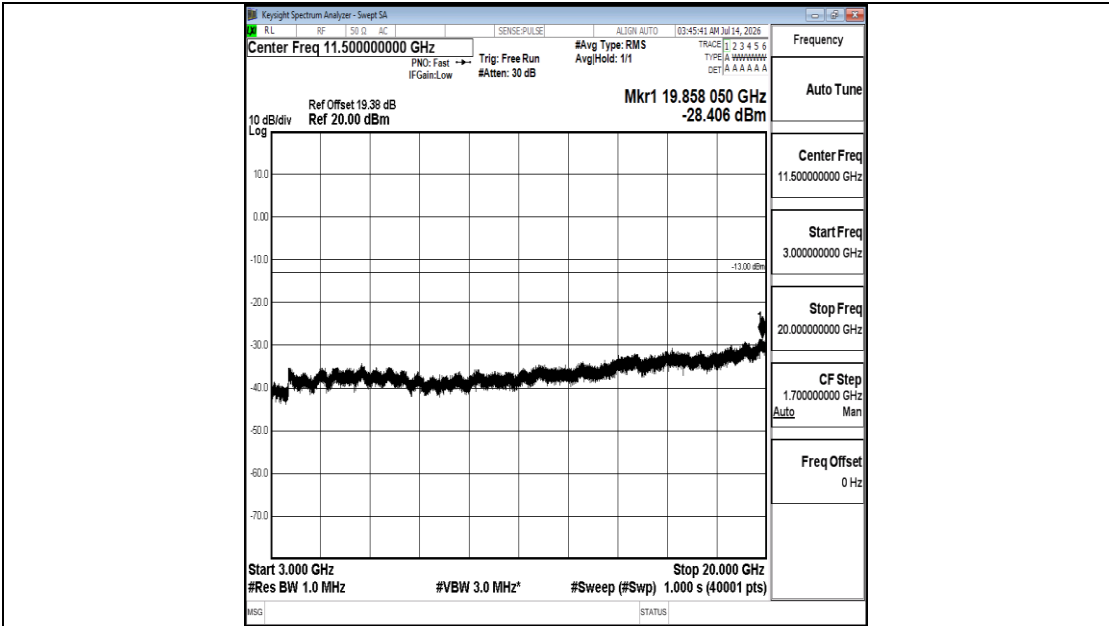
Band25-1.4MHz-QPSK-26683-1RB#0-3000~20000-PASS
