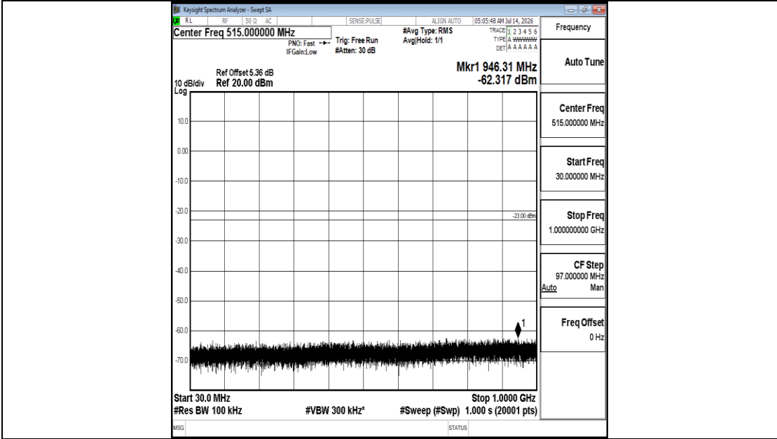
Band25-10MHz-16QAM-26090-1RB#0-30~1000-PASS
