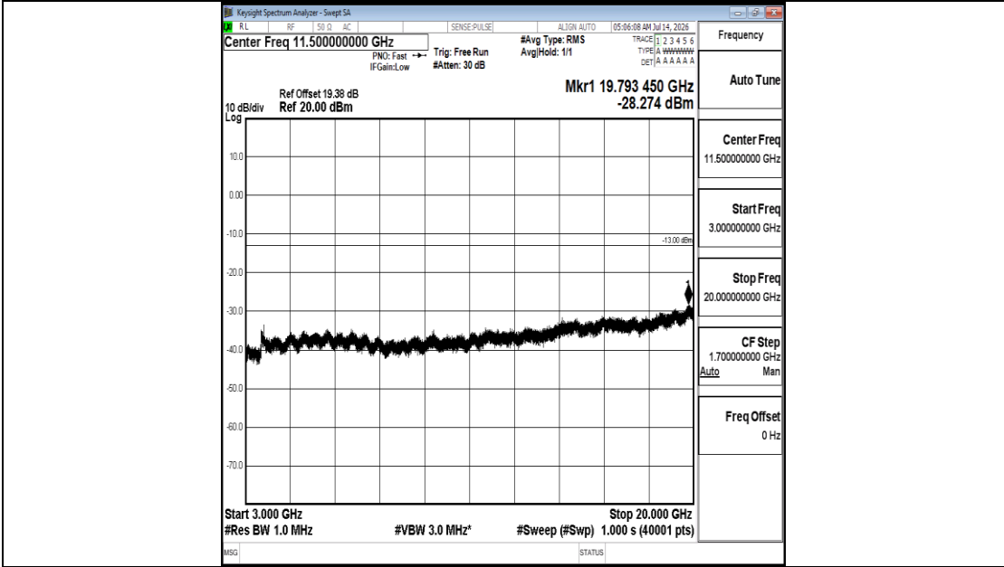
Band25-10MHz-16QAM-26090-1RB#0-3000~20000-PASS
