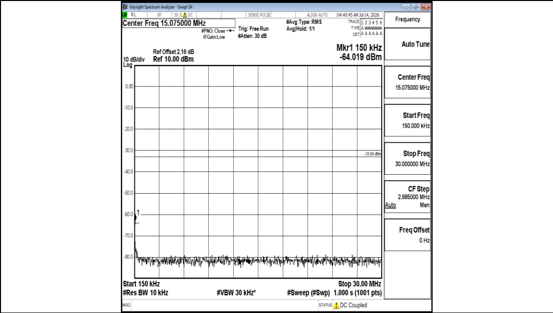
Band25-5MHz-QPSK-26365-1RB#0-0.15~30-PASS
