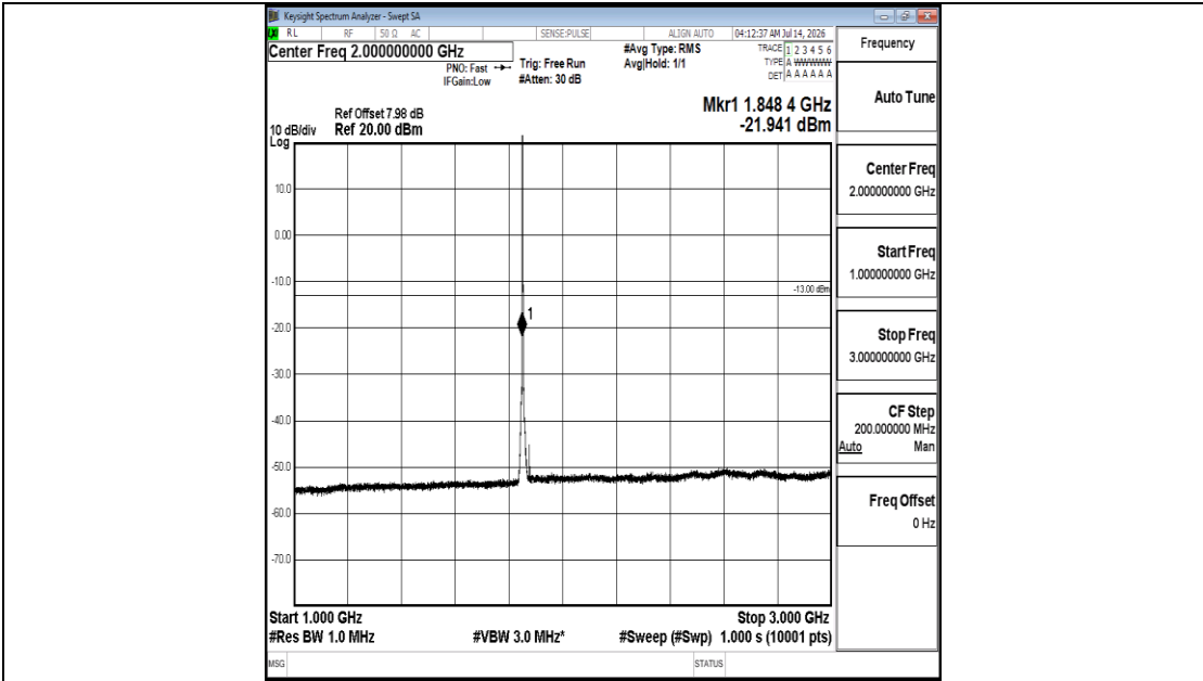
Band25-3MHz-16QAM-26055-1RB#0-1000~3000-PASS
