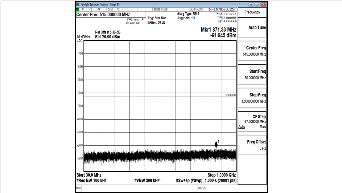
Band25-5MHz-QPSK-26365-1RB#0-30~1000-PASS
