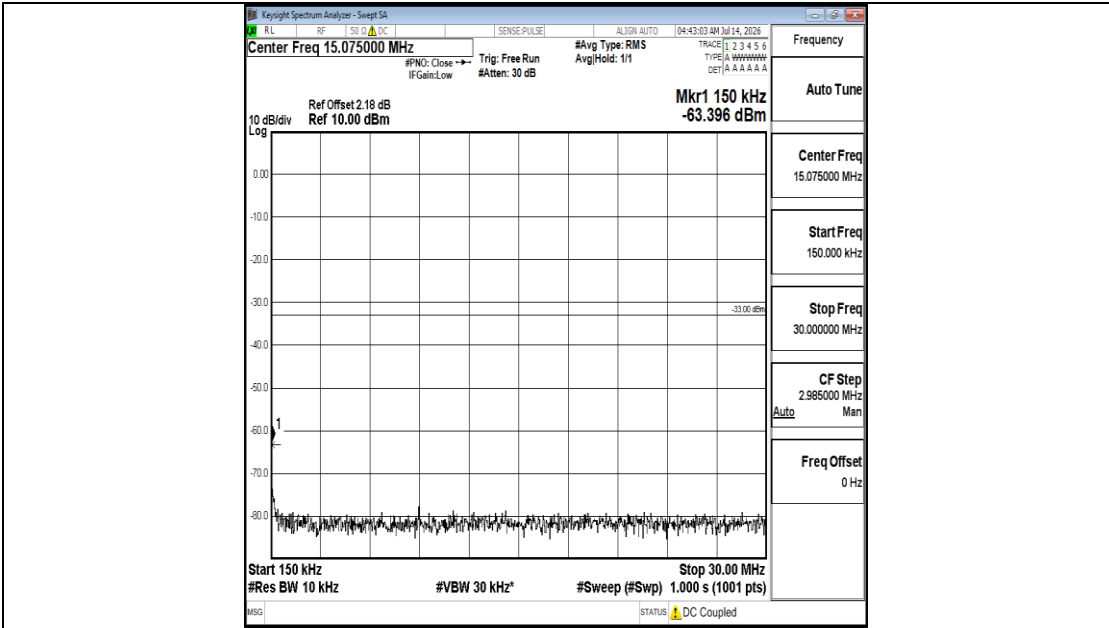
Band25-5MHz-16QAM-26665-1RB#0-0.15~30-PASS
