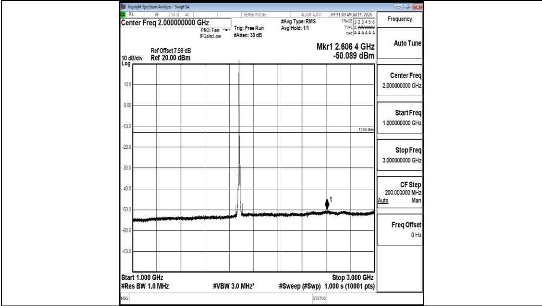
Band25-5MHz-QPSK-26365-1RB#0-1000~3000-PASS
