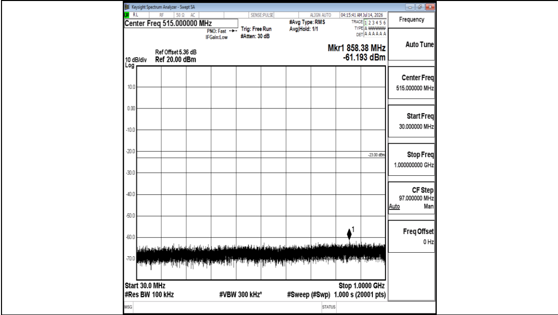
Band25-3MHz-16QAM-26675-1RB#0-30~1000-PASS
