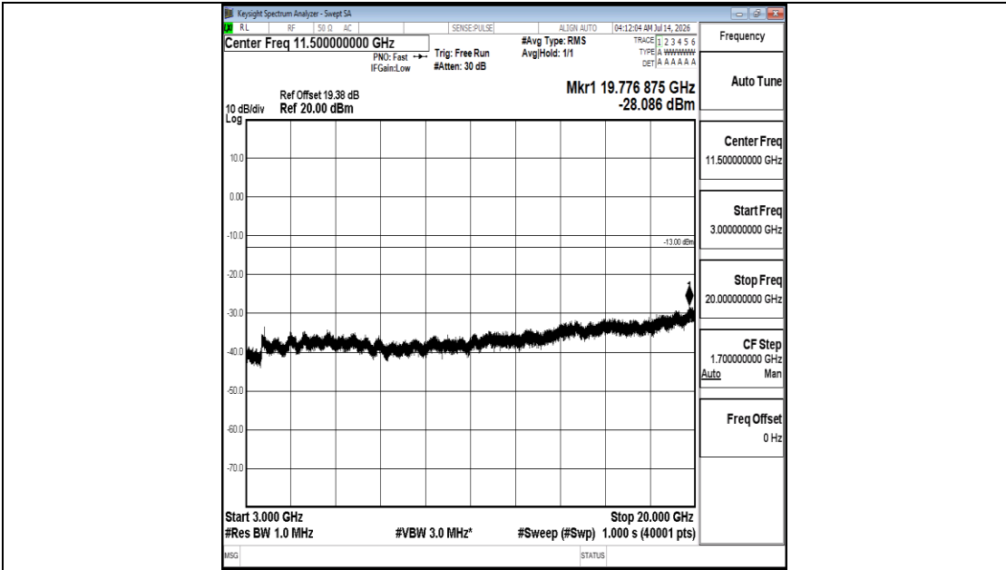
Band25-3MHz-QPSK-26055-1RB#0-3000~20000-PASS
