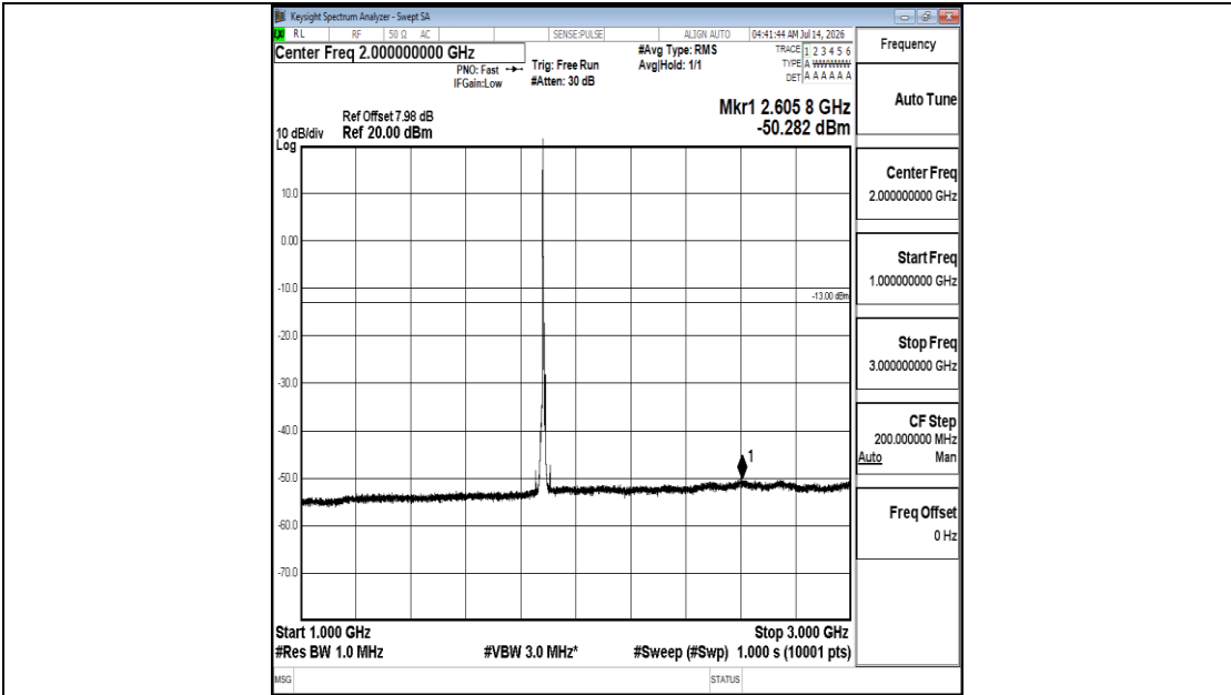
Band25-5MHz-16QAM-26365-1RB#0-1000~3000-PASS
