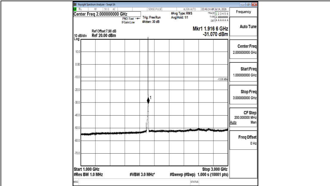
Band25-1.4MHz-16QAM-26683-1RB#0-1000~3000-PASS
