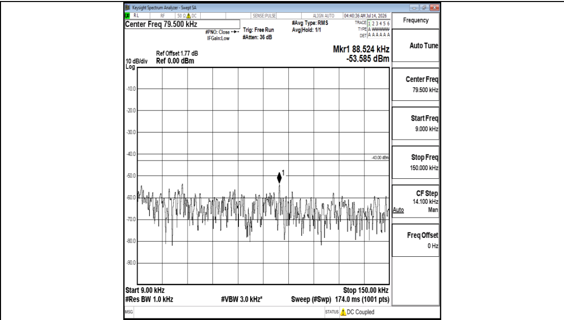
Band25-5MHz-QPSK-26365-1RB#0-0.009~0.15-PASS
