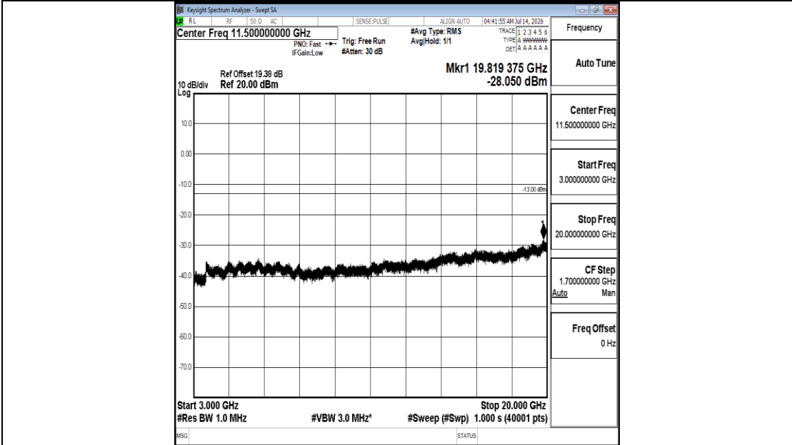
Band25-5MHz-16QAM-26365-1RB#0-3000~20000-PASS
