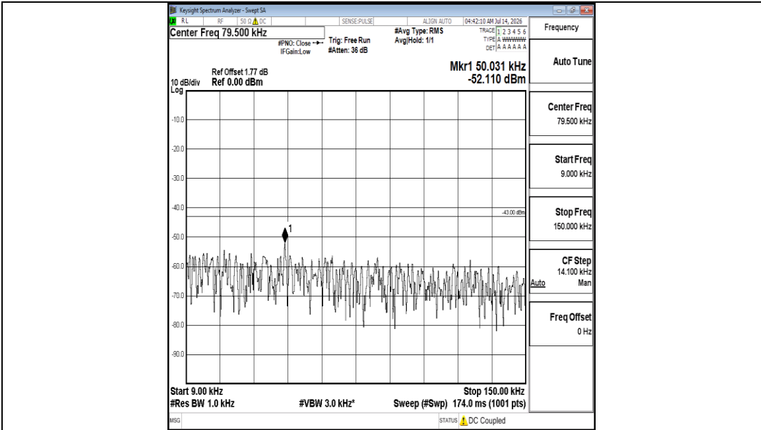
Band25-5MHz-QPSK-26665-1RB#0-0.009~0.15-PASS
