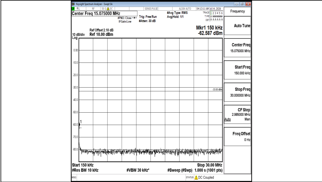
Band25-3MHz-QPSK-26365-1RB#0-0.15~30-PASS
