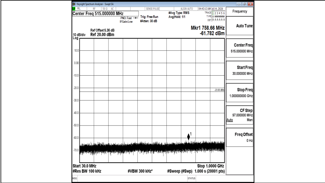
Band25-5MHz-16QAM-26665-1RB#0-30~1000-PASS
