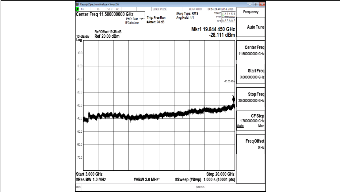
Band25-3MHz-16QAM-26365-1RB#0-3000~20000-PASS
