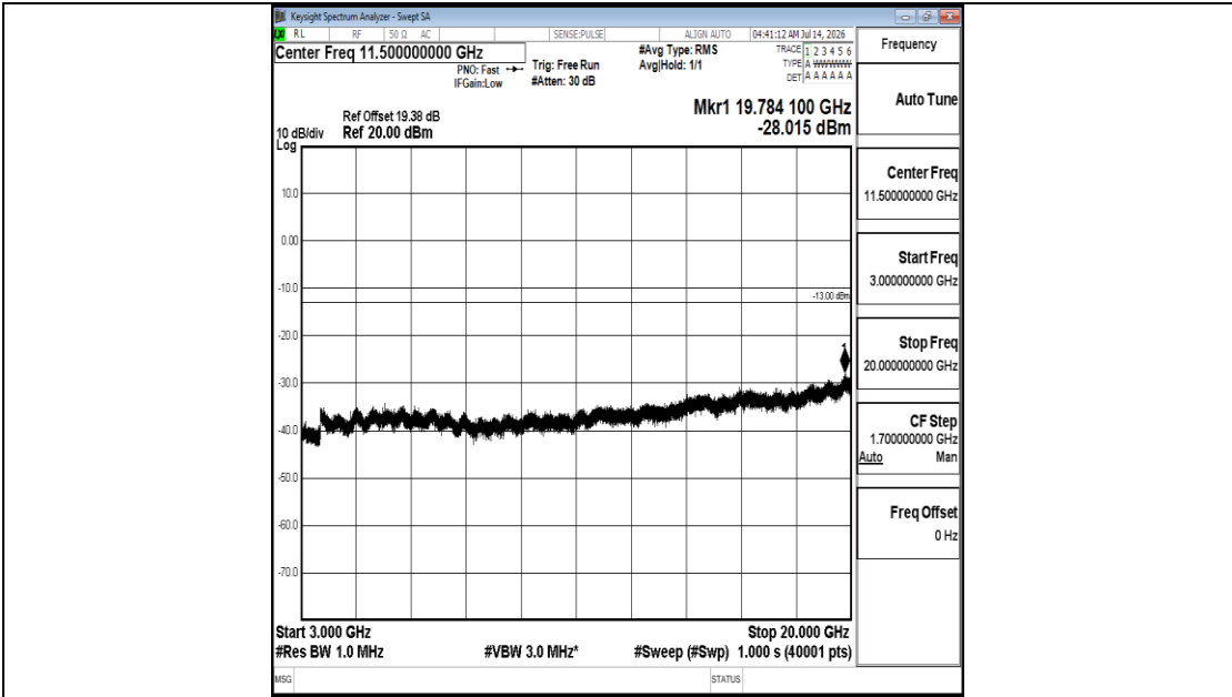
Band25-5MHz-QPSK-26365-1RB#0-3000~20000-PASS
