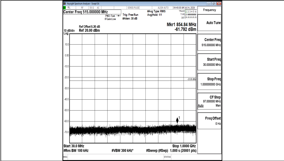
Band25-5MHz-16QAM-26065-1RB#0-30~1000-PASS
