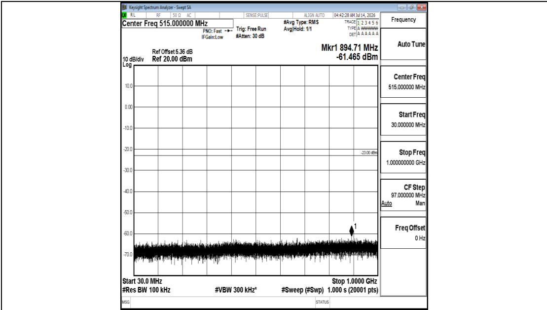
Band25-5MHz-QPSK-26665-1RB#0-30~1000-PASS
