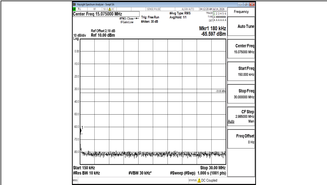
Band25-3MHz-16QAM-26055-1RB#0-0.15~30-PASS
