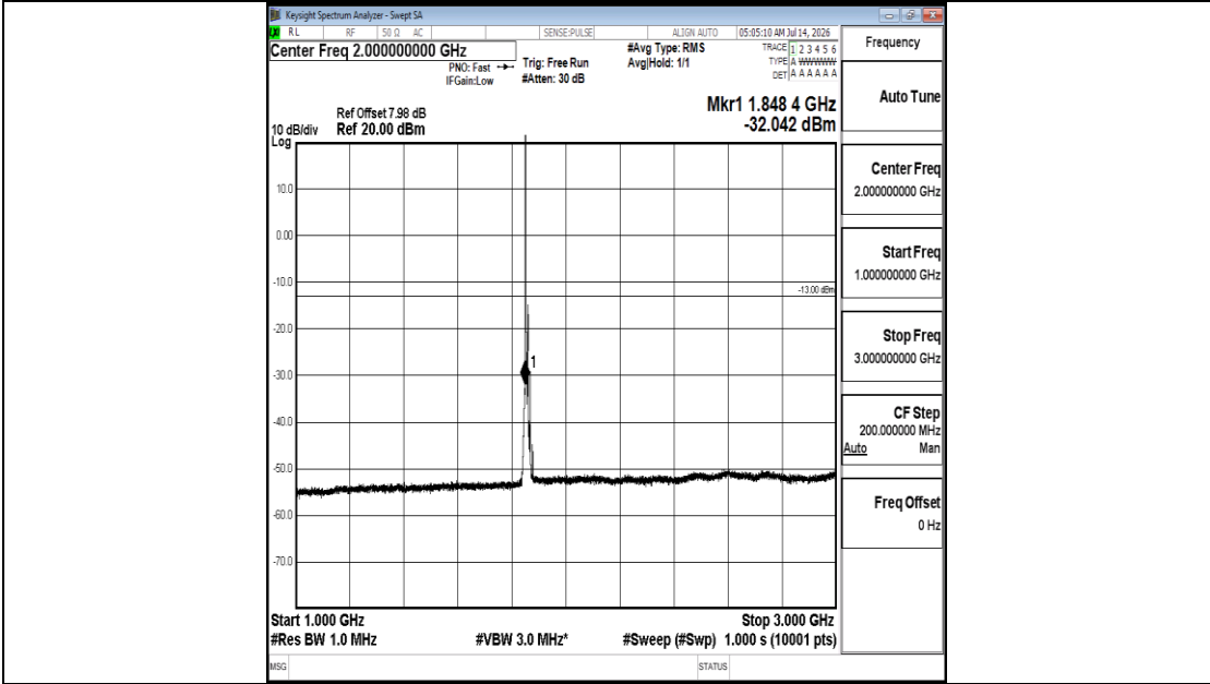
Band25-10MHz-QPSK-26090-1RB#0-1000~3000-PASS
