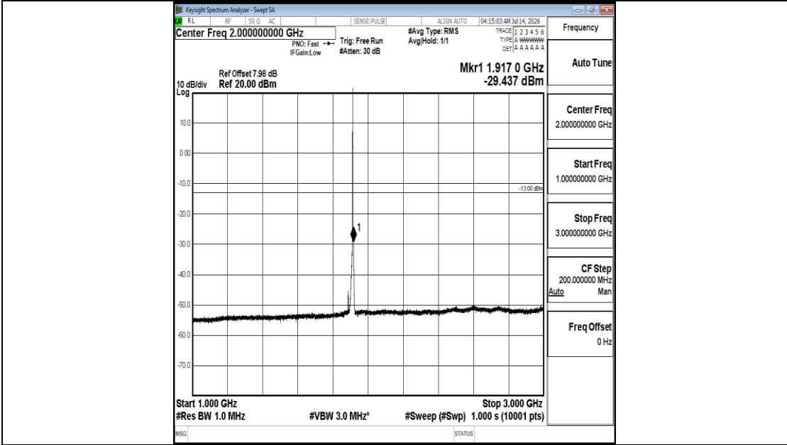
Band25-3MHz-QPSK-26675-1RB#0-1000~3000-PASS
