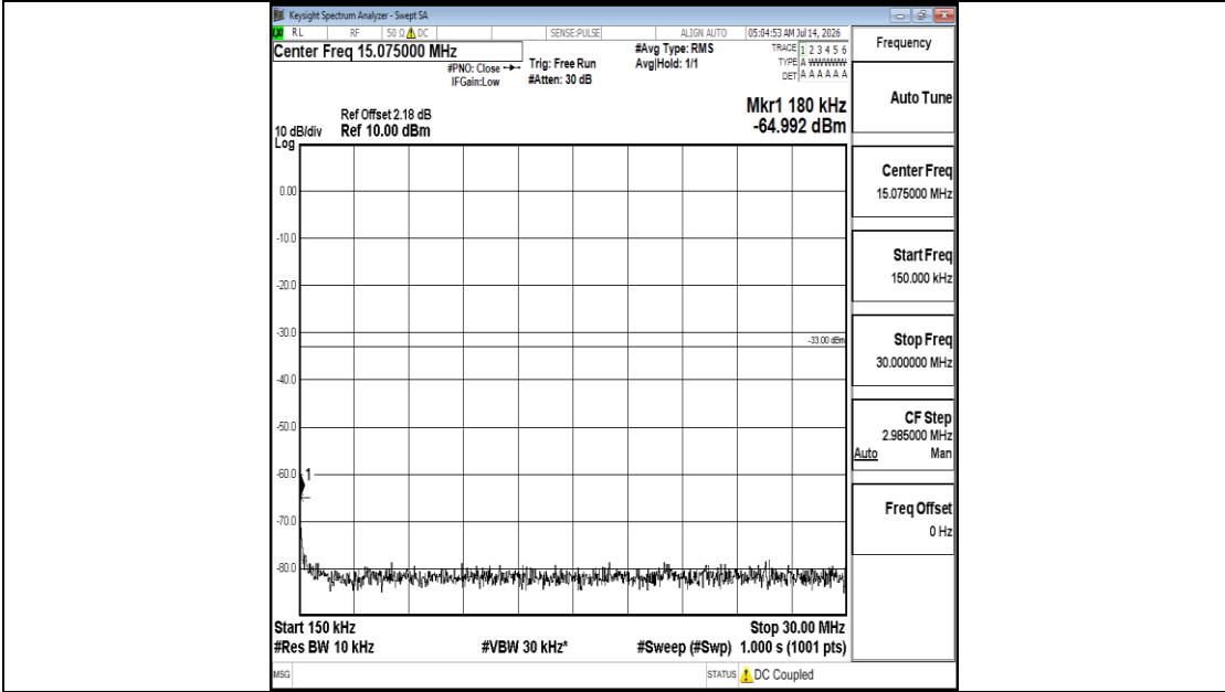
Band25-10MHz-QPSK-26090-1RB#0-0.15~30-PASS
