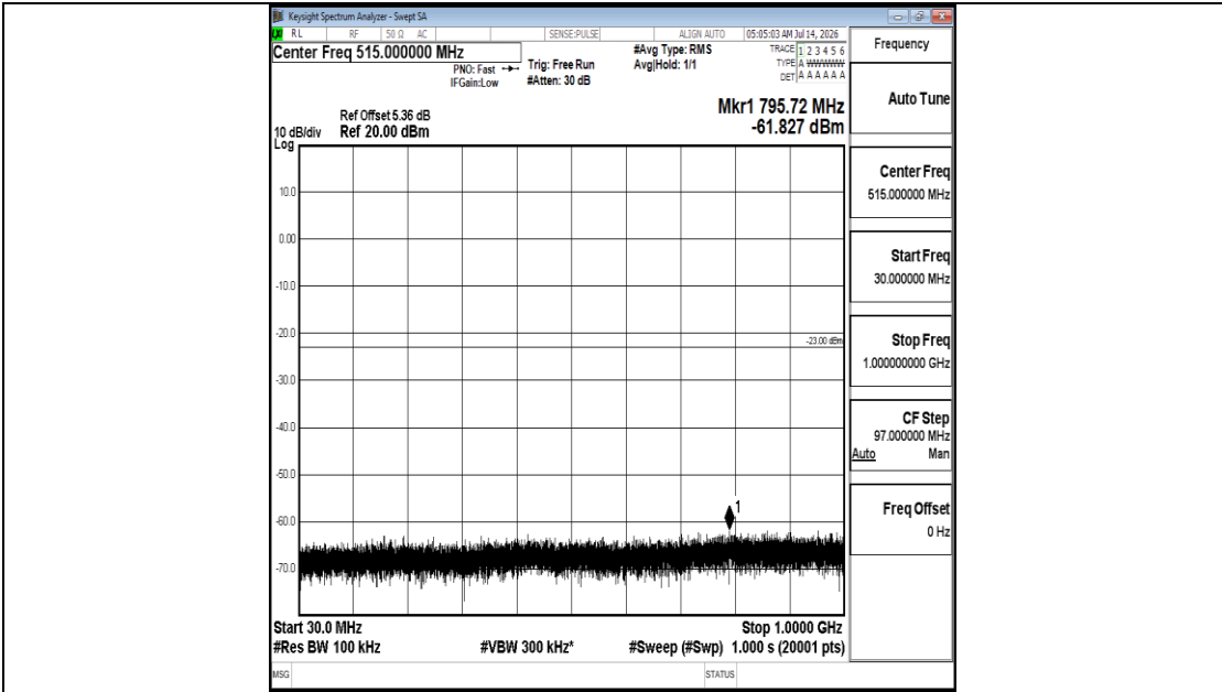
Band25-10MHz-QPSK-26090-1RB#0-30~1000-PASS
