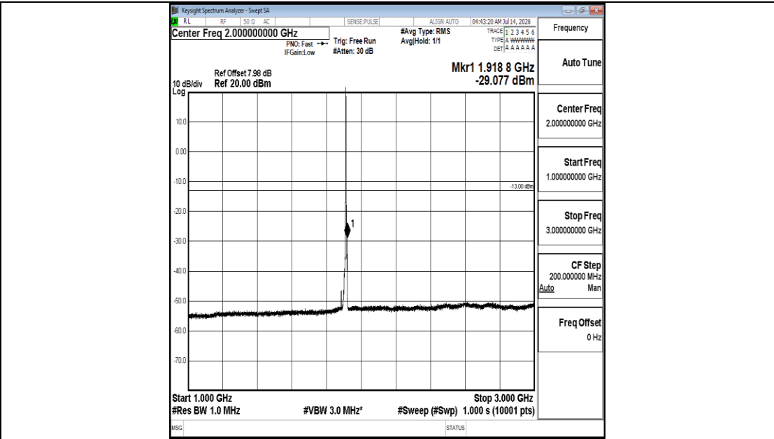
Band25-5MHz-16QAM-26665-1RB#0-1000~3000-PASS
