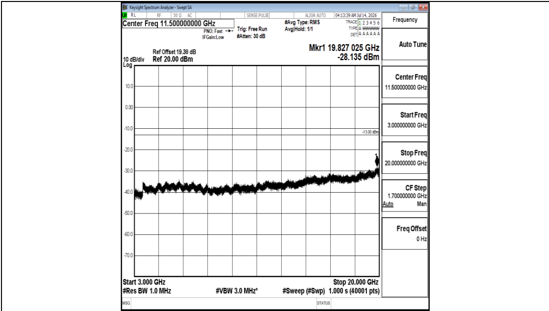
Band25-3MHz-QPSK-26365-1RB#0-3000~20000-PASS
