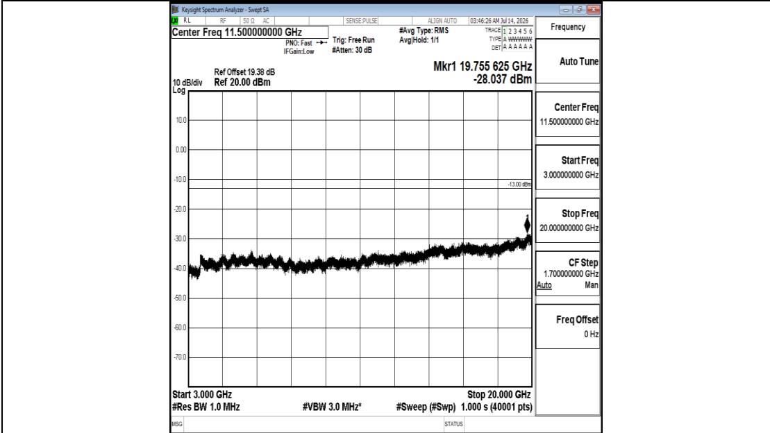
Band25-1.4MHz-16QAM-26683-1RB#0-3000~20000-PASS
