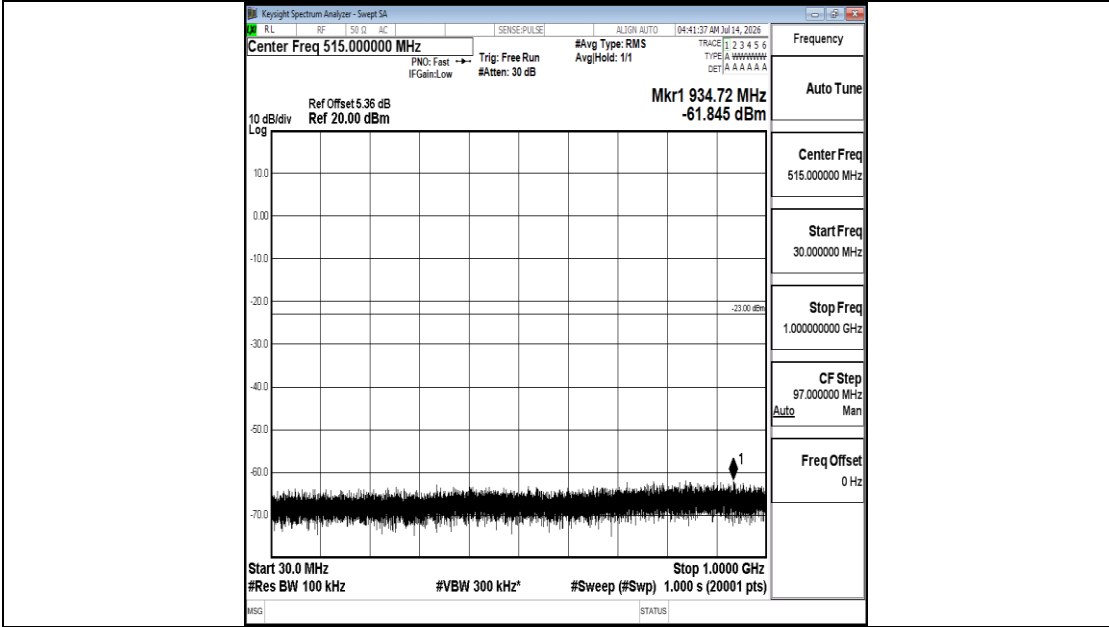
Band25-5MHz-16QAM-26365-1RB#0-30~1000-PASS
