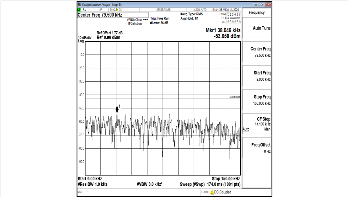
Band25-3MHz-QPSK-26675-1RB#0-0.009~0.15-PASS
