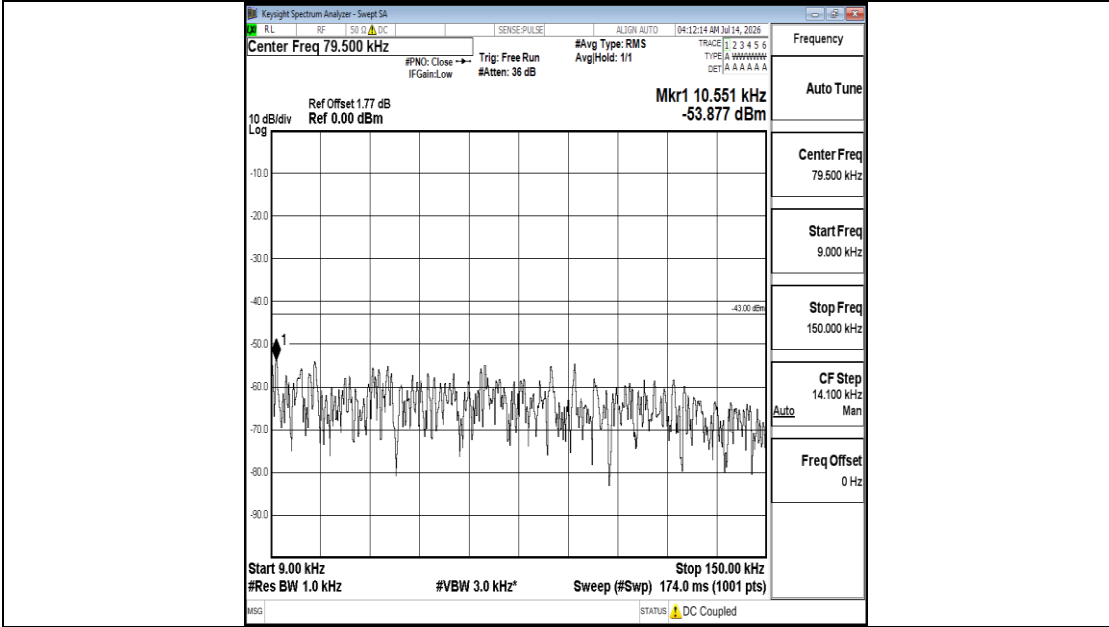
Band25-3MHz-16QAM-26055-1RB#0-0.009~0.15-PASS
