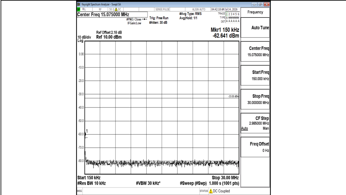
Band25-5MHz-QPSK-26665-1RB#0-0.15~30-PASS
