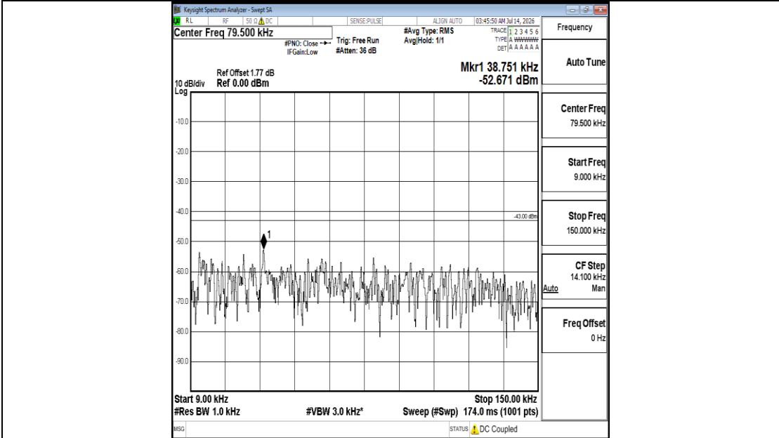
Band25-1.4MHz-16QAM-26683-1RB#0-0.009~0.15-PASS
