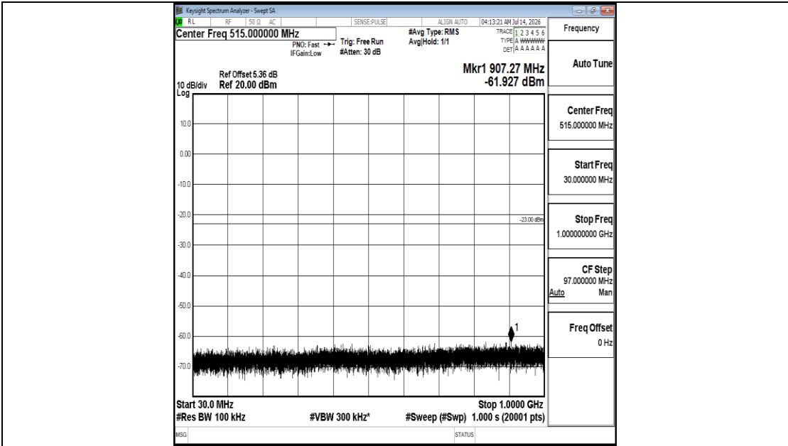
Band25-3MHz-QPSK-26365-1RB#0-30~1000-PASS
