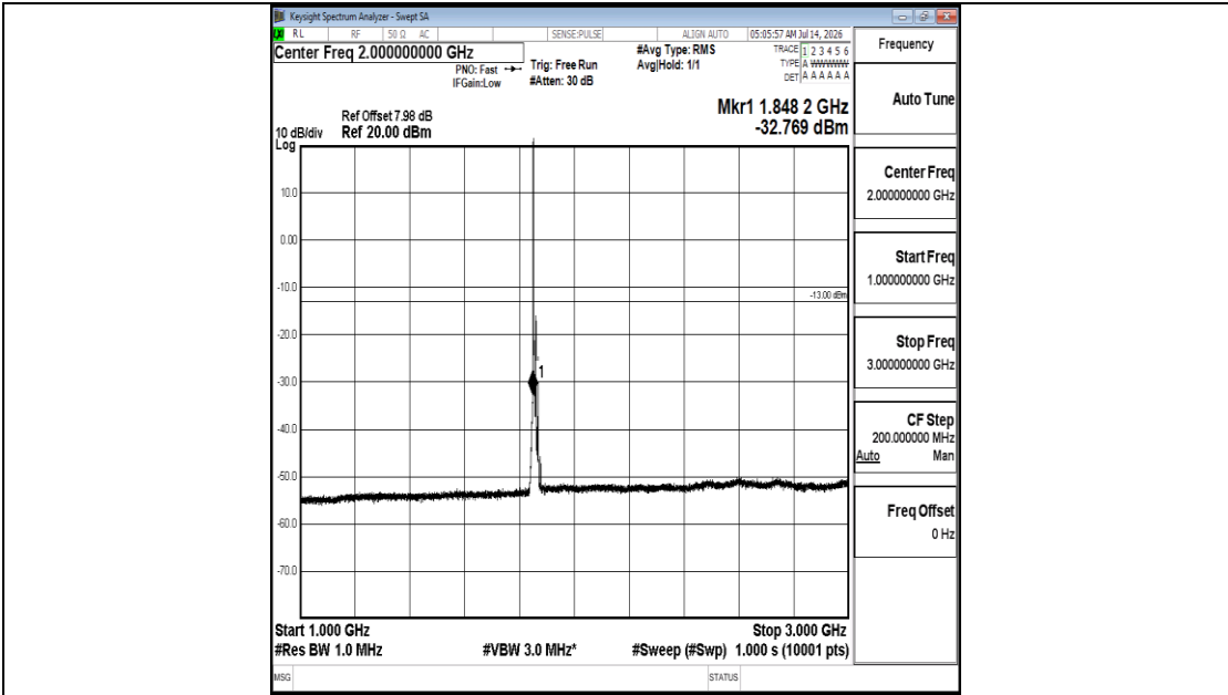
Band25-10MHz-16QAM-26090-1RB#0-1000~3000-PASS
