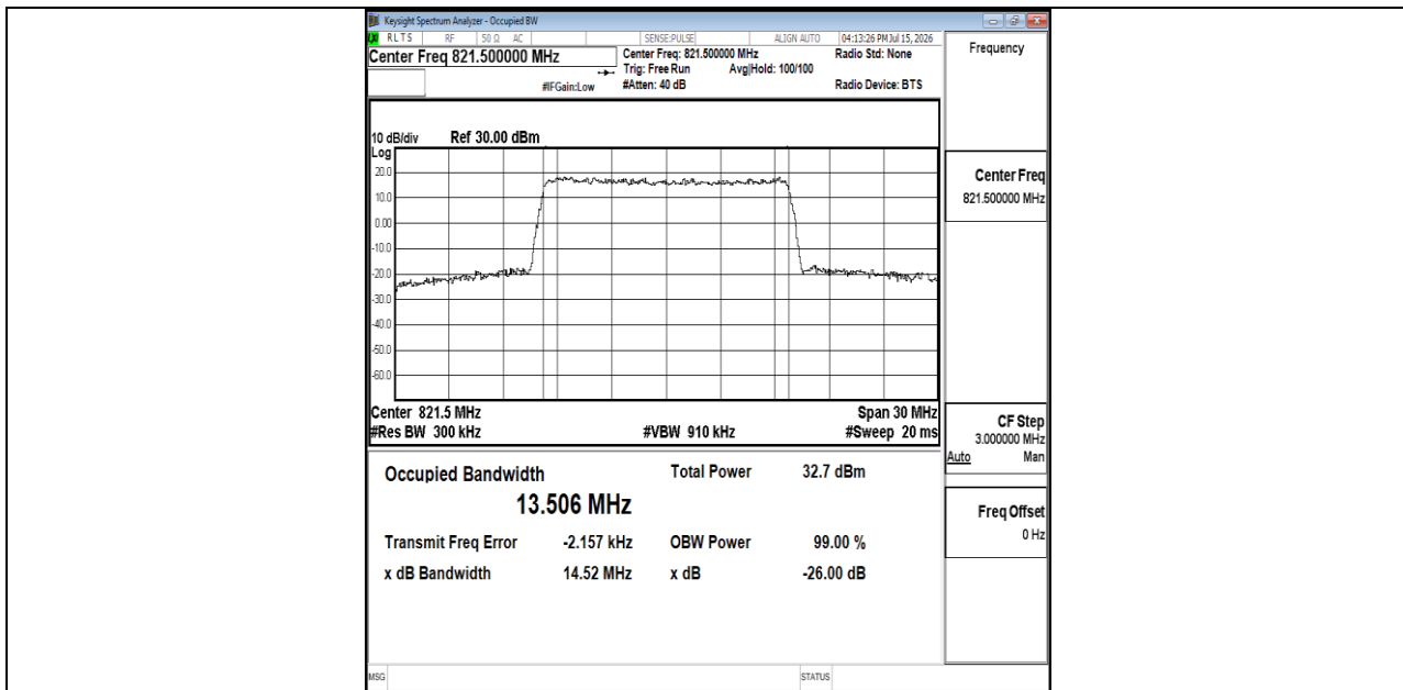
Band26(814-824)-15MHz-QPSK-26765-75RB#0-PASS
