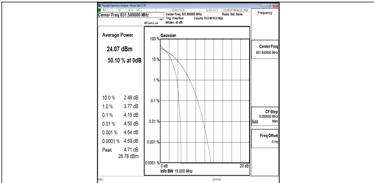
Band26(824-849)-15MHz-QPSK-26865-1RB#0-PASS
