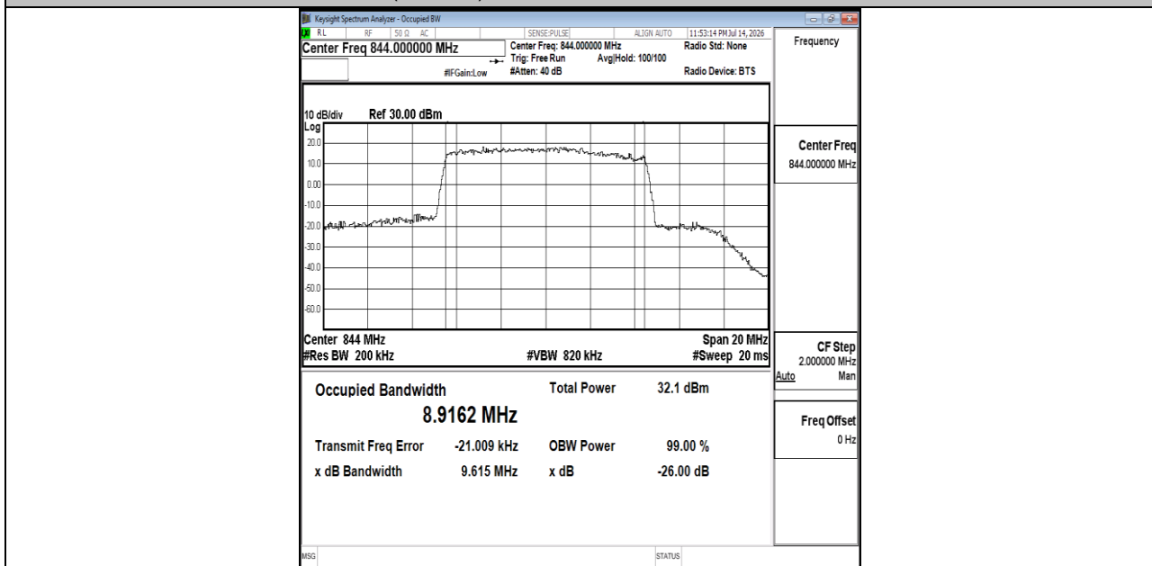
Band26(824-849)-10MHz-16QAM-26990-50RB#0-PASS
