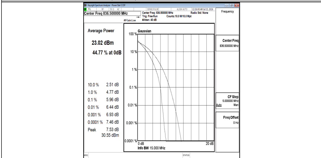
Band26(824-849)-15MHz-QPSK-26915-75RB#0-PASS
