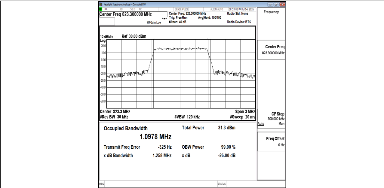
Band26(814-824)-1.4MHz-QPSK-26783-6RB#0-PASS
