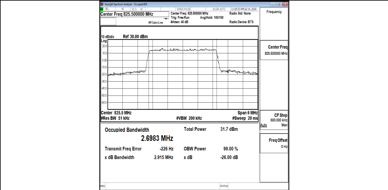
Band26(824-849)-3MHz-16QAM-26805-15RB#0-PASS
