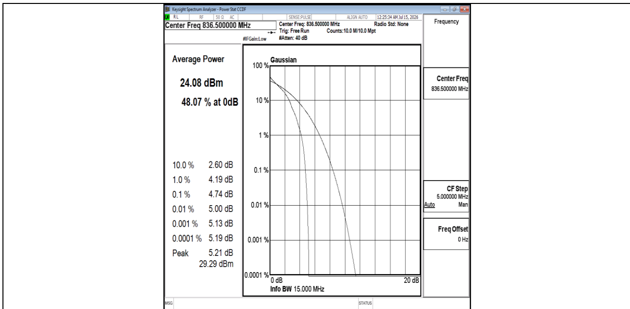
Band26(824-849)-15MHz-QPSK-26915-1RB#0-PASS
