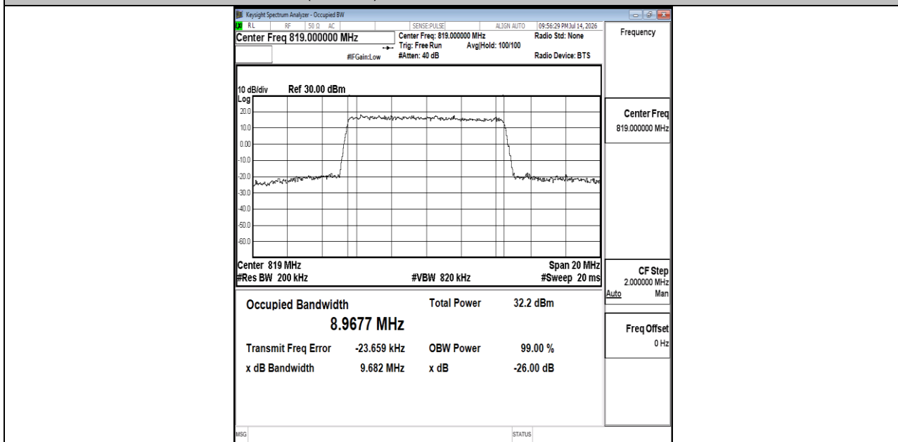
Band26(814-824)-10MHz-16QAM-26740-50RB#0-PASS
