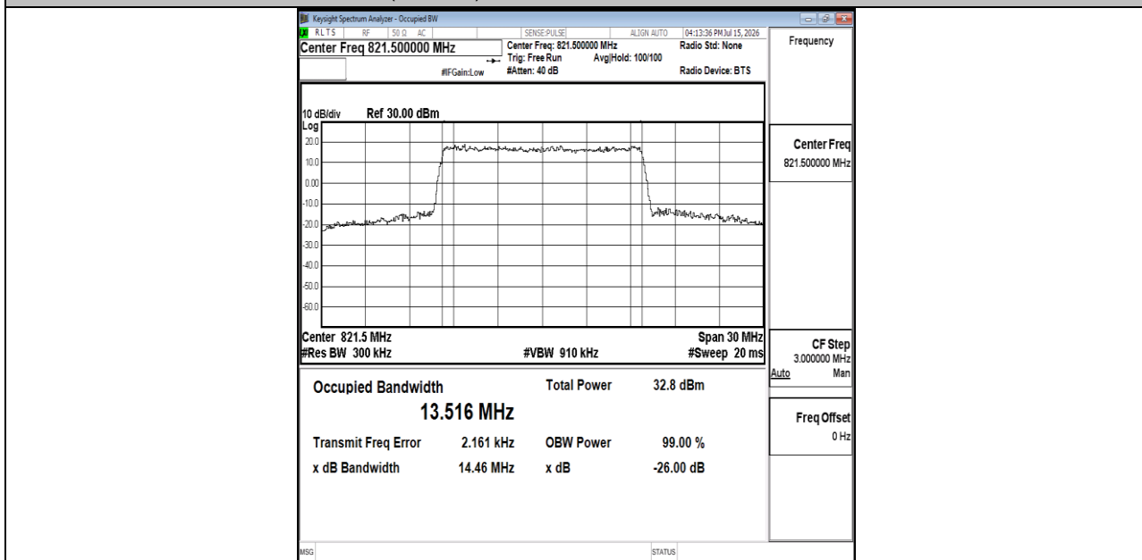
Band26(814-824)-15MHz-16QAM-26765-75RB#0-PASS
