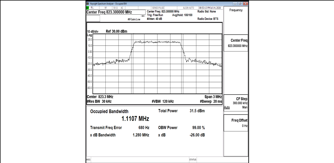
Band26(814-824)-1.4MHz-16QAM-26783-6RB#0-PASS
