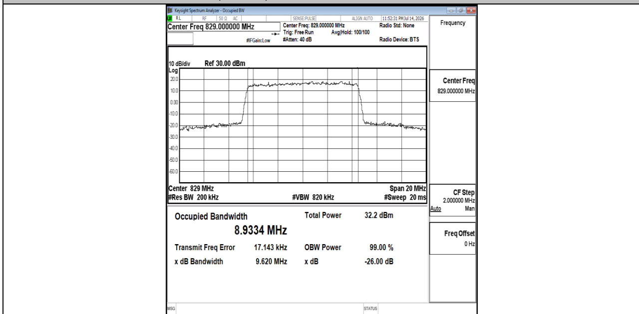
Band26(824-849)-10MHz-16QAM-26840-50RB#0-PASS
