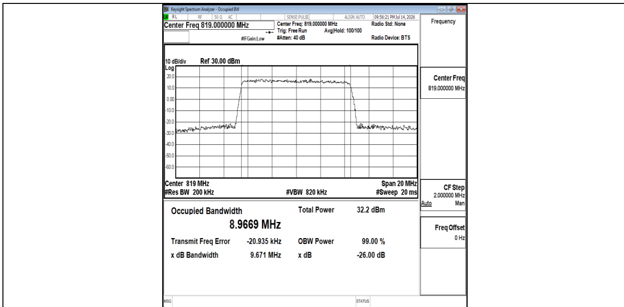
Band26(814-824)-10MHz-QPSK-26740-50RB#0-PASS
