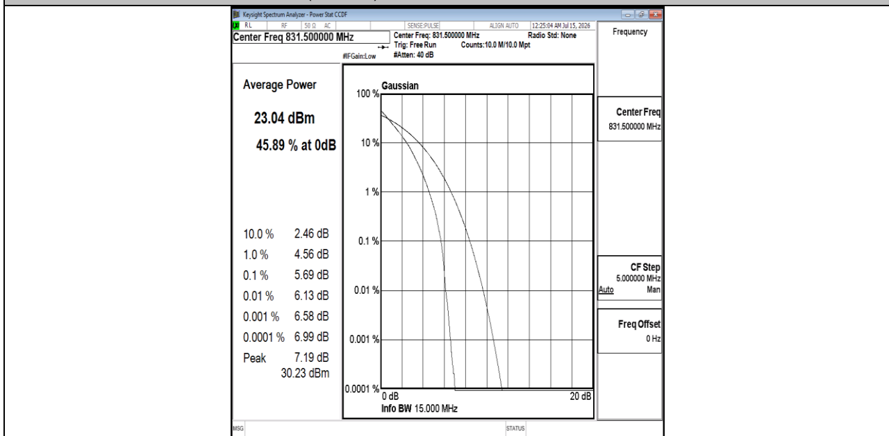
Band26(824-849)-15MHz-QPSK-26865-75RB#0-PASS
