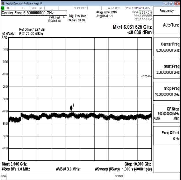
Band26(814-824)-3MHz-16QAM-26775-1RB#0-3000~10000-PASS
