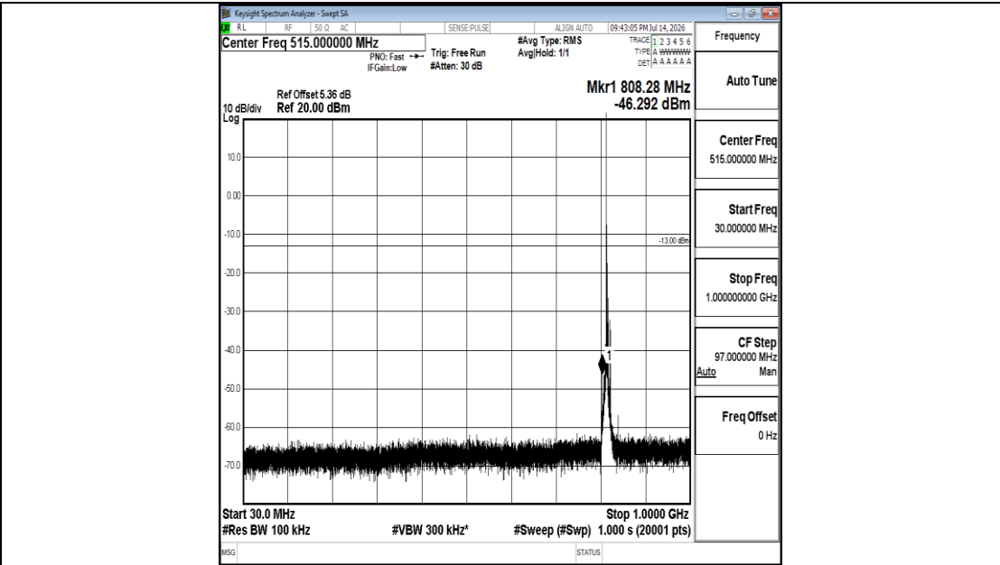
Band26(814-824)-5MHz-QPSK-26740-1RB#0-30~1000-PASS
