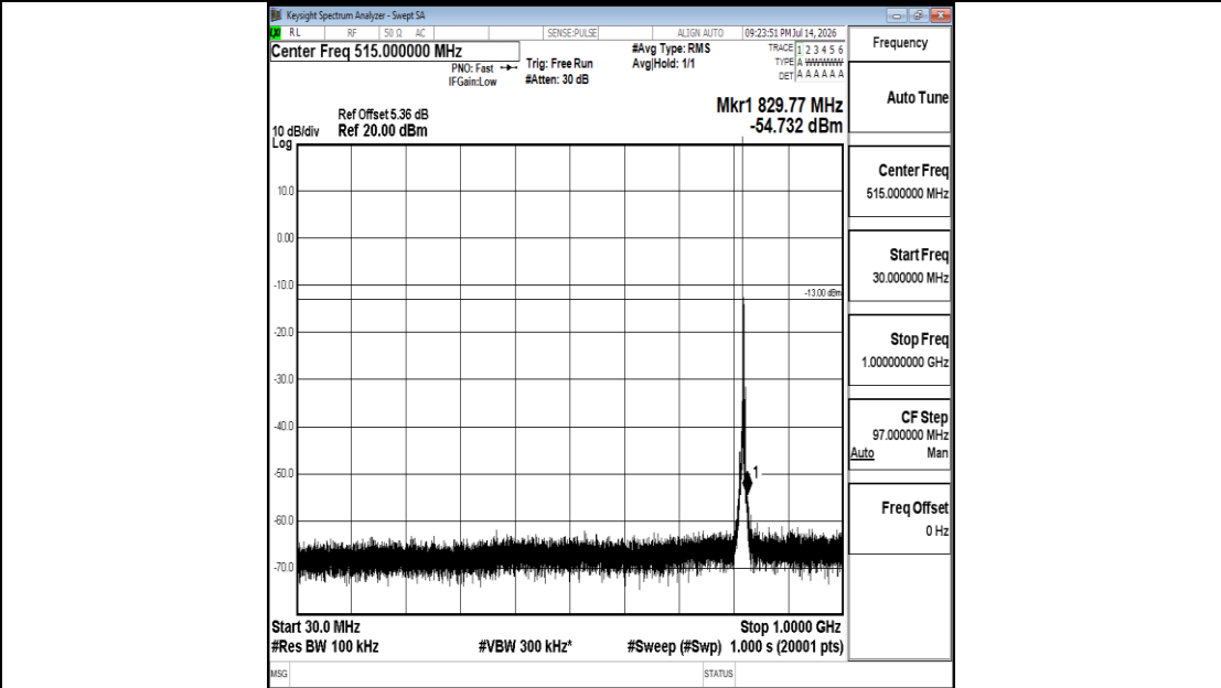
Band26(814-824)-3MHz-16QAM-26775-1RB#0-30~1000-PASS
