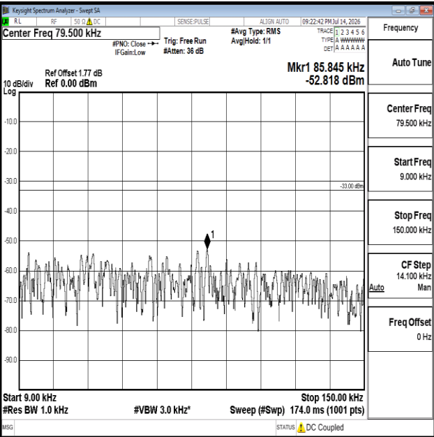
Band26(814-824)-3MHz-QPSK-26775-1RB#0-0.009~0.15-PASS
