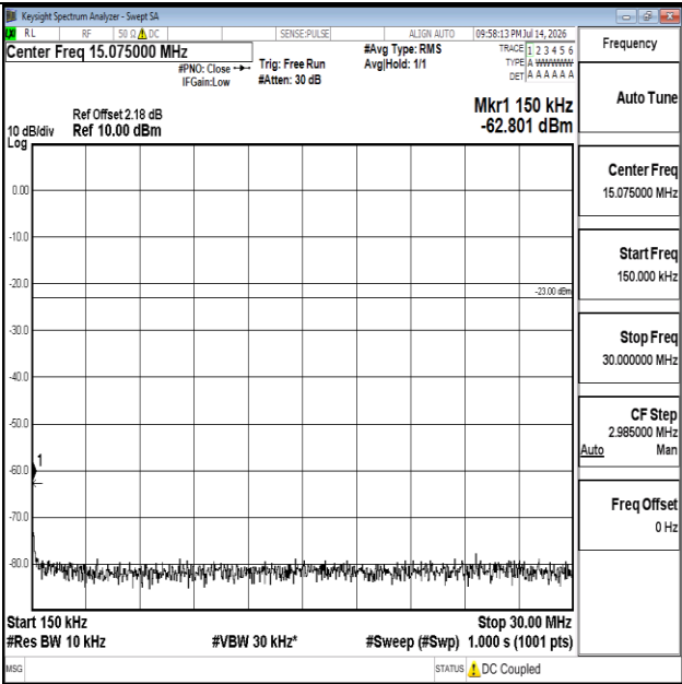
Band26(814-824)-10MHz-16QAM-26740-1RB#0-0.15~30-PASS
