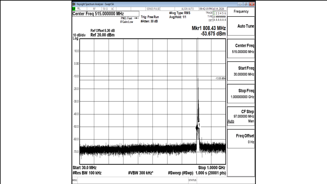
Band26(814-824)-5MHz-16QAM-26715-1RB#0-30~1000-PASS
