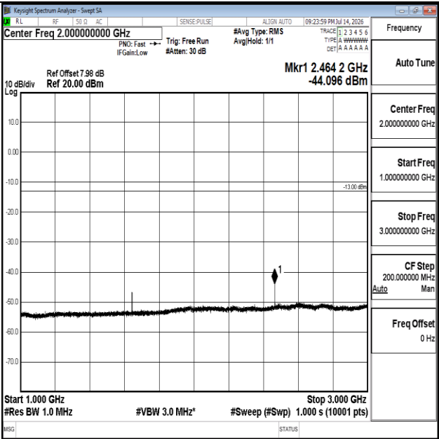
Band26(814-824)-3MHz-16QAM-26775-1RB#0-1000~3000-PASS
