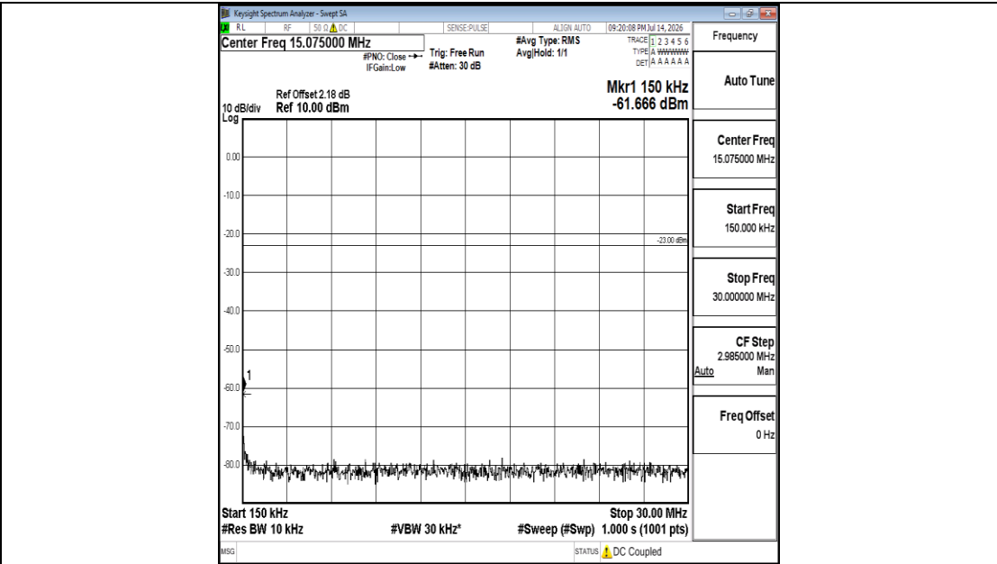
Band26(814-824)-3MHz-16QAM-26705-1RB#0-0.15~30-PASS
