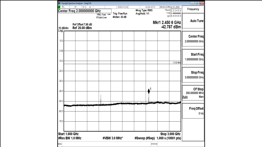
Band26(814-824)-5MHz-QPSK-26740-1RB#0-1000~3000-PASS
