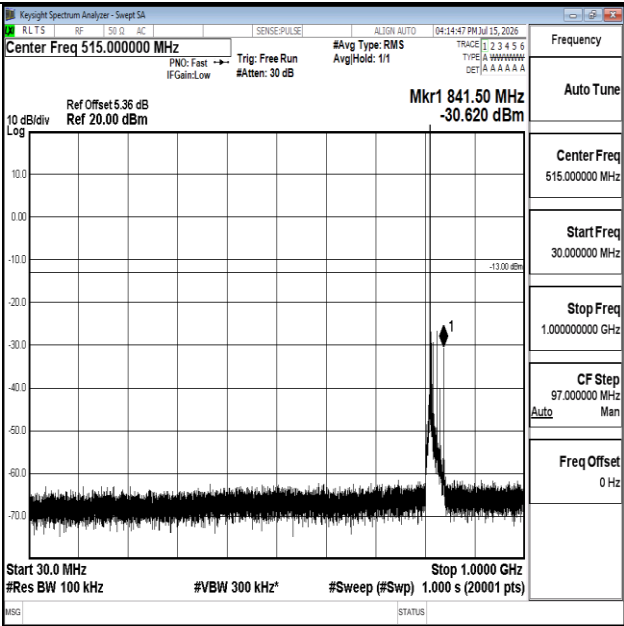
Band26(814-824)-15MHz-QPSK-26765-1RB#0-30~1000-PASS
