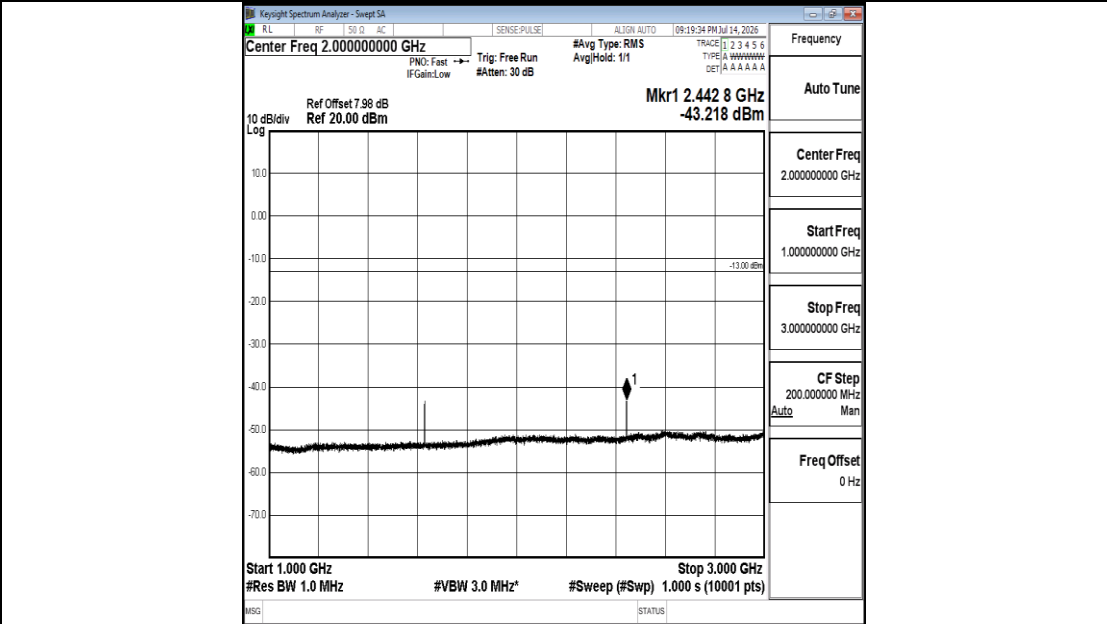
Band26(814-824)-3MHz-QPSK-26705-1RB#0-1000~3000-PASS
