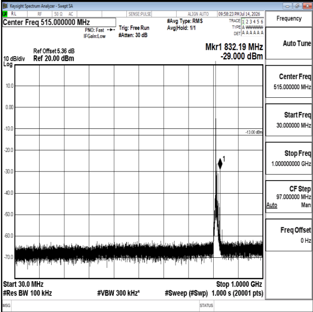
Band26(814-824)-10MHz-16QAM-26740-1RB#0-30~1000-PASS
