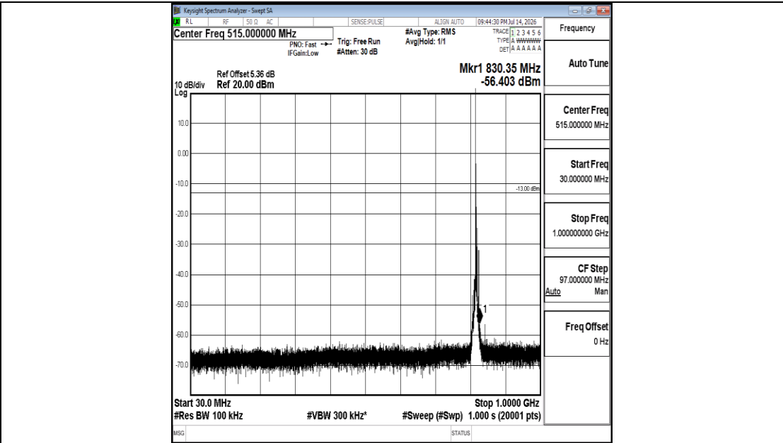
Band26(814-824)-5MHz-QPSK-26765-1RB#0-30~1000-PASS
