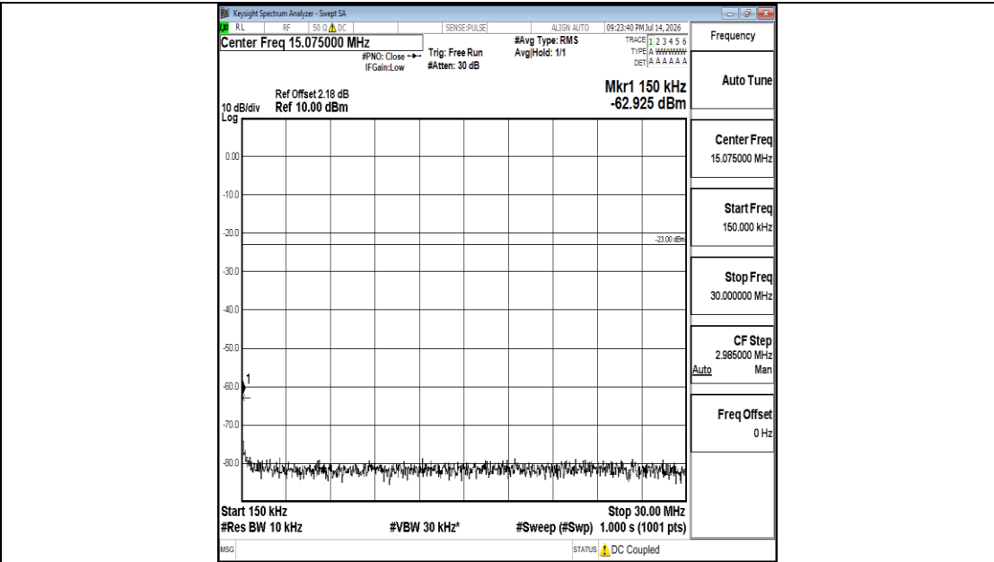
Band26(814-824)-3MHz-16QAM-26775-1RB#0-0.15~30-PASS
