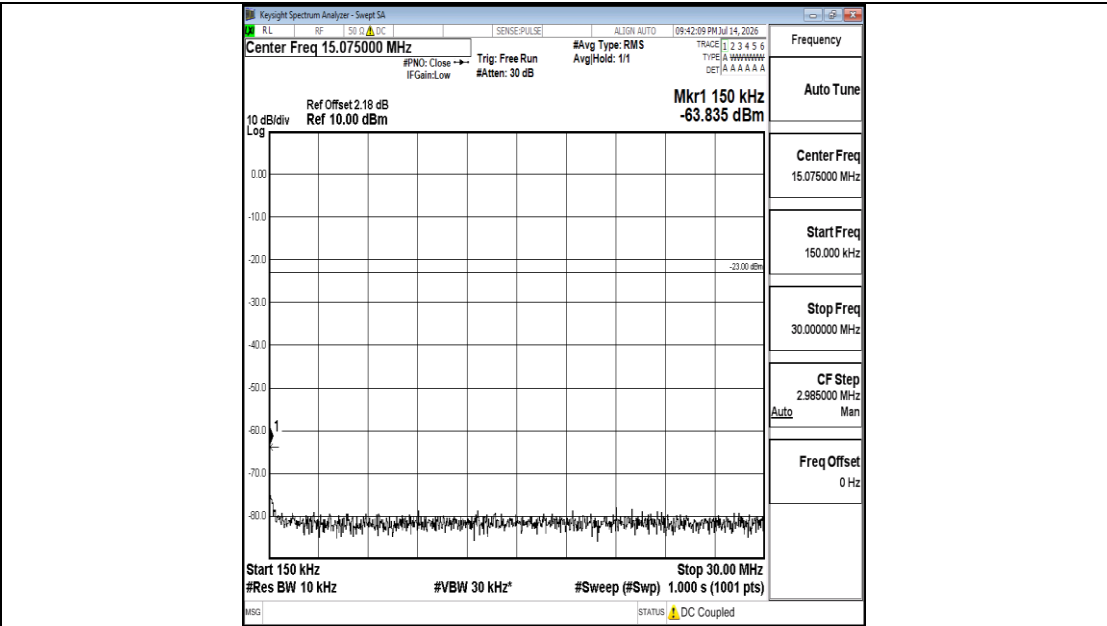
Band26(814-824)-5MHz-16QAM-26715-1RB#0-0.15~30-PASS
