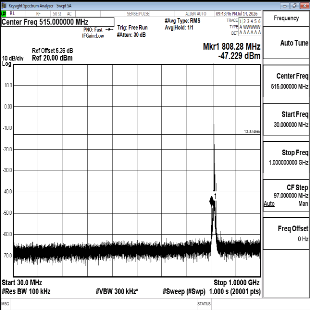
Band26(814-824)-5MHz-16QAM-26740-1RB#0-30~1000-PASS
