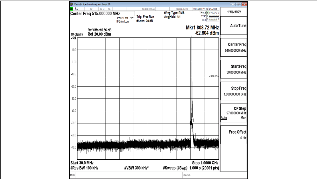
Band26(814-824)-3MHz-QPSK-26705-1RB#0-30~1000-PASS
