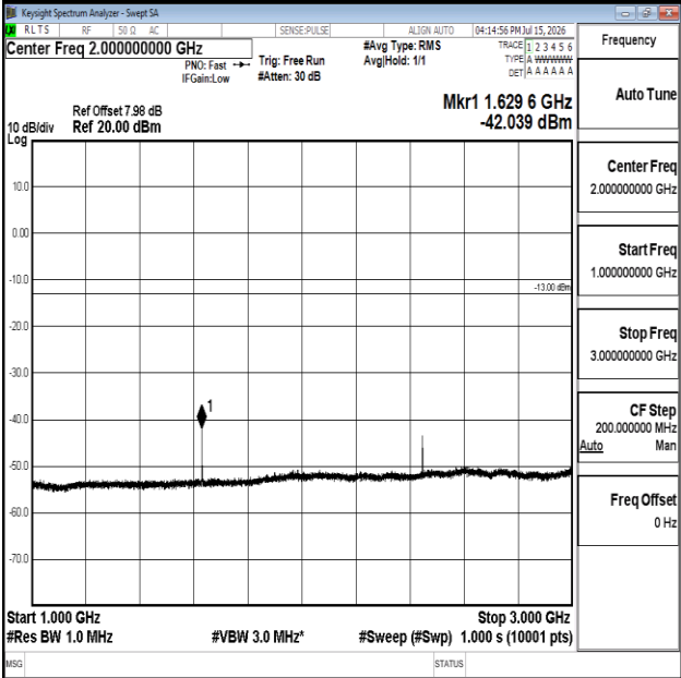
Band26(814-824)-15MHz-QPSK-26765-1RB#0-1000~3000-PASS
