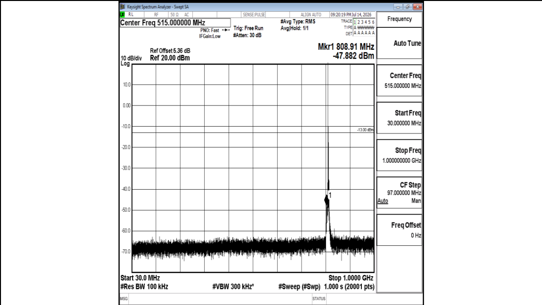
Band26(814-824)-3MHz-16QAM-26705-1RB#0-30~1000-PASS
