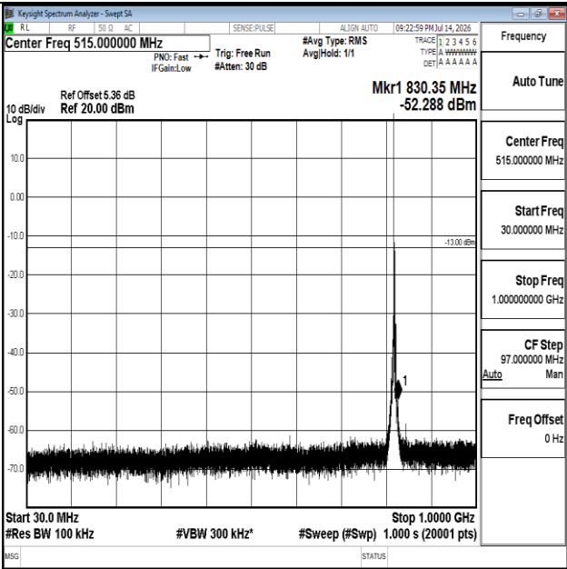
Band26(814-824)-3MHz-QPSK-26775-1RB#0-30~1000-PASS
