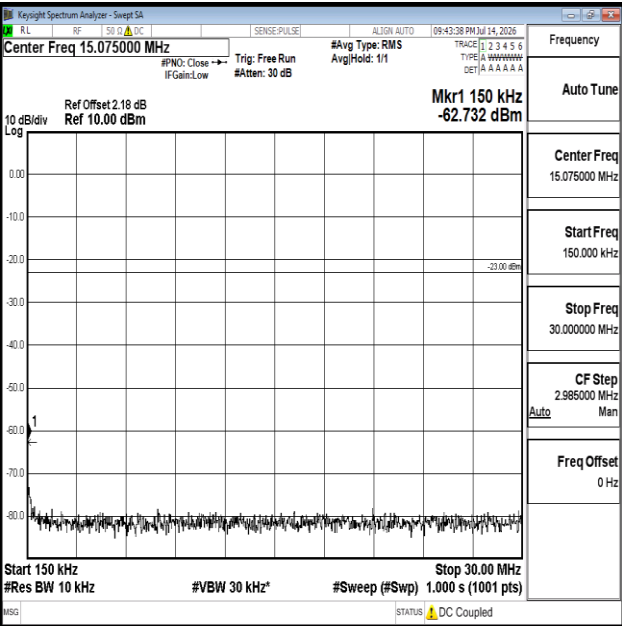
Band26(814-824)-5MHz-16QAM-26740-1RB#0-0.15~30-PASS
