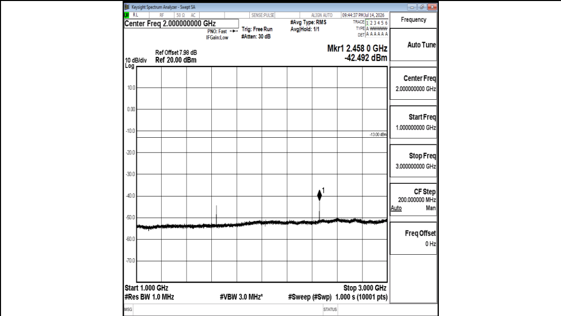
Band26(814-824)-5MHz-QPSK-26765-1RB#0-1000~3000-PASS
