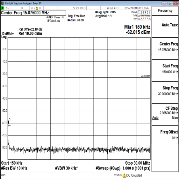
Band26(814-824)-3MHz-QPSK-26775-1RB#0-0.15~30-PASS
