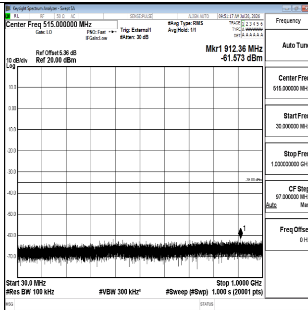
Band41-5MHz-16QAM-40620-1RB#0-30~1000-PASS
