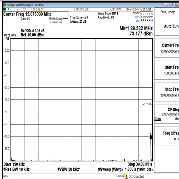
Band41-5MHz-QPSK-40620-1RB#0-0.15~30-PASS
