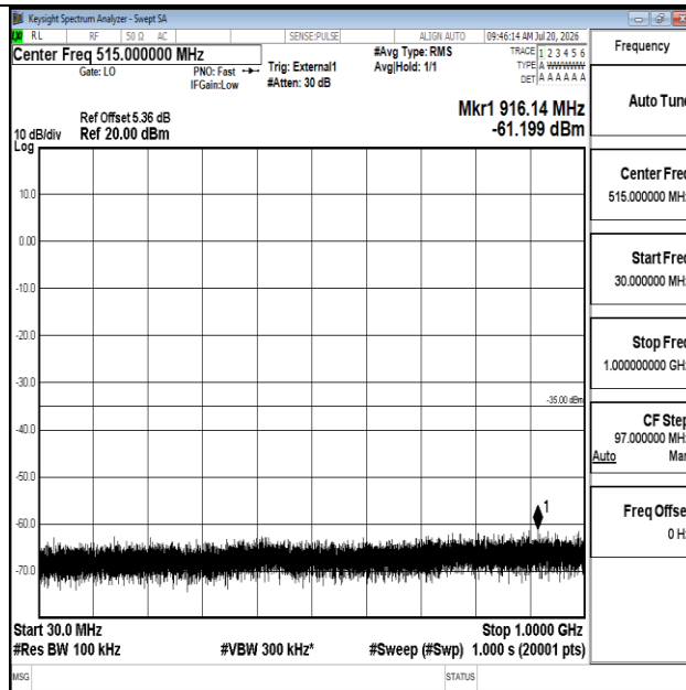
Band41-5MHz-16QAM-39675-1RB#0-30~1000-PASS
