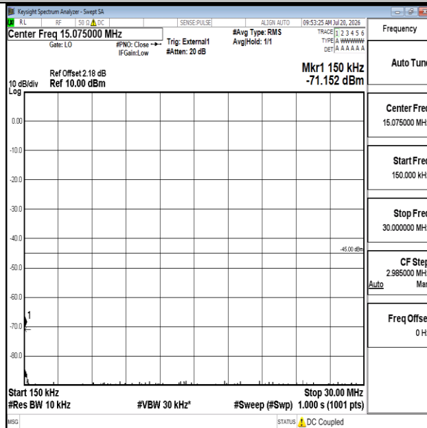
Band41-5MHz-QPSK-41565-1RB#0-0.15~30-PASS
