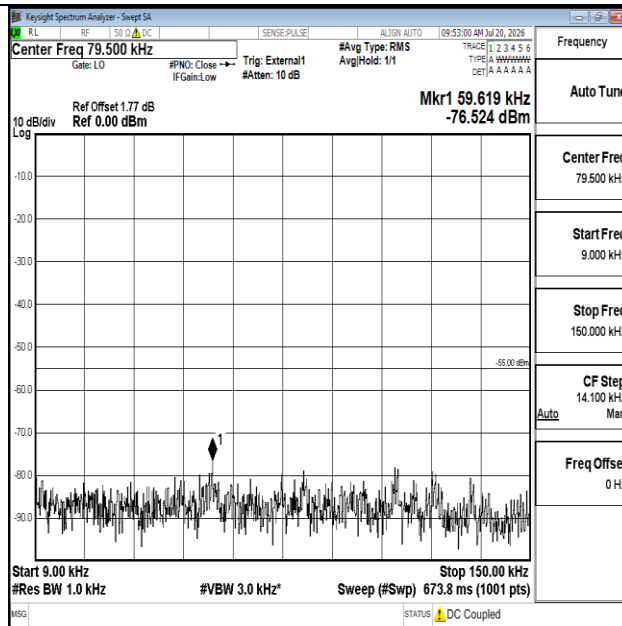
Band41-5MHz-QPSK-41565-1RB#0-0.009~0.15-PASS
