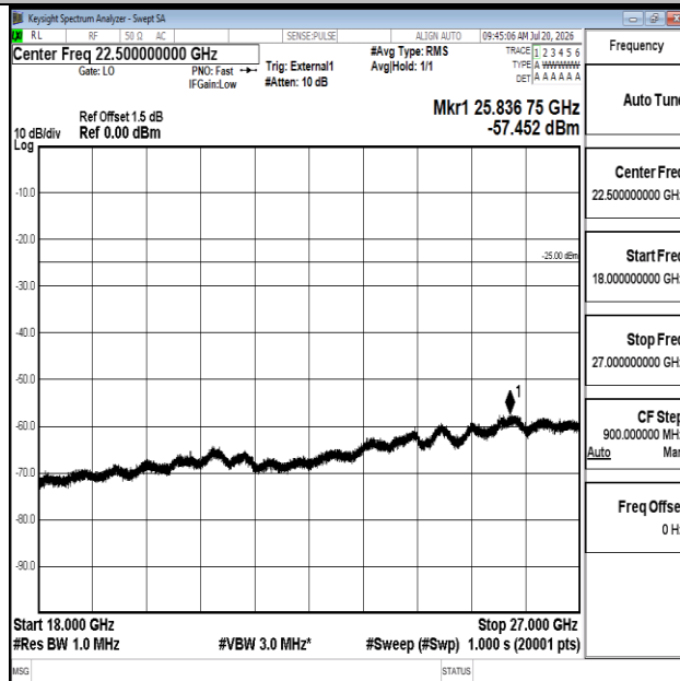
Band41-5MHz-QPSK-39675-1RB#0-18000~27000-PASS
