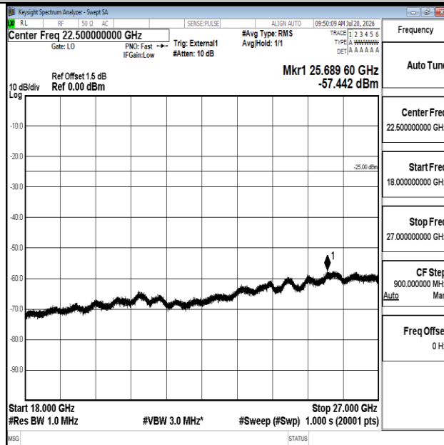
Band41-5MHz-QPSK-40620-1RB#0-18000~27000-PASS
