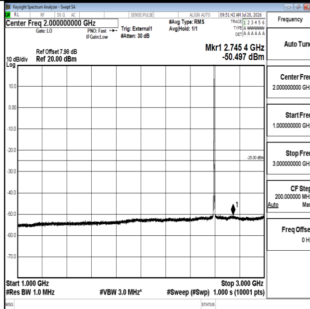
Band41-5MHz-16QAM-40620-1RB#0-1000~3000-PASS
