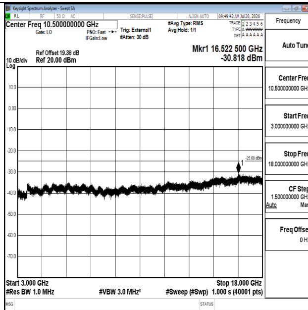
Band41-5MHz-QPSK-40620-1RB#0-3000~18000-PASS
