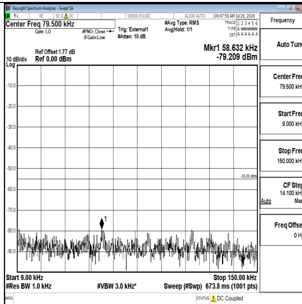
Band41-5MHz-QPSK-40620-1RB#0-0.009~0.15-PASS
