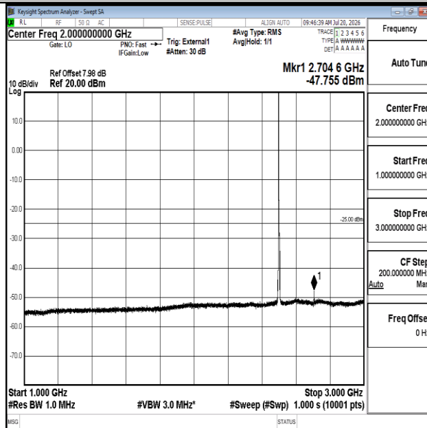
Band41-5MHz-16QAM-39675-1RB#0-1000~3000-PASS
