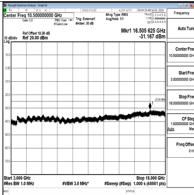
Band41-5MHz-QPSK-39675-1RB#0-3000~18000-PASS
