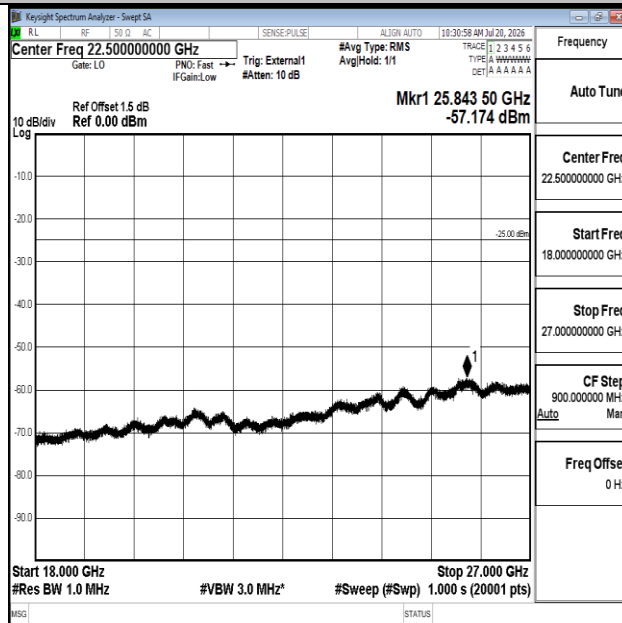
Band41-20MHz-QPSK-39750-1RB#0-18000~27000-PASS
