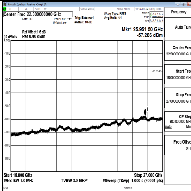
Band41-20MHz-QPSK-40620-1RB#0-18000~27000-PASS
