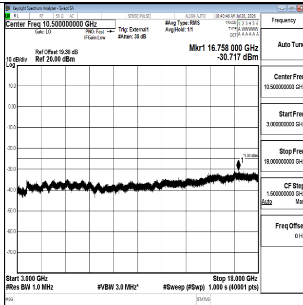
Band41-20MHz-QPSK-41490-1RB#0-3000~18000-PASS
