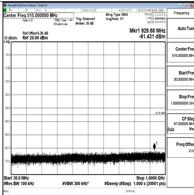
Band41-15MHz-16QAM-40620-1RB#0-30~1000-PASS
