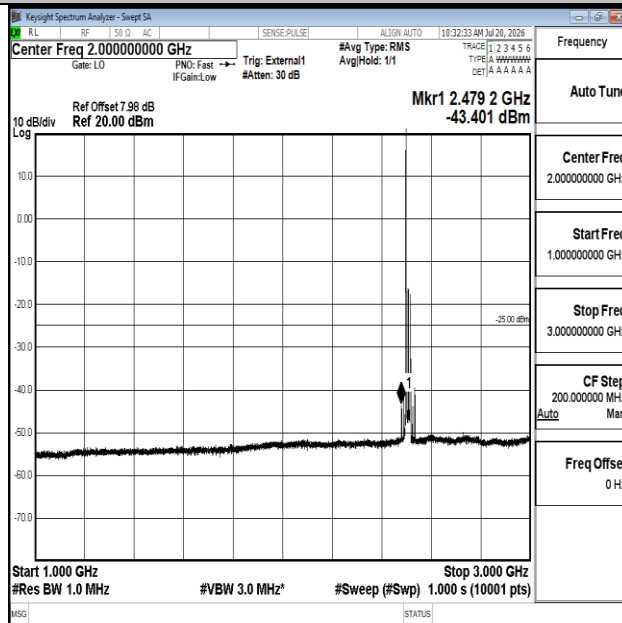
Band41-20MHz-16QAM-39750-1RB#0-1000~3000-PASS
