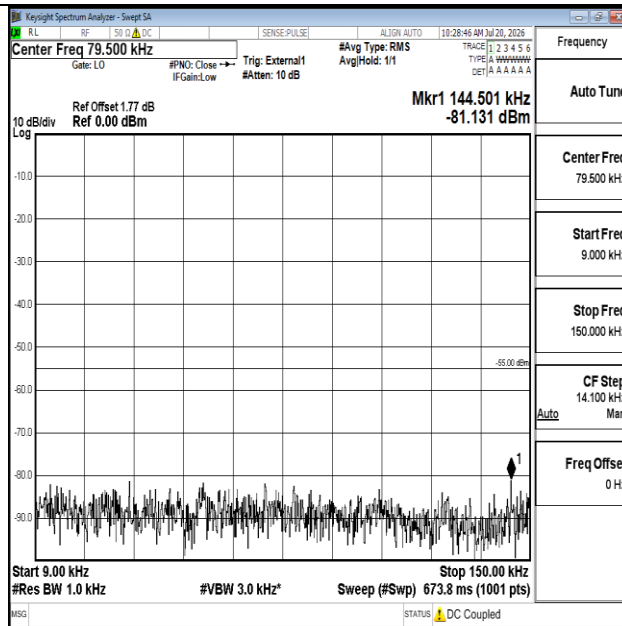
Band41-20MHz-QPSK-39750-1RB#0-0.009~0.15-PASS
