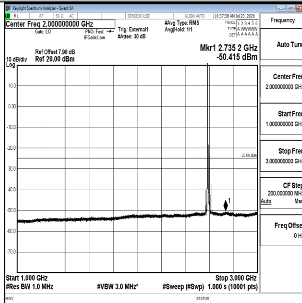
Band41-20MHz-16QAM-40620-1RB#0-1000~3000-PASS
