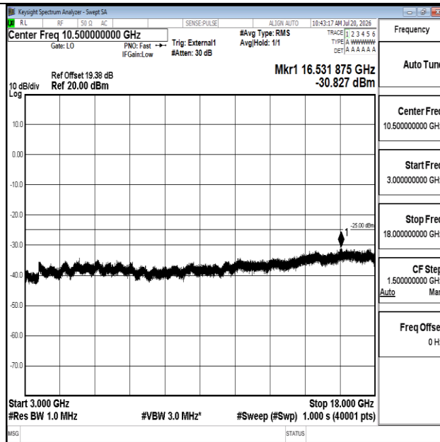
Band41-20MHz-16QAM-41490-1RB#0-3000~18000-PASS
