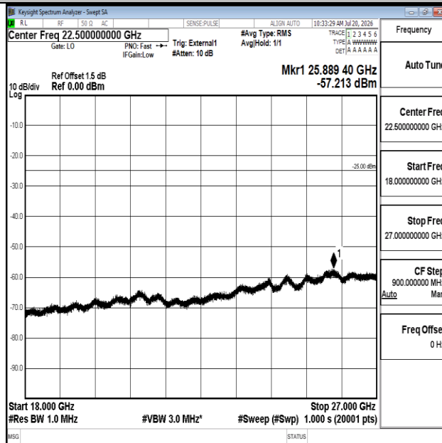
Band41-20MHz-16QAM-39750-1RB#0-18000~27000-PASS
