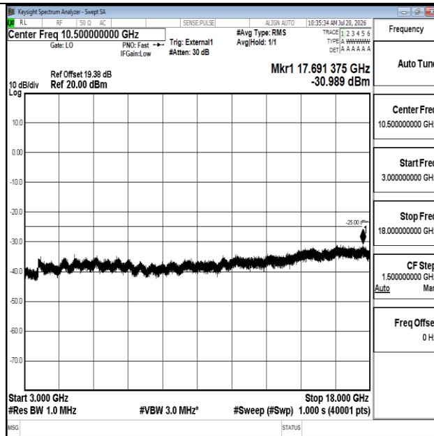
Band41-20MHz-QPSK-40620-1RB#0-3000~18000-PASS
