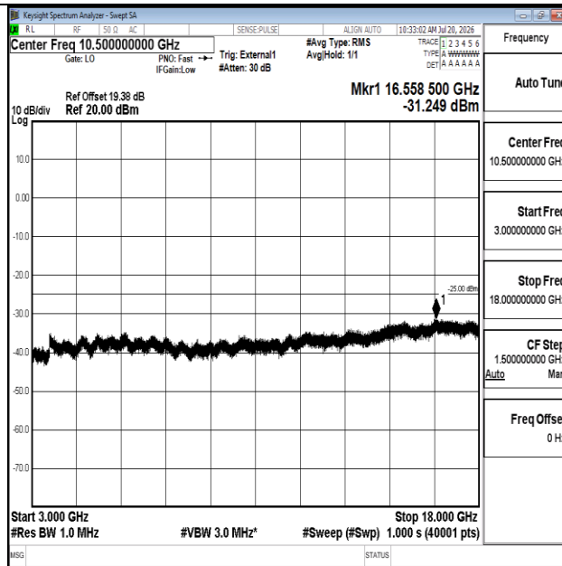
Band41-20MHz-16QAM-39750-1RB#0-3000~18000-PASS
