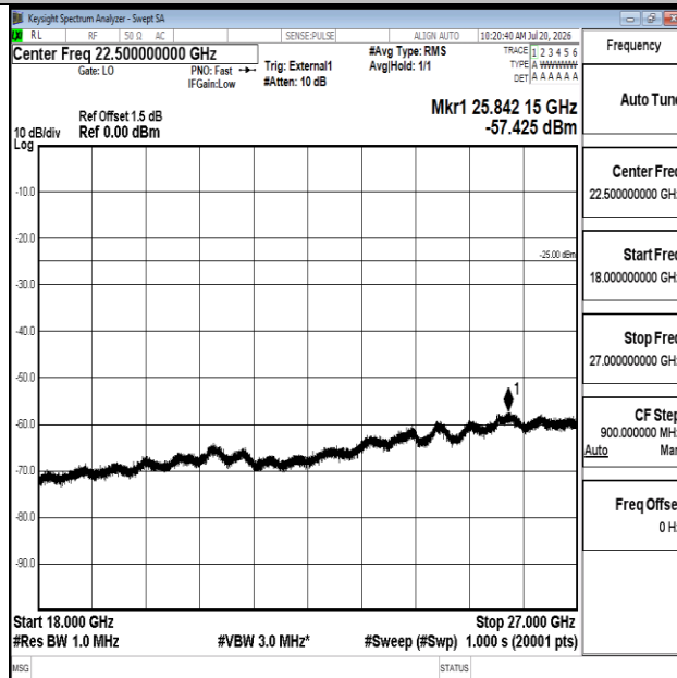
Band41-15MHz-QPSK-40620-1RB#0-18000~27000-PASS
