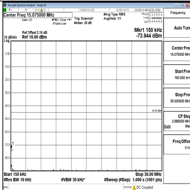
Band41-20MHz-QPSK-39750-1RB#0-0.15~30-PASS
