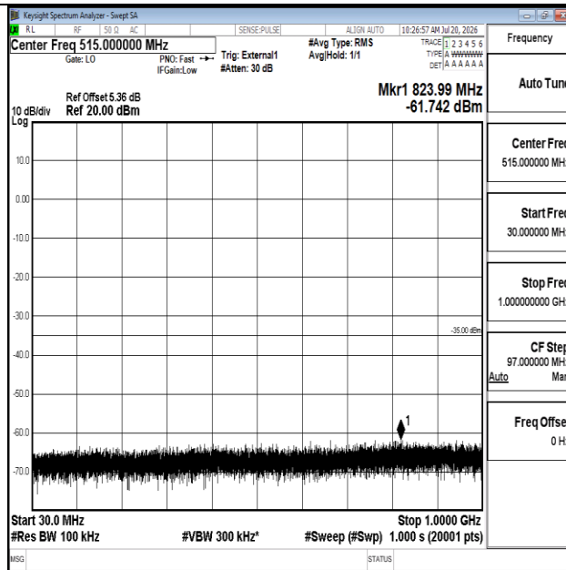
Band41-15MHz-16QAM-41515-1RB#0-30~1000-PASS
