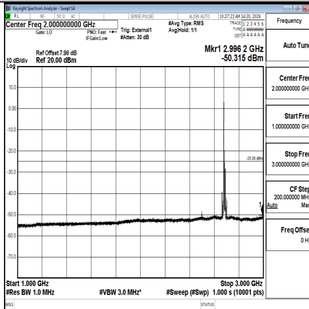
Band41-15MHz-16QAM-41515-1RB#0-1000~3000-PASS
