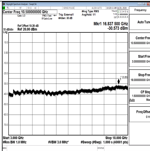
Band41-15MHz-QPSK-40620-1RB#0-3000~18000-PASS
