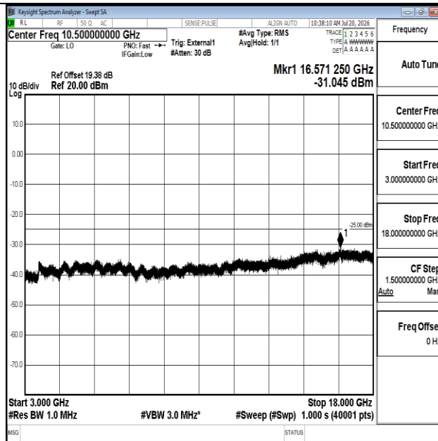
Band41-20MHz-16QAM-40620-1RB#0-3000~18000-PASS
