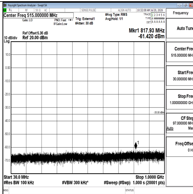
Band41-20MHz-16QAM-39750-1RB#0-30~1000-PASS
