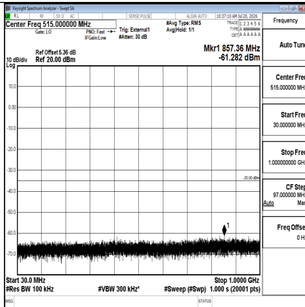
Band41-20MHz-16QAM-40620-1RB#0-30~1000-PASS
