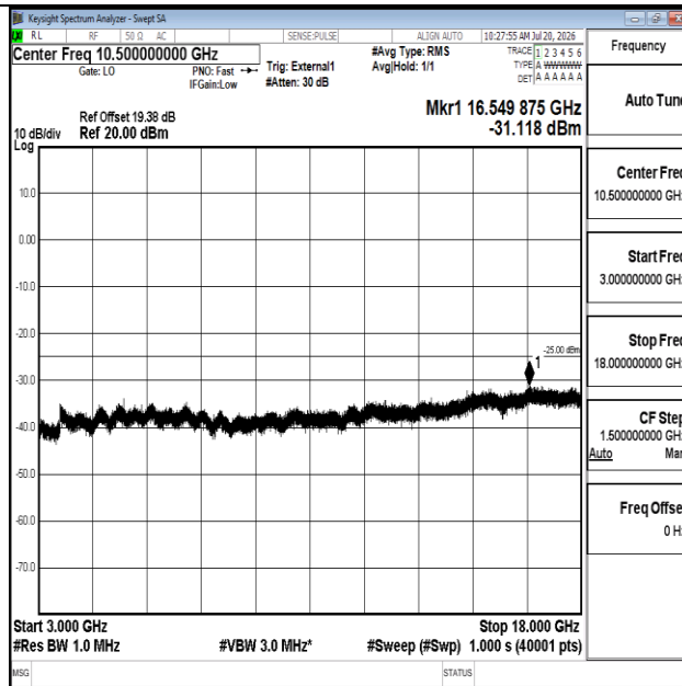
Band41-15MHz-16QAM-41515-1RB#0-3000~18000-PASS
