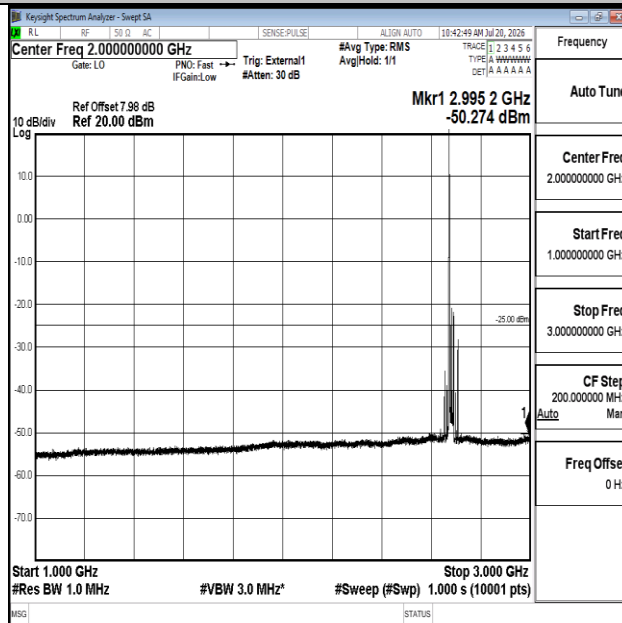
Band41-20MHz-16QAM-41490-1RB#0-1000~3000-PASS
