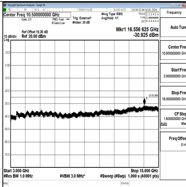
Band41-20MHz-QPSK-39750-1RB#0-3000~18000-PASS
