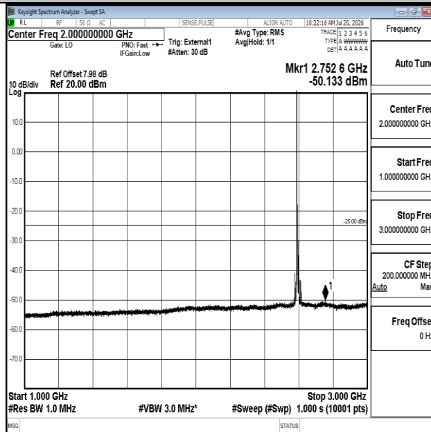
Band41-15MHz-16QAM-40620-1RB#0-1000~3000-PASS
