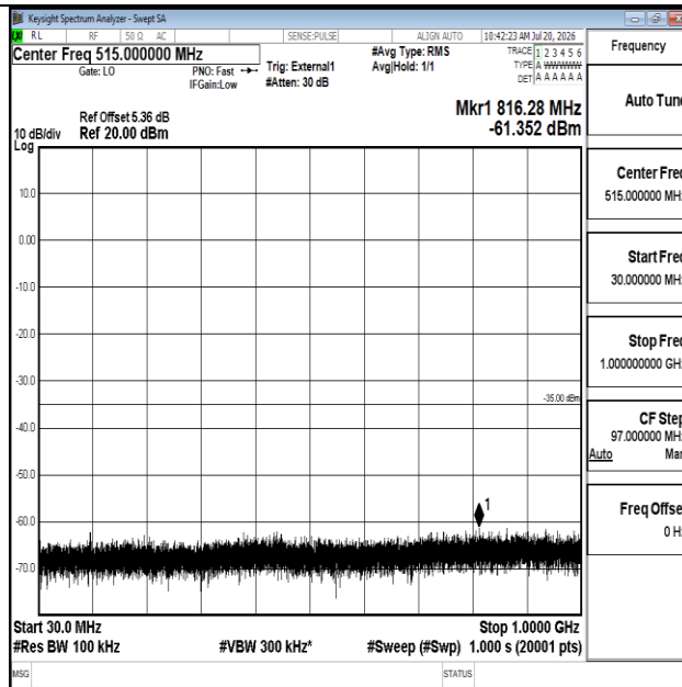
Band41-20MHz-16QAM-41490-1RB#0-30~1000-PASS
