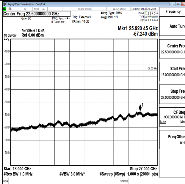
Band41-20MHz-16QAM-40620-1RB#0-18000~27000-PASS
