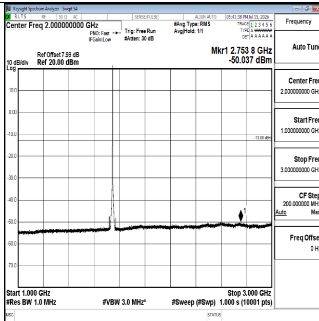
Band66-1.4MHz-16QAM-132322-1RB#0-1000~3000-PASS
