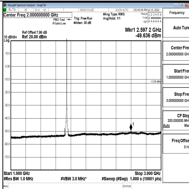
Band66-1.4MHz-QPSK-132322-1RB#0-1000~3000-PASS
