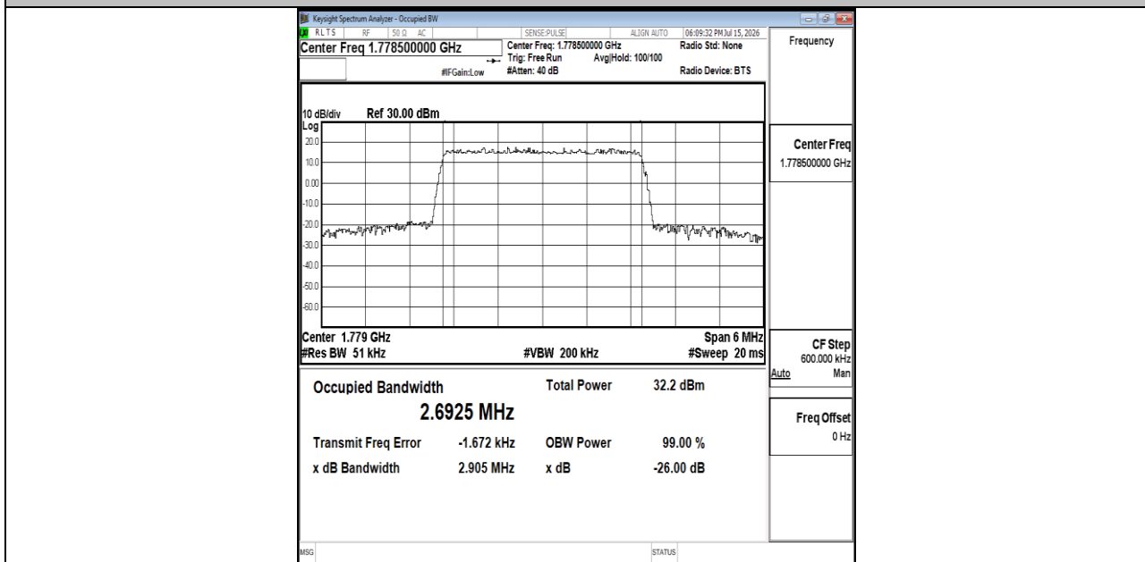
Band66-3MHz-16QAM-132657-15RB#0-PASS
