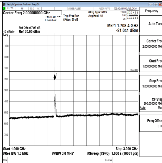
Band66-1.4MHz-16QAM-131979-1RB#0-1000~3000-PASS
