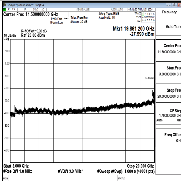
Band66-1.4MHz-16QAM-132322-1RB#0-3000~20000-PASS
