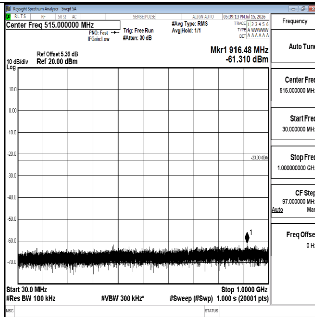
Band66-1.4MHz-QPSK-131979-1RB#0-30~1000-PASS
