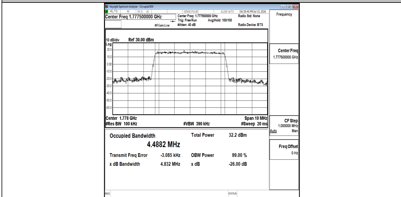
Band66-5MHz-16QAM-132647-25RB#0-PASS
