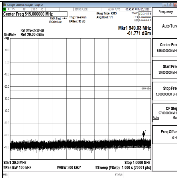
Band66-1.4MHz-QPSK-132322-1RB#0-30~1000-PASS
