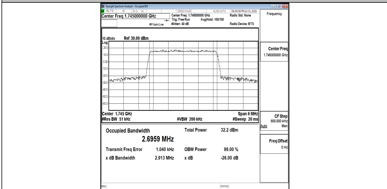
Band66-3MHz-16QAM-132322-15RB#0-PASS
