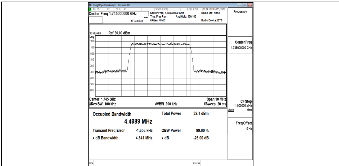
Band66-5MHz-QPSK-132322-25RB#0-PASS
