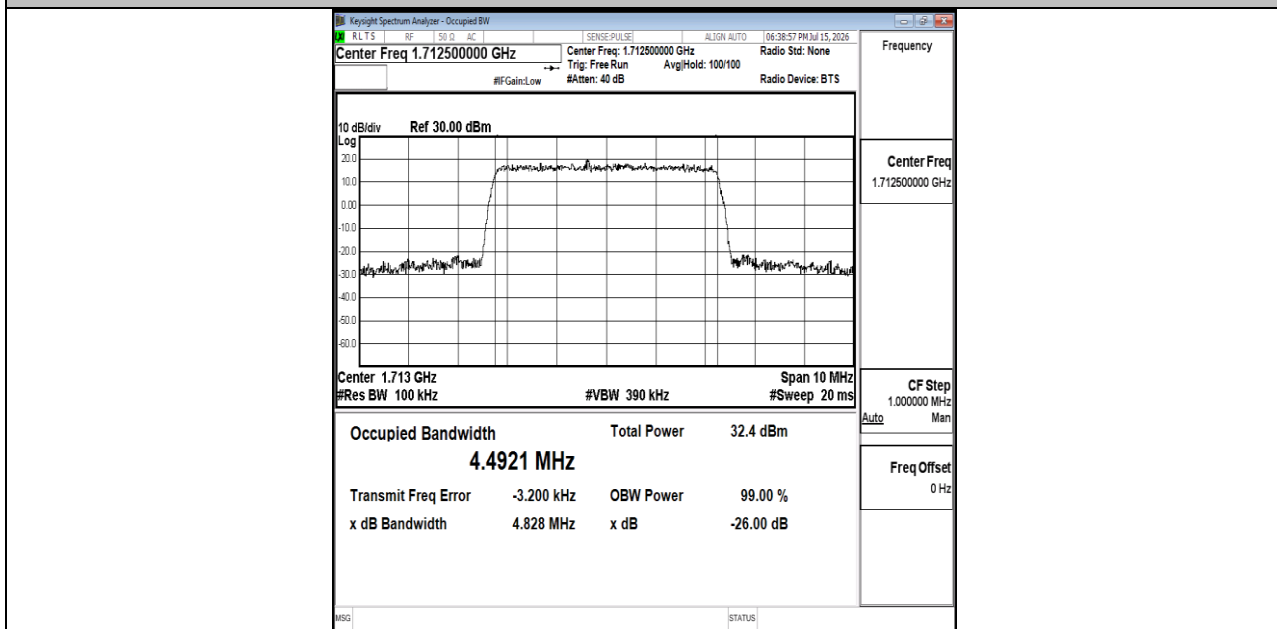
Band66-5MHz-16QAM-131997-25RB#0-PASS
