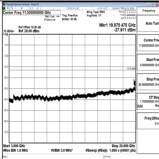
Band66-1.4MHz-16QAM-131979-1RB#0-3000~20000-PASS
