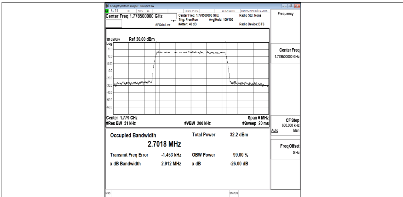
Band66-3MHz-QPSK-132657-15RB#0-PASS
