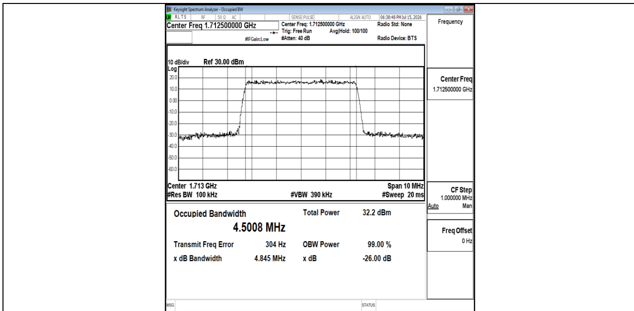
Band66-5MHz-QPSK-131997-25RB#0-PASS
