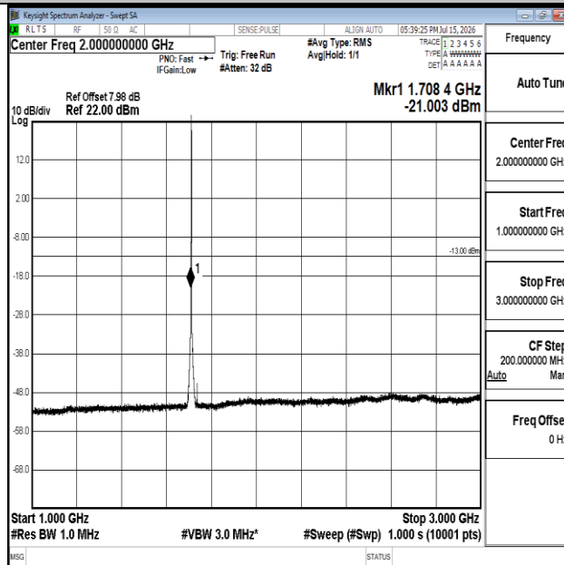
Band66-1.4MHz-QPSK-131979-1RB#0-1000~3000-PASS
