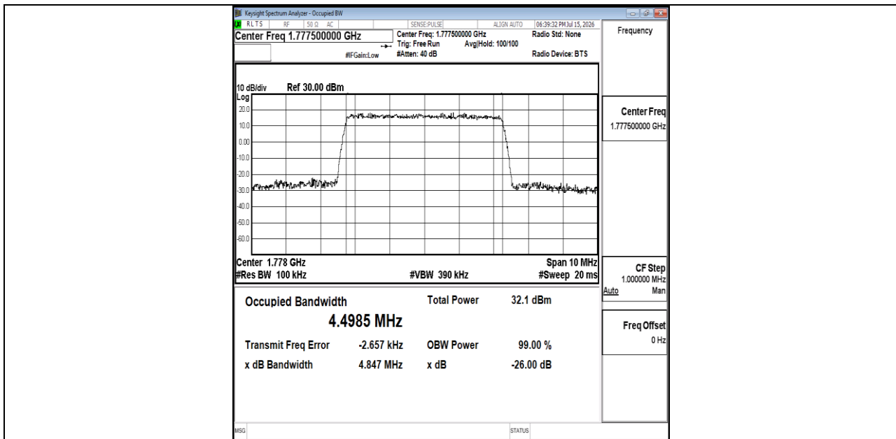
Band66-5MHz-QPSK-132647-25RB#0-PASS
