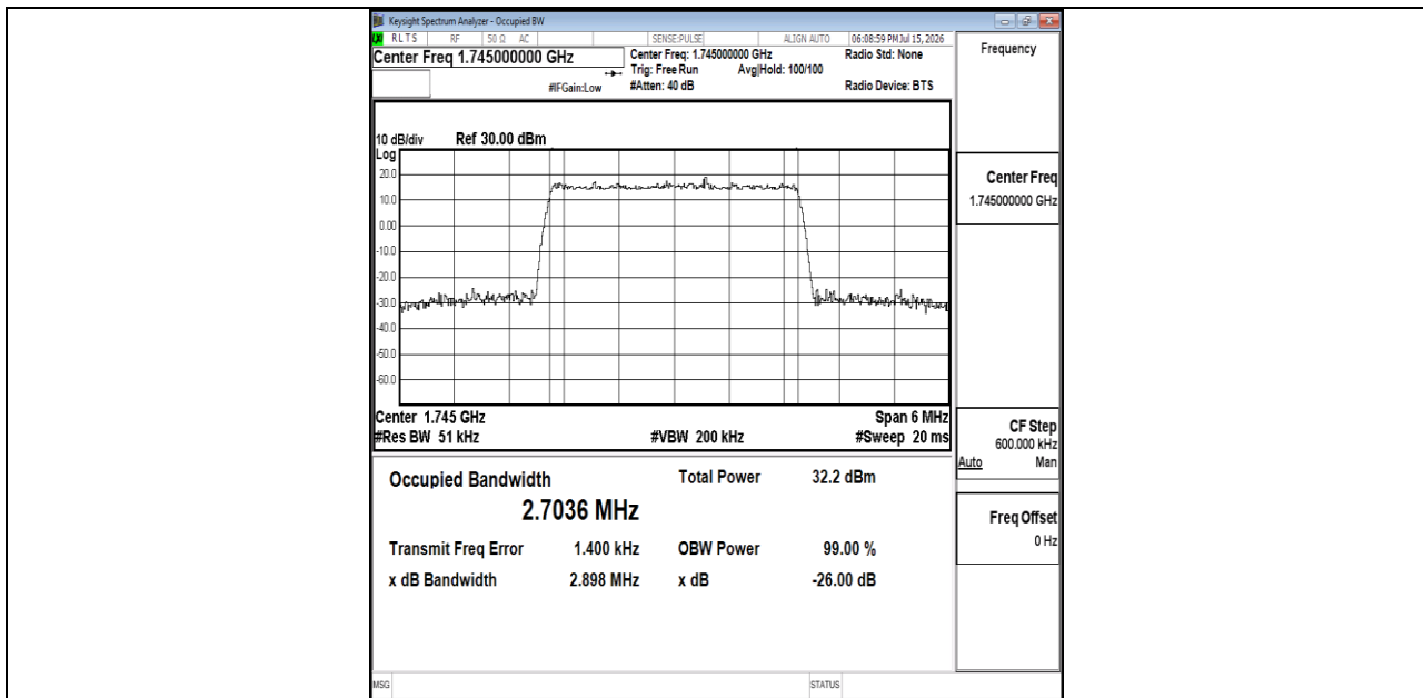
Band66-3MHz-QPSK-132322-15RB#0-PASS
