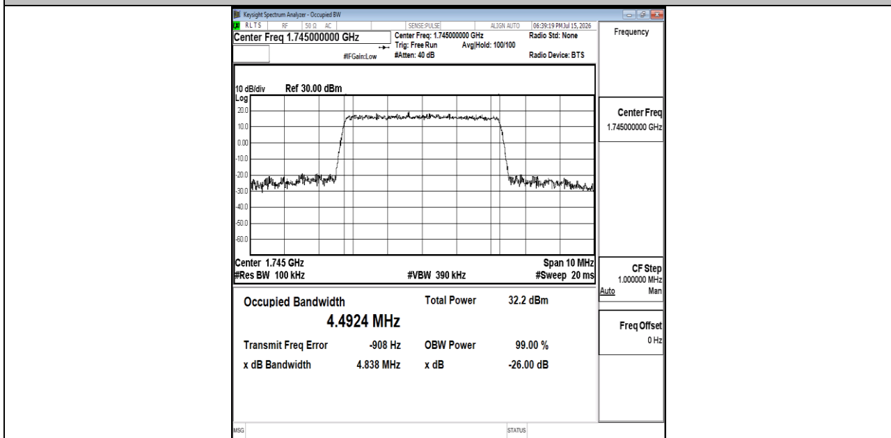
Band66-5MHz-16QAM-132322-25RB#0-PASS
