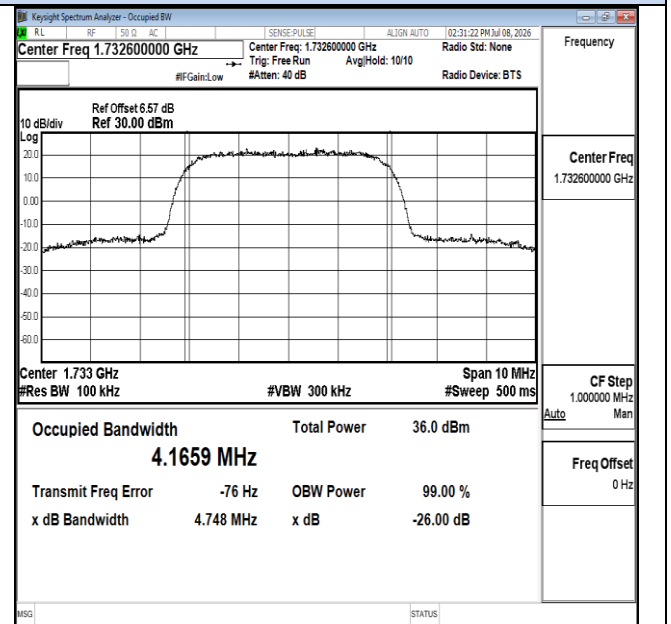
Channel 1413 / 1732.6 MHz
