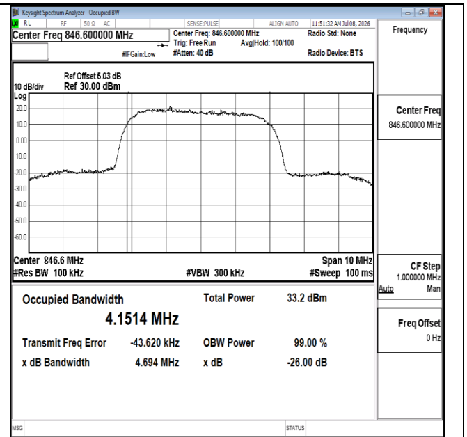
Channel 4233 / 846.6 MHz
