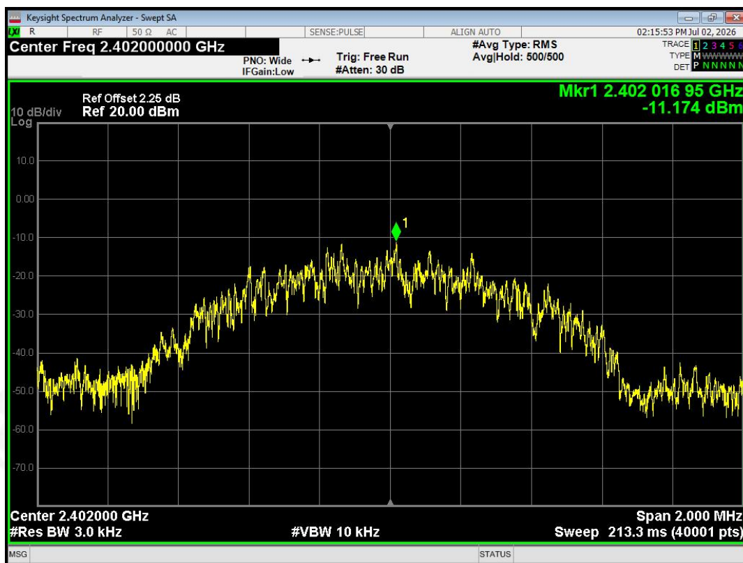
Test Chart GFSK - 2402MHz
