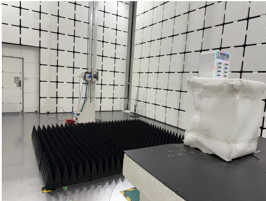
Emissions in Restricted Frequency Bands Emissions in Non-restricted Frequency Bands(1-18 GHz)
