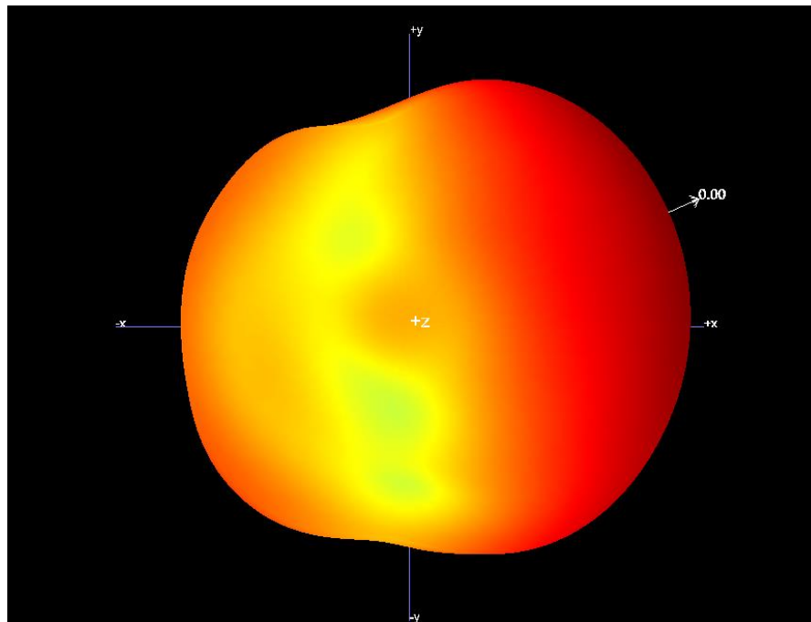
B1.2 3D Pattern for 2450MHz
