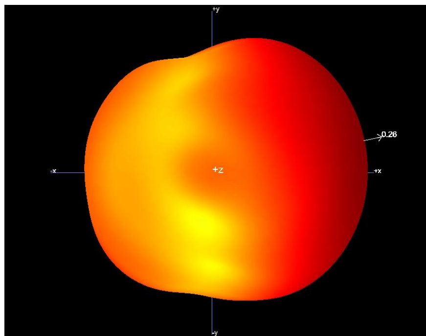
B1.3 3D Pattern for 2500MHz
