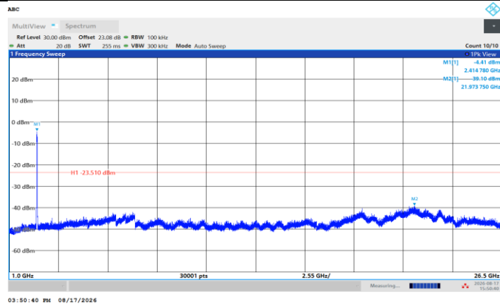
11N40SISO_Ant1_2422_1000~26500
