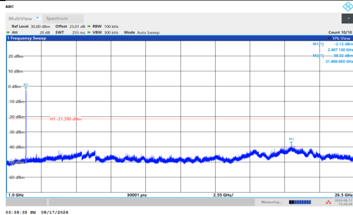
11N20SISO_Ant1_2412_1000~26500
