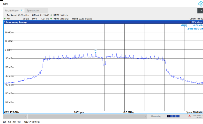
11N40SISO_Ant1_2452_0~Reference
