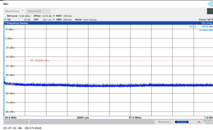
11N40SISO_Ant1_2452_30~1000
