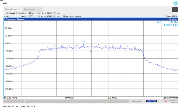
11N20SISO_Ant1_2437_0~Reference
