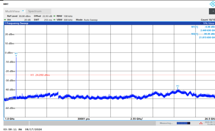
11N40SISO_Ant1_2452_1000~26500
