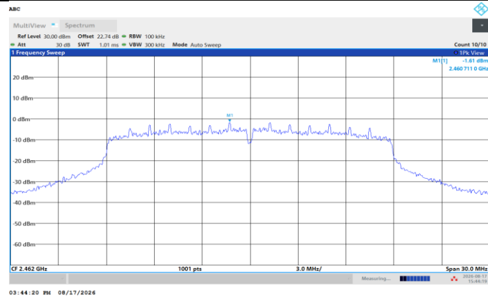
11N20SISO_Ant1_2462_0~Reference
