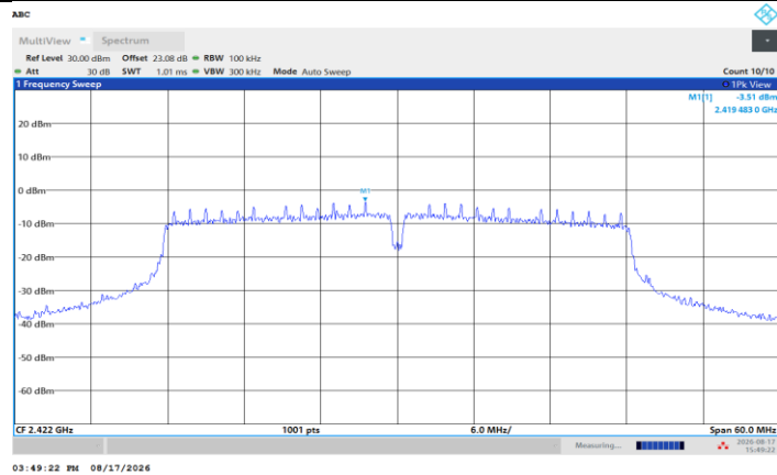
11N40SISO_Ant1_2422_0~Reference
