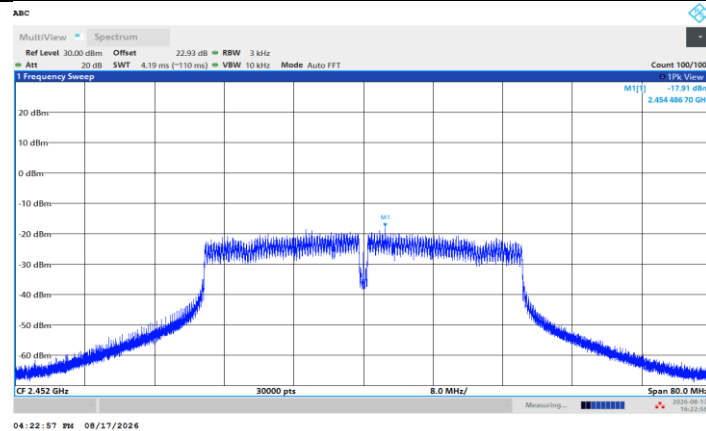
11N40SISO_Ant1_2452
