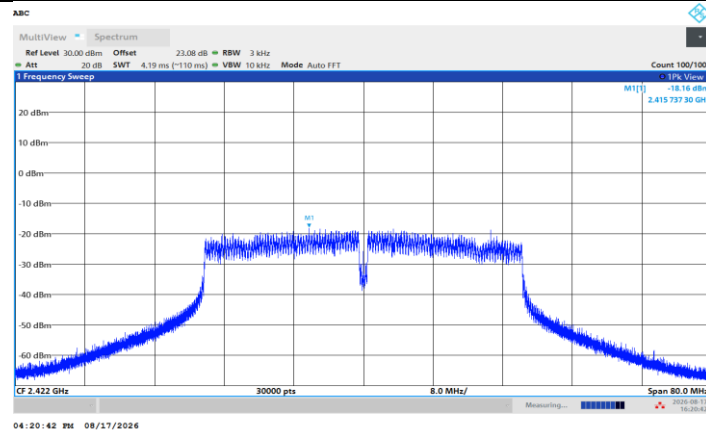
11N40SISO_Ant1_2422
