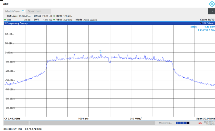
11N20SISO_Ant1_2412_0~Reference
