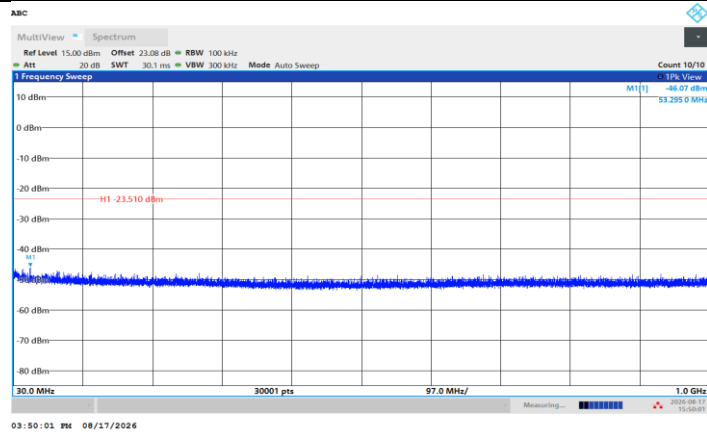
11N40SISO_Ant1_2422_30~1000
