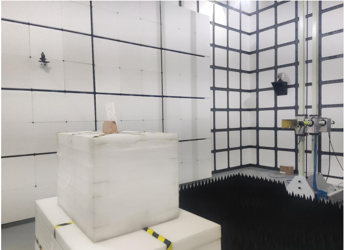
Radiated Emission 18-26.5GHz View
