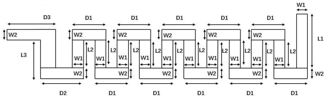
Antenna Dimensions
