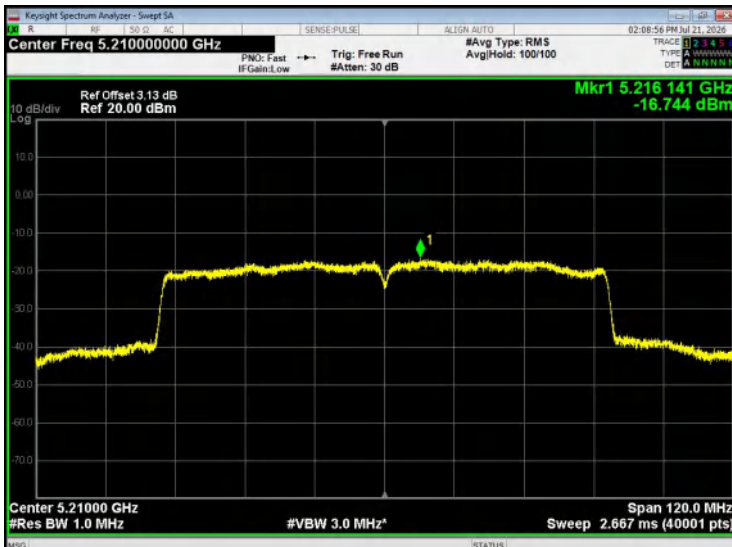
802.11ac80-CH 42
