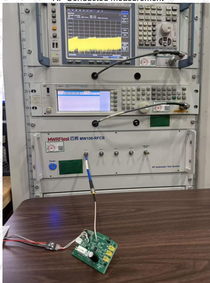
RF Conducted measurement
