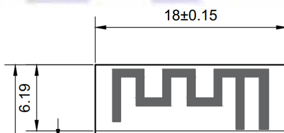
Antenna drawing
