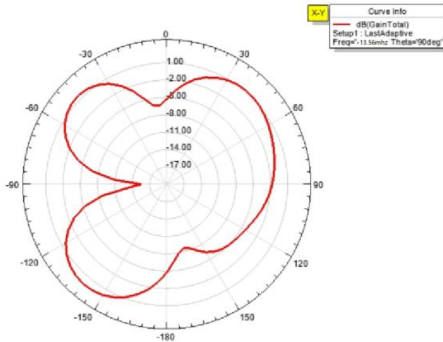
Radiation Pattern 2
