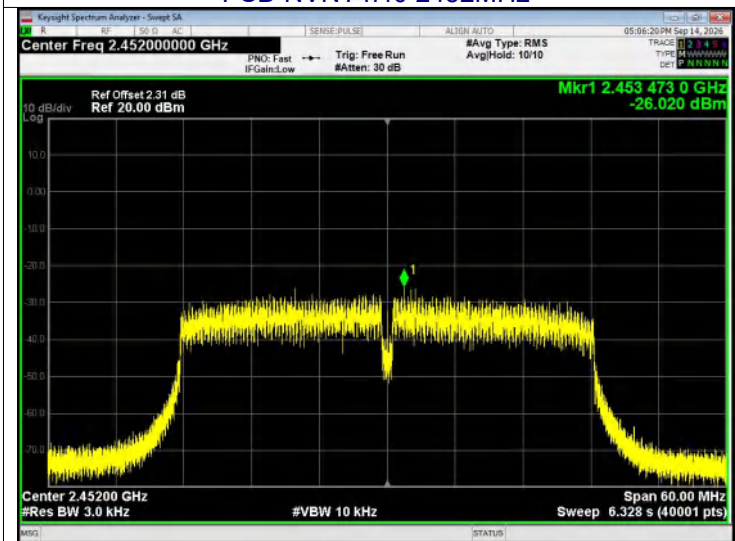
PSD NVNT n40 2452MHz
