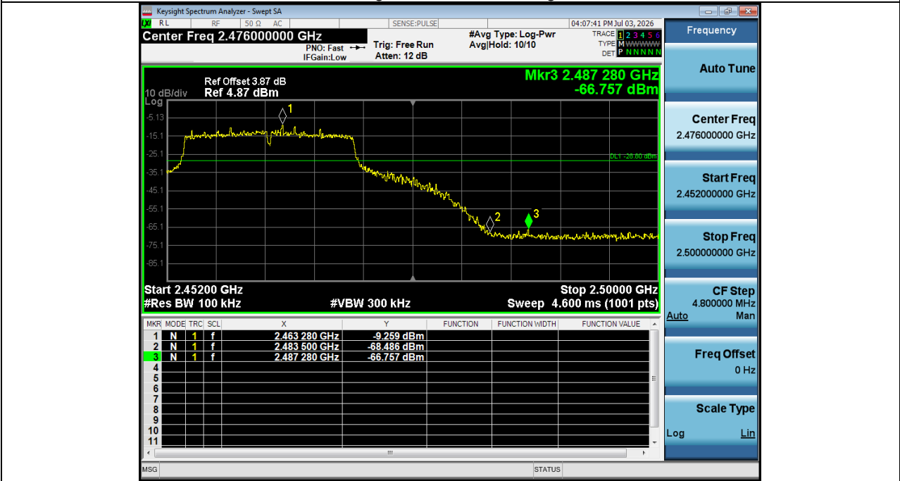
2. Bandedge NVNT_ANT1_802_11g_2462
