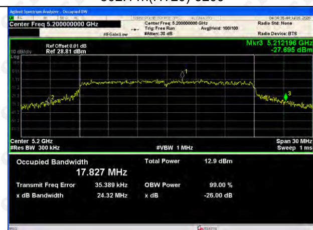
802.11n(HT40)-5190
