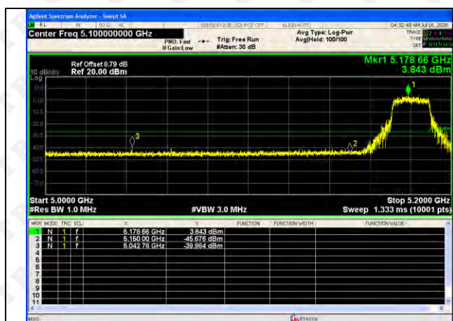
802.11n(HT40)-5190
