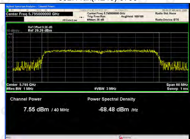
802.11ax(HE40)-5795
