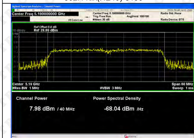
802.11ax(HE40)-5190
