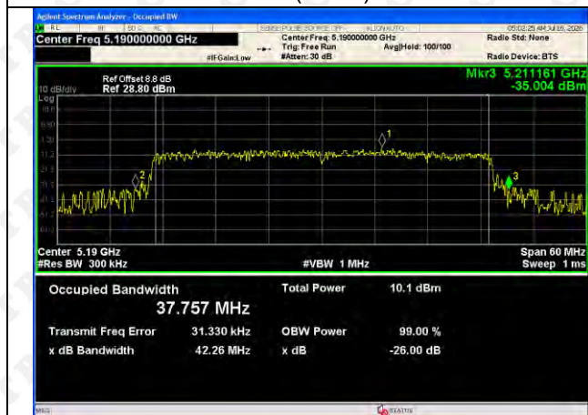
802.11ax(HE40)-5190
