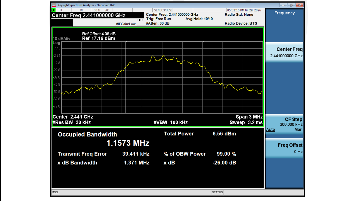
99%_Occupied_Bandwidth_NVNT_ANT1_3-DH1_2441_00
