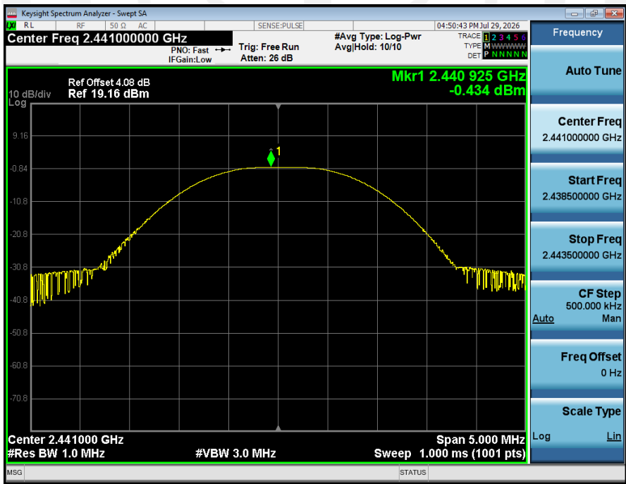
Peak_Output_Power_NVNT_ANT1_1-DH1_2441_00
