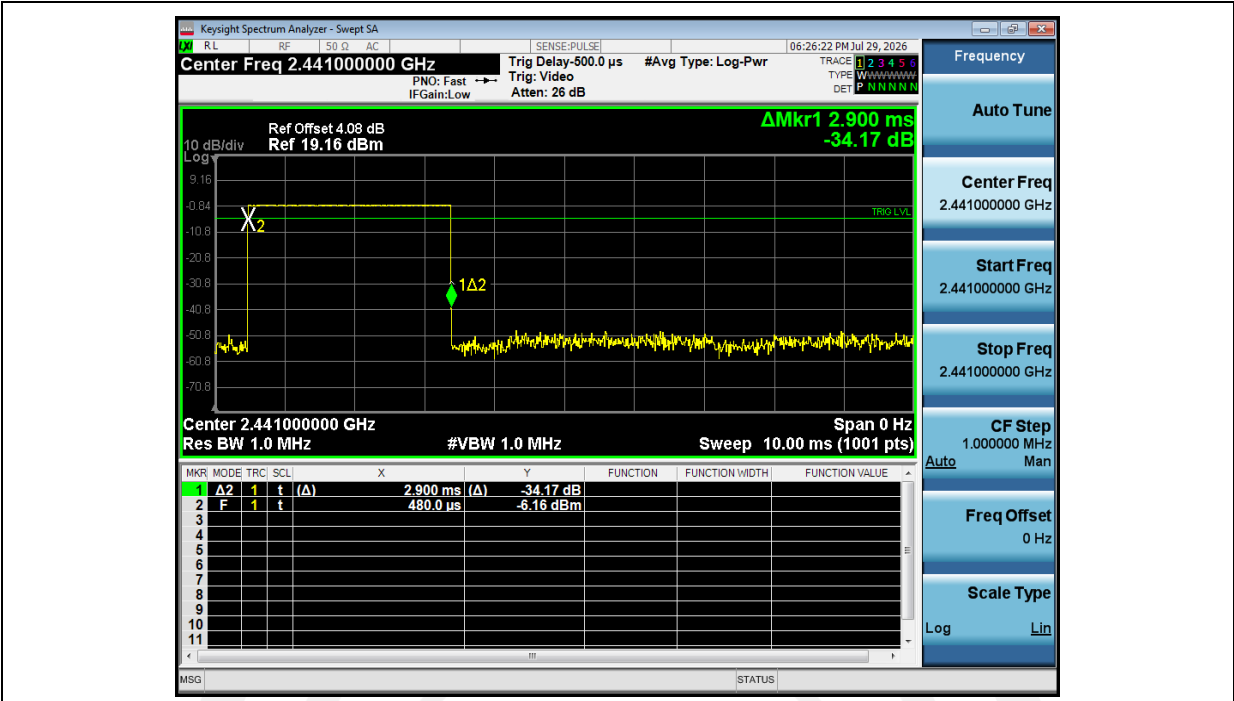
Dwell_Time (Hopping)_NVNT_ANT1_1-DH5_2441_00_Accumulated
