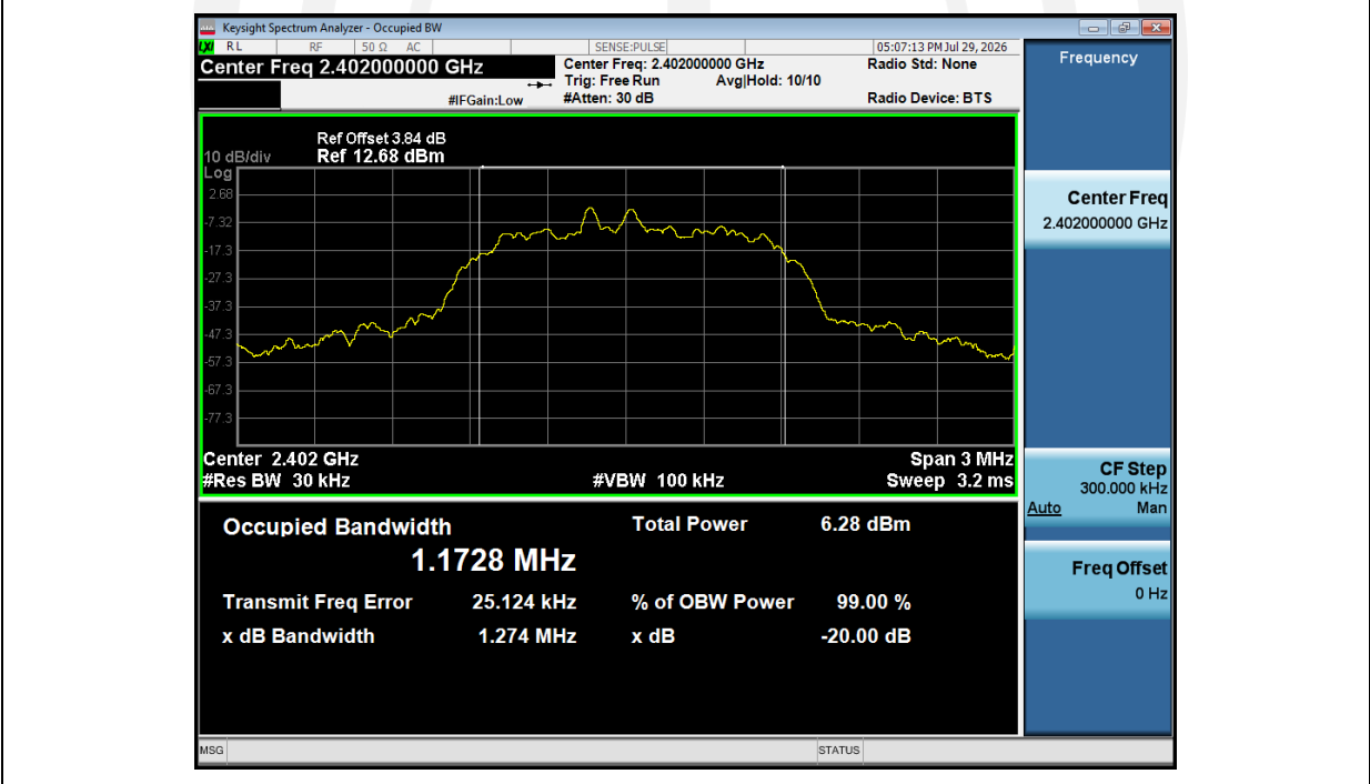
-20dB_Bandwidth_NVNT_ANT1_2-DH1_2402_00
