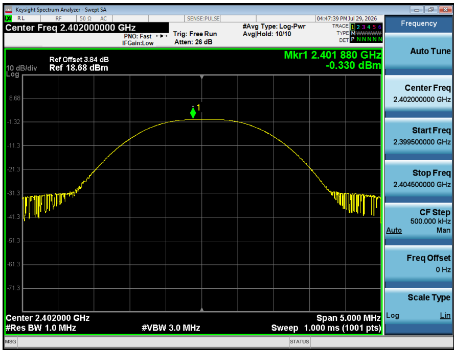
Peak_Output_Power_NVNT_ANT1_1-DH1_2402_00
