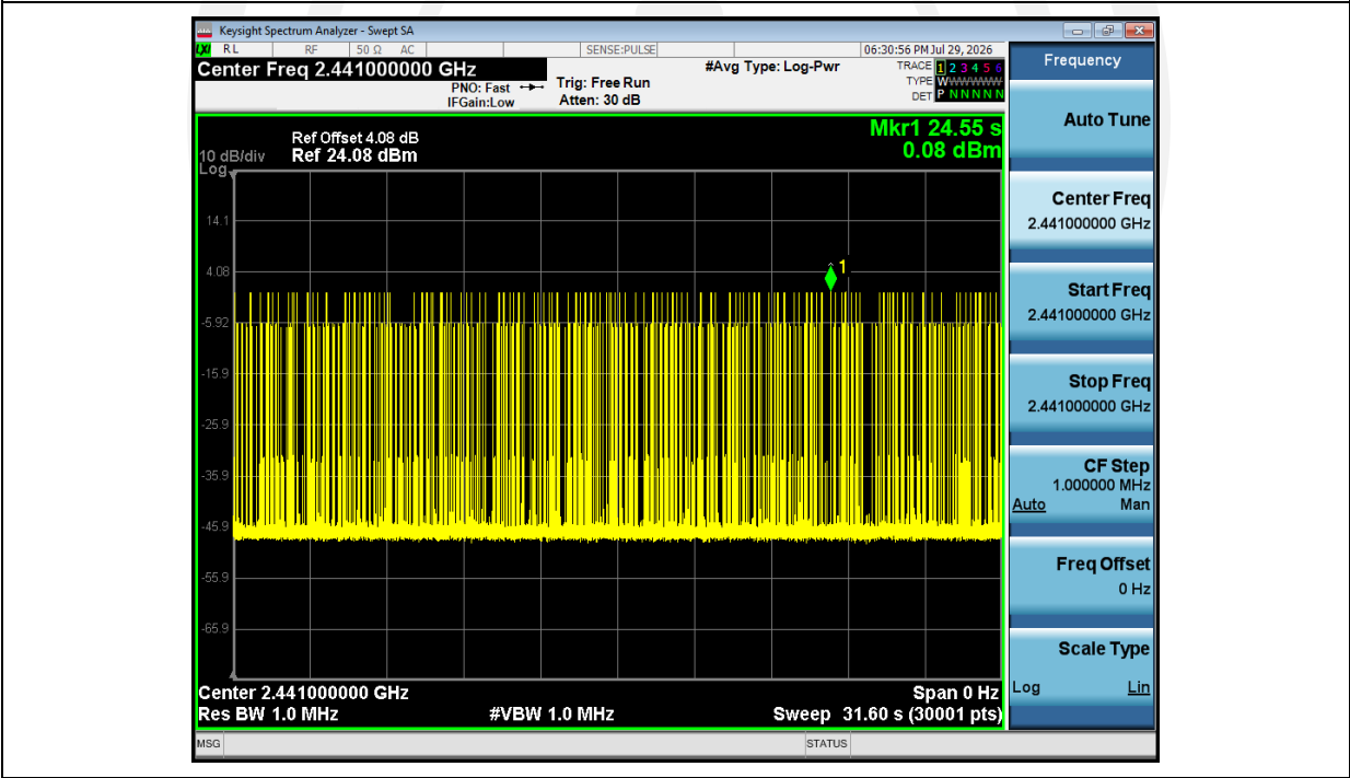
Dwell_Time (Hopping)_NVNT_ANT1_3-DH3_2441_00_Accumulated
