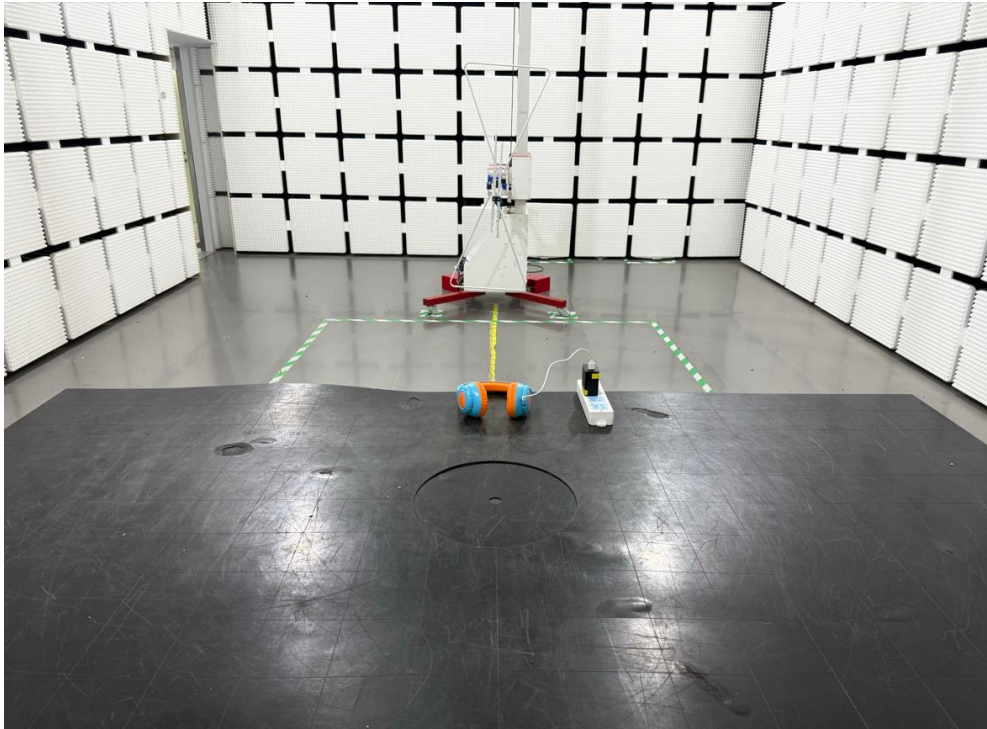
Spurious Radiation Emissions Test (<1G)
