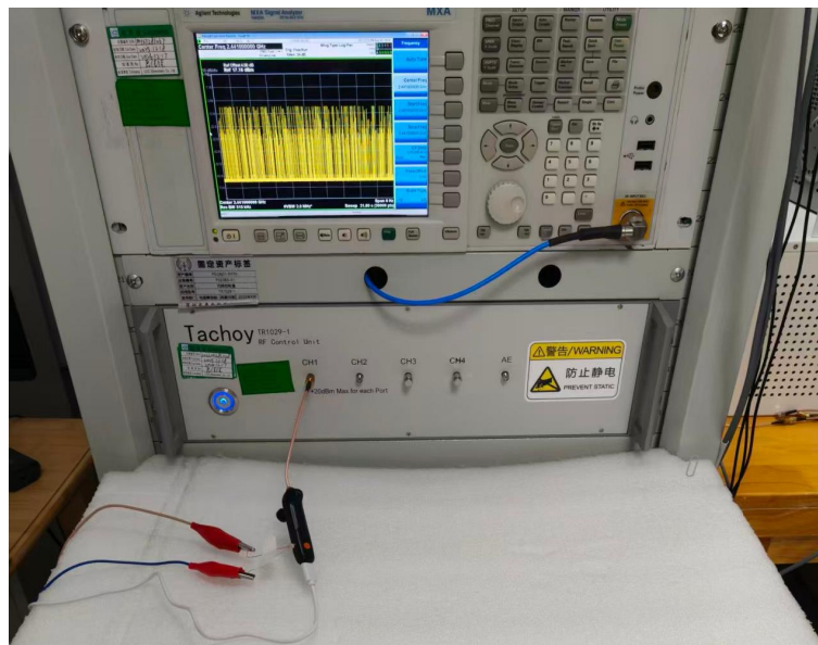
RF Conducted Test Photo
