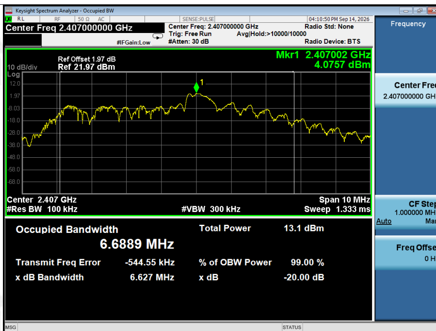
-20dB Bandwidth-GFSK 2407MHz
