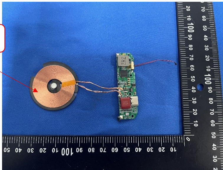
Loop Antenna
