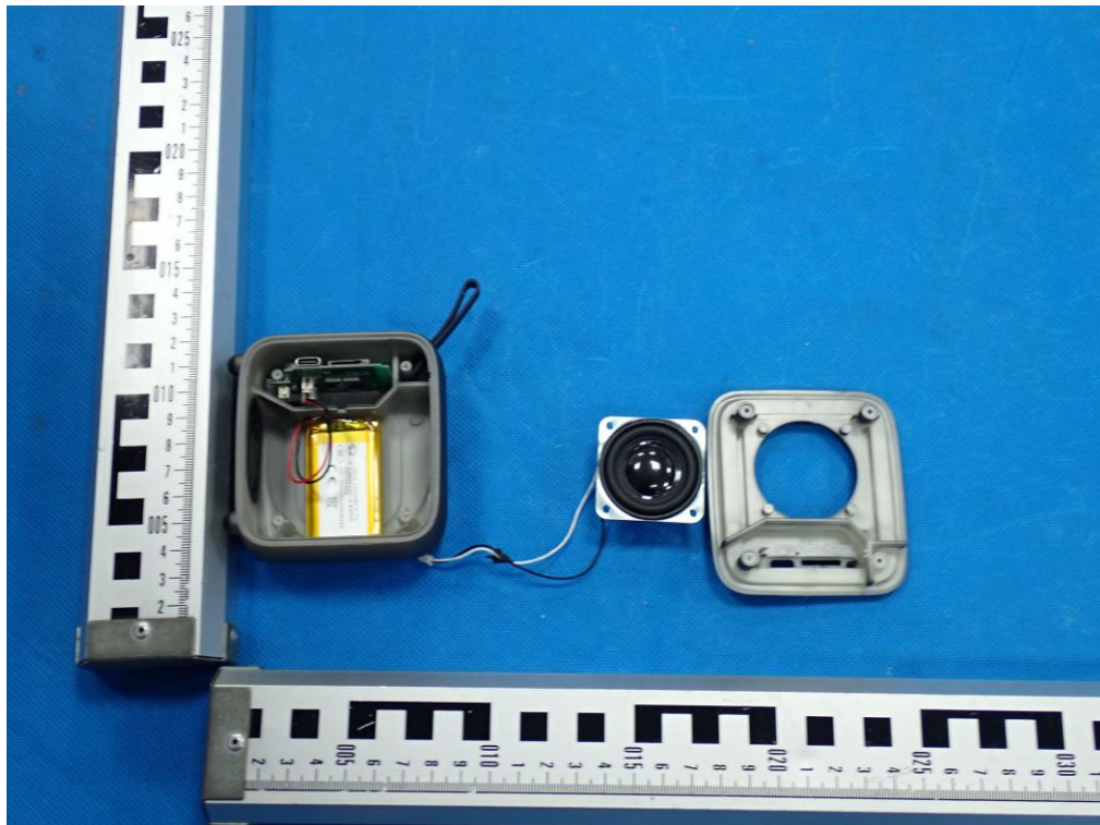
Internal Photo 3
