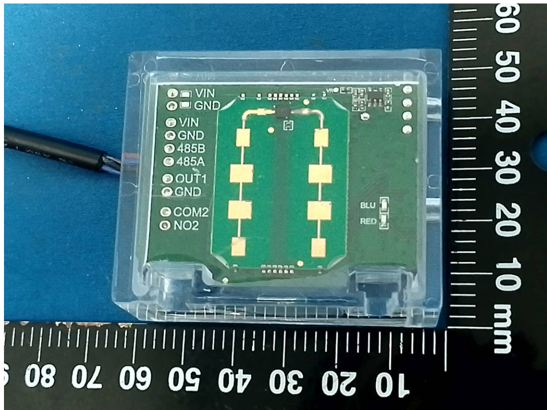
Radar Antenna+Chip
