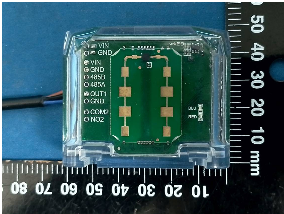
Radar Antenna+Chip
