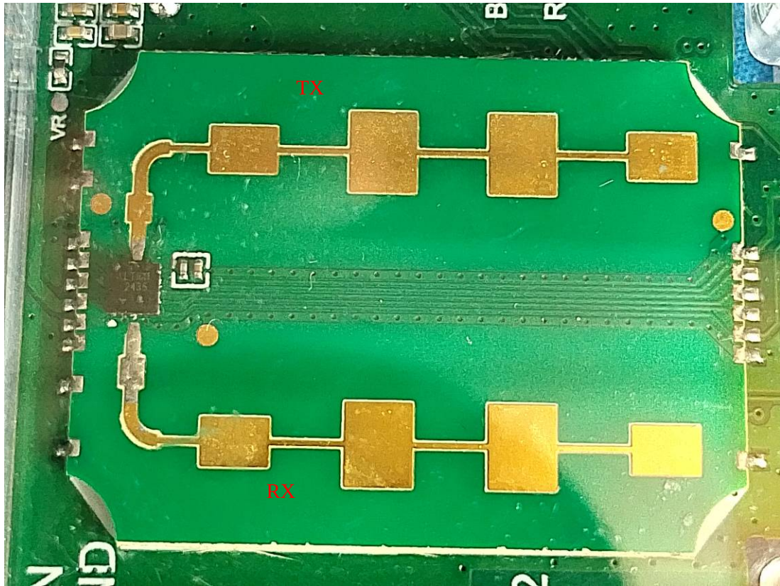
Radar Antenna
