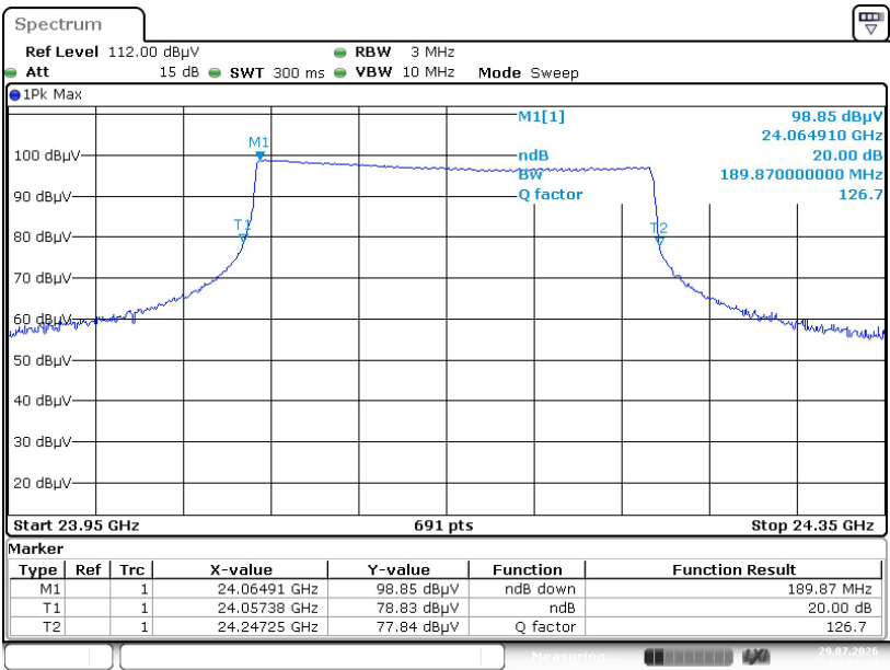
20 dB Bandwidth
