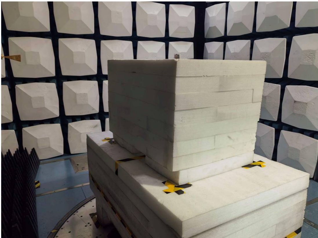
Radiated Emission Above 1GHz View 40-60G
