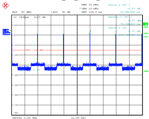
BLE_1M_Middle_Channel
